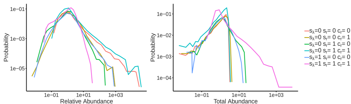
Fig. S19. Numerical simulations of mathematical model #4. The panels show the same distributions as in Fig. S16. The right plot shows the distribution of the total biomass across particles. In all the simulations we set \lambda^d = 1 , \bar{\lambda} = 1 , and \bar{r} = 1 (where the total time of the experiment was also set to be equal to 1). Different values of s_r , s_\lambda and c_r correspond to different colors.
