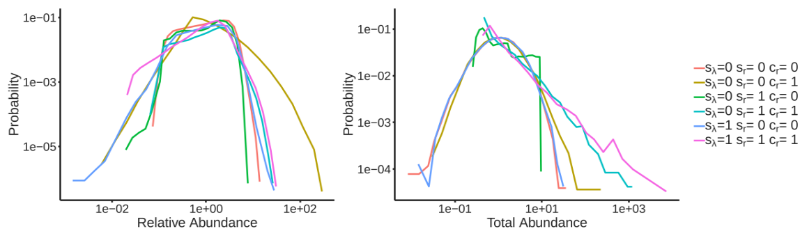
Fig. S18. Numerical simulations of mathematical model #3. Numerical simulations of model #3.
