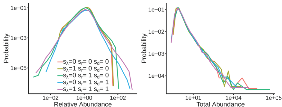
Fig. S17. Numerical simulations of mathematical model #2. The left panel shows the distribution of rescaled relative abundances averaged over MAGs. For each MAG the logarithm of the relative abundances across particles was rescaled by mean and variance, so that it had mean zero and unit variance. Lines represent averages over MAGs. Colors refer to a particular parameterization. The right plot shows the distribution of the total biomass across particles. In all the simulations we set \bar{\lambda} = 1 and \bar{r} = 1 (where the total time of the experiment was also set to be equal to 1). Different values of s_r and s_\lambda correspond to different colors.
