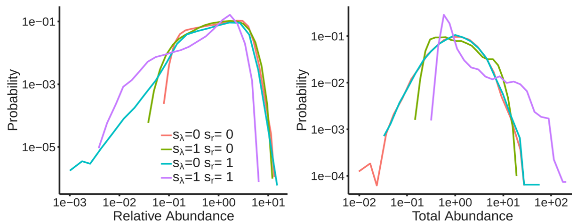
Fig. S16. Numerical simulations of mathematical model #1. The left panel shows the distribution of rescaled relative abundances averaged over MAGs. For each MAG the logarithm of the relative abundances across particles was rescaled by mean and variance, so that it had mean zero and unit variance. Lines represent averages over MAGs. Colors refer to a particular parameterization. The right plot shows the distribution of the total biomass across particles. In all the simulations we set \bar{\lambda} = 1 and \bar{r} = 1 (where the total time of the experiment was also set to be equal to 1). Different values of s_r and s_\lambda correspond to different colors.
