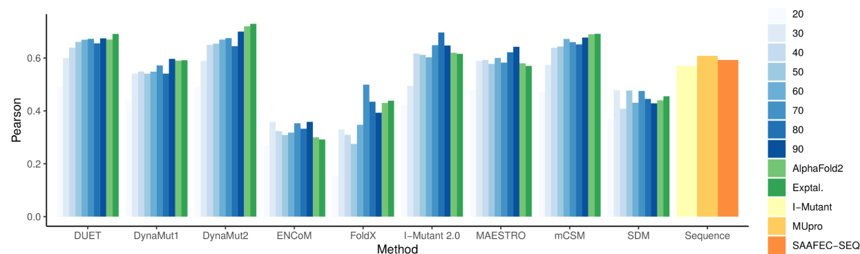
Fig S7 — Comparative performance of methods predicting stability changes upon mutation using AlphaFold2 and MODELLER models. The performance of nine well established structure-based methods is contrasted on a mutation benchmark data set when presented to either AlphaFold2 models (light green bars) or homology models (blue bars) derived from templates of varying identity levels. Baseline performance using experimental structures (dark green bar) and of three sequence-based tools (yellow and orange bars) are also shown.
