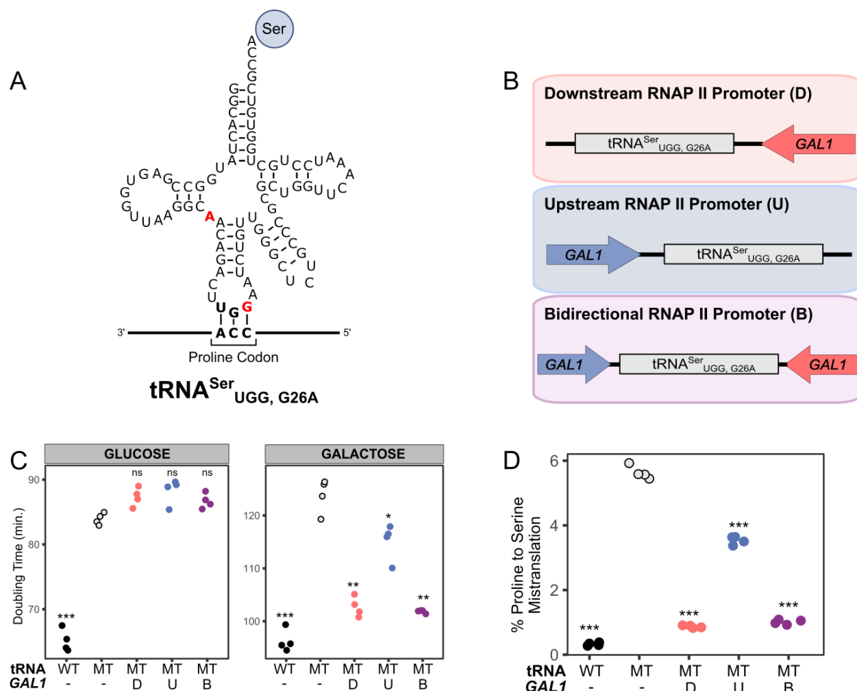
Figure 1. Transcription from a flanking RNAP II promoter decreases mistranslation derived from a mistranslating tRNA gene. (A) The structure of tRNA Ser UGG, G26A . Bases colored red were mutated to allow for non-lethal levels of serine mis-incorporation at proline codons. (B) The GAL1 promoter was cloned either 300 bp downstream (D), 300 bp upstream (U) or both up and downstream (B) of the gene encoding tRNA Ser UGG, G26A . The sequence directly flanking the tRNA encoding sequence is from SUP17 . (C) Wild type yeast strain BY4742 containing either wild type tRNA Ser (WT), mistranslating tRNA Ser UGG, G26A (MT) or the mistranslating tRNA Ser UGG, G26A with GAL1 promoters flanking were grown to saturation overnight in medium lacking uracil. Strains were diluted to an OD 600 of 0.1 in the same media containing either galactose or glucose as the carbon source and grown for 24 hours at 30°C with agitation. OD 600 was measured every 15 minutes and doubling time in minutes calculated from the growth curves. (D) Mass spectrometry analysis of the cellular proteome was performed on the strains described in (C) grown in galactose to determine the frequency of proline to serine substitution. In each panel, points represent biological replicates and stars indicate significant differences compared to the unregulated tRNA Ser UGG, G26A mistranslating strain (Welch's T-test; * p < 0.01 , ** p < 0.001 , *** p < 0.0001 ; ns – not statistically different).
