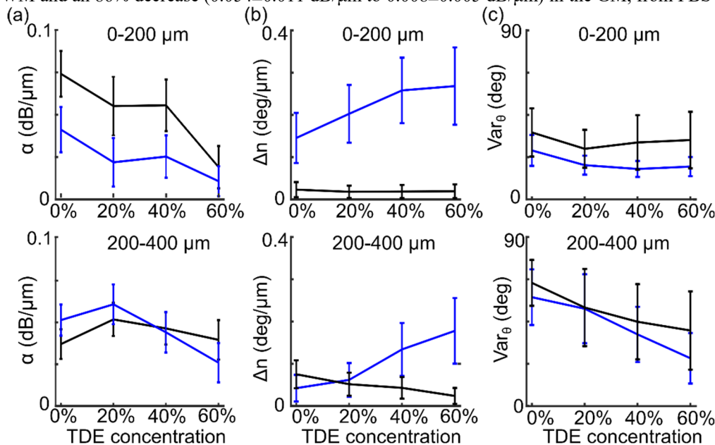
Fig. 4. PS-OCT measurements with respect to TDE concentration. Attenuation coefficient \alpha (a), apparent birefringence \Delta n (b) and s.t.d. of axis orientation \text{Var}_\theta (c) using 0-200 \mu\text{m} (top panel) and 200-400 \mu\text{m} (bottom panel) interval at 0%, 20%, 40% and 60% TDE concentration. The error bars indicate s.t.d. of A-lines, and the blue and black curves indicate WM and GM, respectively.
