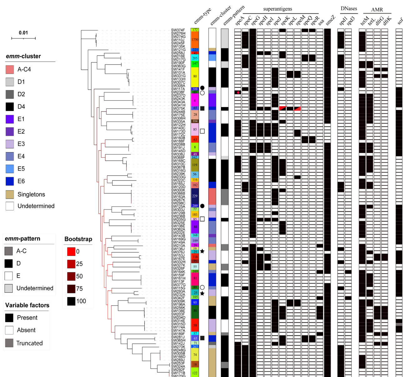
Figure 1: Phylogenetic analysis of 107 genomes from LIC isolates. A maximum likelihood phylogeny was constructed from the core-gene alignment (1,242,112bp) using RAxML (22) with 100 bootstraps. Isolates clustered by emm -type except those indicated, whereby two lineages were represented by a single emm genotype: star; emm 25, filled square; emm 65, open square; emm 85, open circle; emm 89, filled circle; emm 209). Also shown is the presence (black)/absence (white) of the superantigen genes ( speA , speC , speG , speH-M , speQ , speR , ssa and smeZ ) and DNase genes spd1 and spd3 ; four other DNase genes ( sda1 , sda2 , sdn , and
