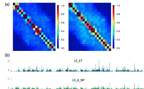
Figure S9. (a) Heatmaps of merged L4 subtype1 (left) and subtype2 (right) on chr11:105,000,000-125,000,000. (b) The mean RNAseq on chr11:105,000,000-125,000,000. The RNAseq plot is available in https://human-mtg-rna-hub.s3-us-west-2.amazonaws.com/HumanMTGRNAHub.html [29].
