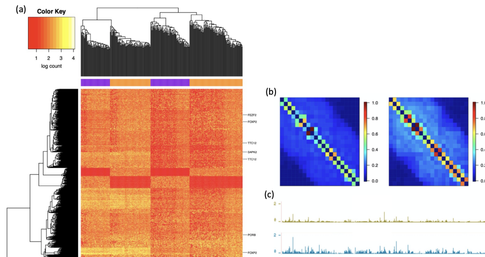
Figure 4. Correspondence between differential 3D structures and differential gene expressions among further subtypes. (a) Heatmap of 500 positions in the 2D interaction matrix with the largest variation among the cells (each row is a position and each column is a cell), with a 2-way clustering outcome placing the L4 cells into the two purple groups and the L5 cells into the two orange groups, and genes showing differential expression [29] indicated on the right edge of the heatmap; (b) Mega 2D matrices of normalized and scaled interaction intensities displayed as heatmaps, with the left for L5T1 and right for L5T2; (c) Mean gene expression for two L5 subtypes described in the literature [29].
