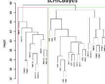
schHiCBayes
