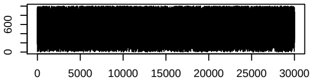
traceplot of a in (40,42)
