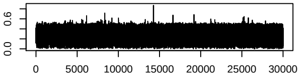
traceplot of \alpha in (40,42)
