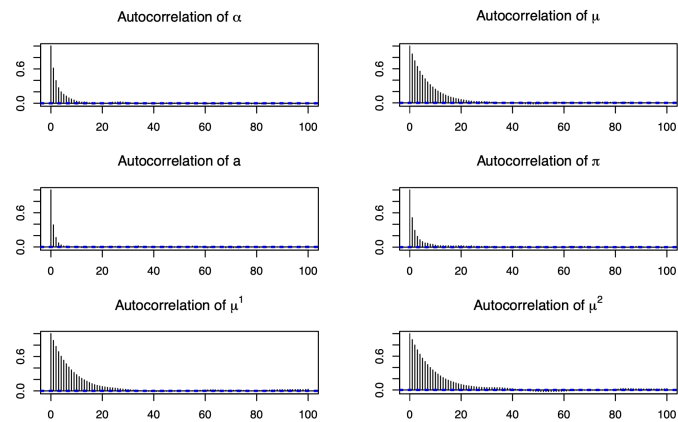
Figure S13. Autocorrelation plots for 6 parameters at position (i, j) = (40, 42) for the simulated dataset with 10 T1 cells at 7K sequencing depth: \mu is the overall expectation for all single cells, and \mu^1 and \mu^2 are the realizations in the first and second single cell, respectively.
