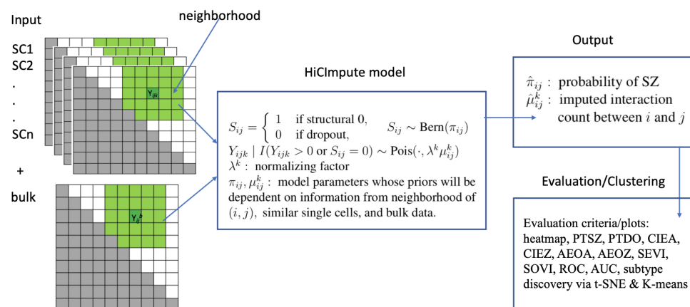
Figure 1. Schematic of the HiCImpute algorithm. Each green region on the left denotes the neighborhood. The indicator variable S_{ij} denotes whether an observed zero at the (i, j) position is a structural zero or not. The \lambda^k is related to the sequencing depth of single cell k and acts as a normalizing factor. Finally, the intensity parameter \mu_{ij}^k is assumed to follow a common distribution across all similar single cells; shrinkage estimation with information from neighborhoods and bulk data will be obtained, which provides accommodations for potential overdispersion. PTSZ (proportion of true structural zeros correctly identified), PTDO (proportion of true dropouts correctly identified), AEOA (absolute error of all observed), AEOZ (absolute error of observed zeros), CIEA (correlation between imputed and expected for all observed), CIEZ (correlation between imputed and expected for observed zeros), SEVI (scatterplot of expected versus imputed), and SOVI (scatterplot of observed versus imputed), ROC (receiver operational characteristics), AUC (area under the curve).
