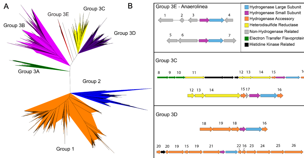
Figure 6. (A) Phylogeny of NiFe hydrogenase large subunit proteins from groups 1, 2, and 3, containing sequences from the Chloroflexi supergroup alongside references, and showing the relative placement of the newly proposed group 3E. (B) Genomic context diagrams for groups 3E, 3C, and 3D showing the diversity in function between the NiFe hydrogenase subtypes in the Chloroflexi supergroup. Group 3E was not found to regularly co-occur with accessory proteins, whereas group 3C often occurred proximal to heterodisulfide reductase genes (hdrA2B2C2), and group 3D often co-occurred with numerous accessory and electron transfer subunit genes. Numbered genes are annotated as follows:
