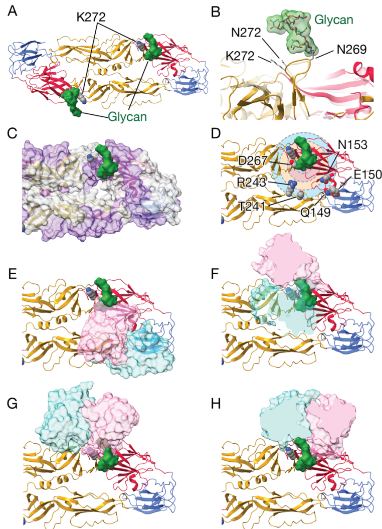
Figure S5. Identification of B-cell epitopes and E:nAb complexes from other flaviviruses in proximity to the kl loop in the YFV E protein. (A) Dimer structure of YFV-17D E (PDB: 6IW4; Domain I: red, Domain II: yellow, Domain III: blue) with the modeled kl loop (residues 267 to 272), including K272 and the glycan moiety (in green) (Lu et al., 2019). The glycan structure corresponds to the experimentally determined glycan moiety observed in the envelope protein of Dengue 2 (glycosylated N153; PDB: 4UTC) (Rouvinski et al., 2015). (B) Close-up view of the modeled kl loop, the glycan moiety on N269, and K272. Faded structure corresponds to X-ray monomeric structure of 17D E (with Asn at position 272, PDB: 6EPK). (C–D) Predicted and known B-cell epitopes in proximity to the kl loop. Surface-shaded representation of the YFV-17D E dimer with the modeled kl loop (residues 267–272, with K at position 272) and the glycan moiety (in green) is shown. (E) Purple colored surface patches correspond to predicted B-cell epitopes. (F) Concentric circles (with radius = 5Å, 10Å, 15Å and 20Å) are centered at Ca of glycosylated Asn 269. Residues represented as spheres have been described to be part of B-cell epitopes
