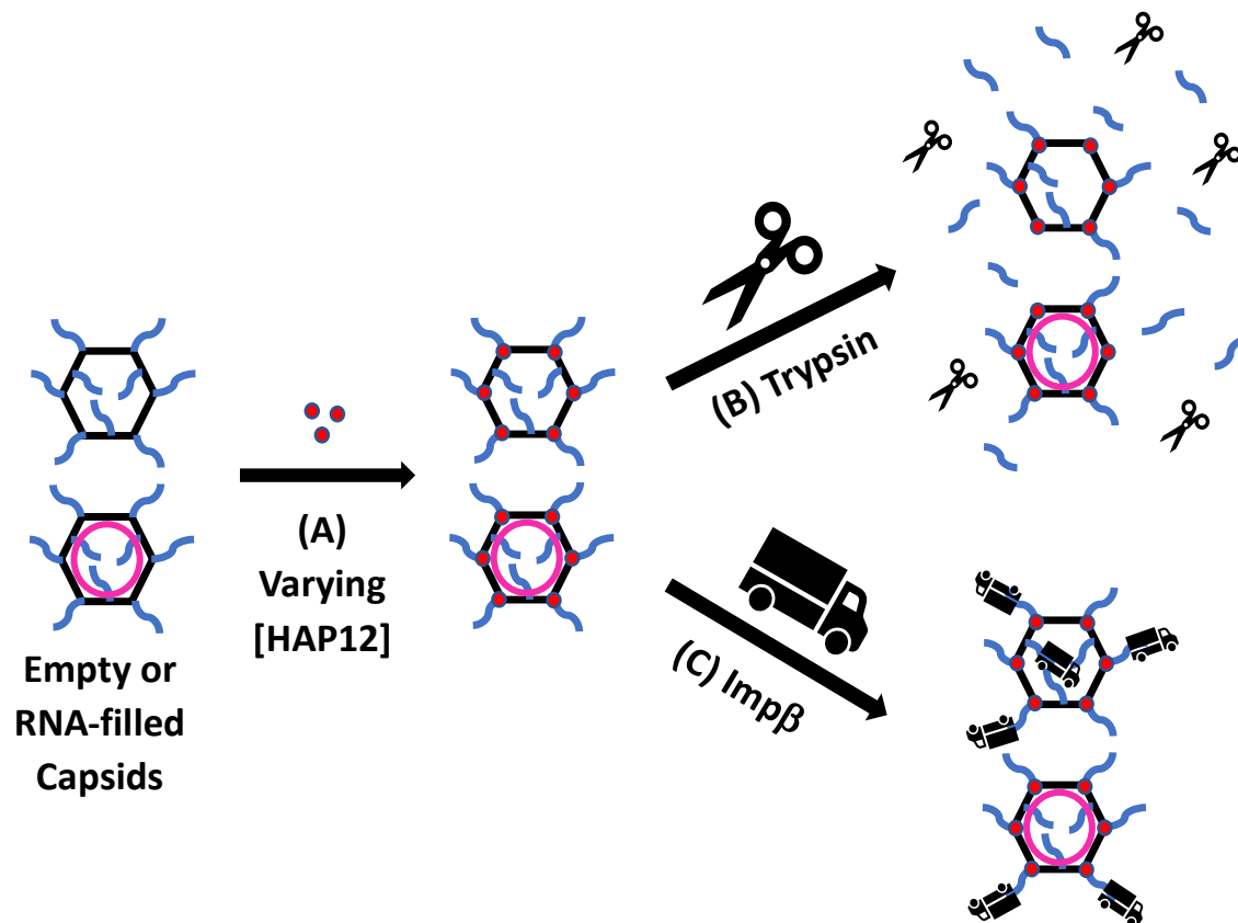
Figure 1. Capsid proteolysis and Impβ binding experimental schematic. (A) Empty and RNA-filled capsids were initially treated with varying concentrations of the CpAM HAP12 and then interrogated by proteolysis or Impβ-binding. Trypsin is represented by scissors, and Impβ is represented by trucks. HAP12-treatment was characterized in terms of “saturation”: at saturating HAP12 concentrations, there is one active HAP12 molecule for every HAP pocket. (B) HAP12-treated empty, pgRNA-filled, and E. coli RNA-filled capsids were digested with trypsin and reactions were quenched before proteolyzed products were resolved using SDS-PAGE and LC-MS. (C). HAP12-treated empty and E. coli RNA-filled capsids were mixed with Impβ and dialyzed into a low NaCl concentration buffer to allow binding. Impβ-bound capsids were analyzed using SEC, SDS-PAGE, TEM, and CDMS.
