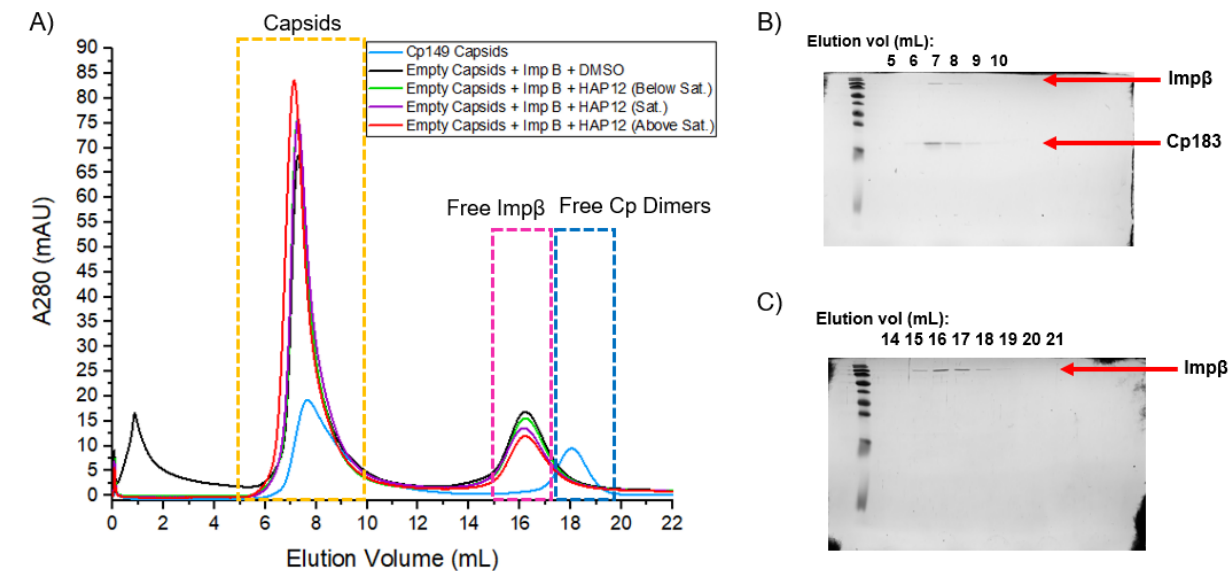
Supplementary Figure 1. At super-sat. [HAP12], the capsid peak shifted to the left, which indicated elution of complexes larger than capsids. To resolve Impβ-bound capsids, 200 μL of each sample were injected onto a Superose 6 column. SEC fractions were collected and analyzed via SDS-PAGE. Panel A shows a compiled chromatograph of empty capsids ± Impβ ± varying HAP12 concentrations; a mixture of Cp149 capsids and dimers were run as a control. The dashed boxes designate at which volumes certain proteins elute at: yellow – capsids, pink – free Impβ, and blue – free dimers. Panels B-C show gel images of collected SEC fractions. Panel B shows co-elution of Cp183 and Impβ at 7-9 mL. Panel C shows elution of free Impβ at 15-19 mL.
