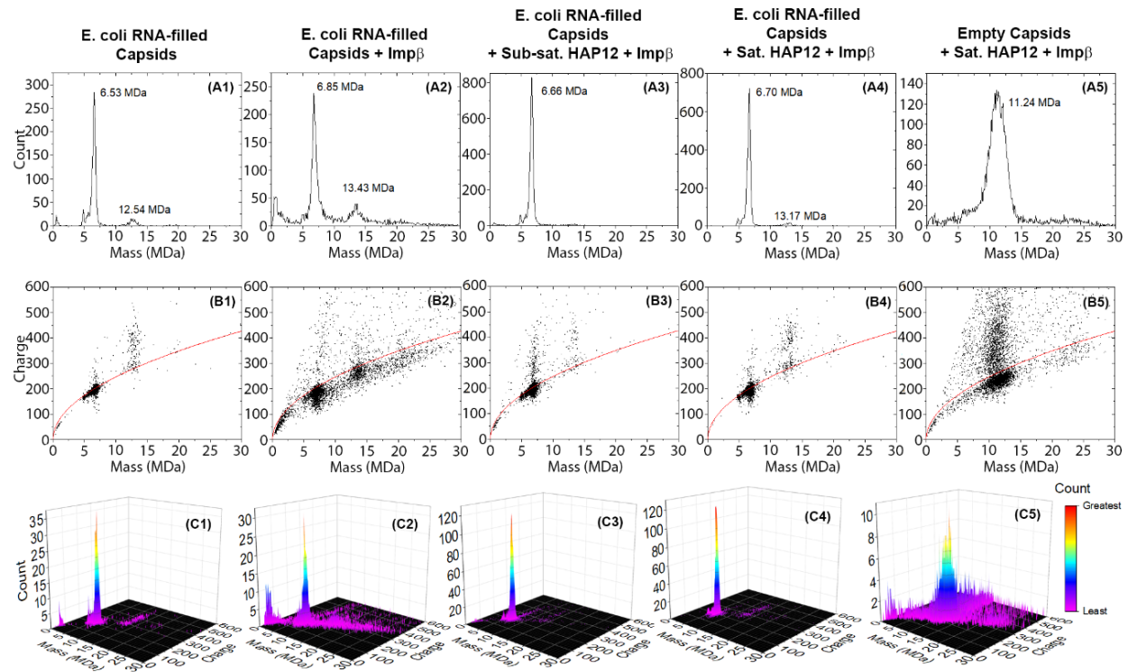
Supplementary Figure 4. CDMS of E. coli RNA-filled capsids \pm Imp \beta \pm HAP12 showed no significant shifts in mass and charge. Panels: A1-A5 mass spectra, B1-B5 charge vs. mass plots with Rayleigh limit (red curve), and C1-C5 3D heatmaps. For E. coli RNA-filled capsids, no mass shifts were observed despite addition of Imp \beta or HAP12. For all E. coli RNA capsid samples, a concentration of ions was detected along the Rayleigh limit, suggesting spherical capsids. The 3D heatmaps show that E. coli RNA capsids fall into a single population of ions. Conversely, after addition of super-saturating HAP12 and Imp \beta , empty capsids undergo a mass shift and ion population changes that are similar to empty capsids treated with saturating HAP12 (Figure 6).
