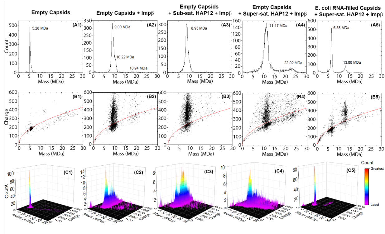
Figure 6. CDMS of empty capsids \pm Imp \beta \pm HAP12 showed shifts in mass and charge. Panels: A1-A5 mass spectra, B1-B5 charge vs. mass plots to identify individual ions (the Raleigh limit (red) shows the theoretical limit for the of charges on a spherical ion), and C1-C5 3D heat maps to identify distributions of populations. For empty capsids, mass shifts indicated Imp \beta binding to capsids. Most capsids showed two charged populations: a population near the Rayleigh limit, suggesting spherical particles, and a second, higher charged plume, suggesting extended or highly textured structures. Columns 1-4 show how empty capsids change mass and charge distributions in response to Imp \beta and/or HAP12. E. coli RNA-filled capsids (column 5) \pm Imp \beta \pm HAP12 exhibited no significant changes in their mass spectra, charge vs. mass plots, or 3D heatmaps.
