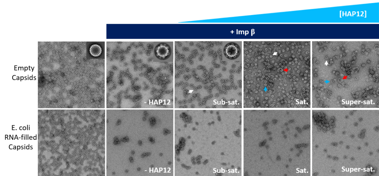
Figure 4. HAP12 with Imp \beta led to disruption of empty capsids. Empty and E. coli -RNA-filled capsids were mixed with Imp \beta so that there were 80 Imp \beta per capsid (Cp183 dimer and Imp \beta concentrations were 11.9 \mu M and 8 \mu M respectively), dialyzed into low salt (150 mM NaCl) to facilitate binding, and visualized by negative stain TEM. Relative HAP12 concentrations are shown in white. Arrows highlight capsids of specified morphology: white arrows – round, “normal”, capsids; blue arrows – deformed/intact capsids; red arrows – broken capsids/aberrant structures. Drug-free empty capsids appeared spherical and intact, which is reflected in its representative 2D particle projection (inset). After addition of Imp \beta , capsids with no HAP12 or sub-saturating HAP12 concentrations similarly appeared round and intact; each have representative cross-sections that show well-ordered, external Imp \beta density (insets and Supp. Figure 2). Introduction of Imp \beta and saturating or higher concentrations of HAP12 to empty capsids produced broken capsids and heterogenous complexes (see also Figure 5). E. coli RNA-Filled capsids remained morphologically unchanged even with treatment with high concentration of HAP12.
