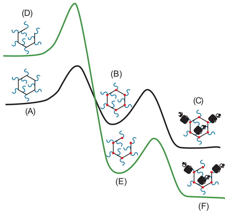
Figure 7. Free energy diagram of an empty capsid in its strained (A-C, black) and ruptured (D-F, green) states mediated by HAP12 and Imp \beta . Free energy schematics for a strained (A-C) or ruptured (D-F) empty capsid shown in black and green, respectively. Because it has fewer interdimer contacts, an untreated, ruptured capsid (D) is at a higher energy state than an intact, drug-free capsid (A). After enough HAP molecules (red dots) bind to cause capsid deformation, the strained, intact capsid (B) pays a global strain penalty and is at a higher energy level. By rupturing, a HAP-bound capsid relieves the global strain and achieves a lower energy state (E). Although Imp \beta -binding (black trucks) provides some stability to capsids, this interaction applies further mechanical strain on the capsid (C), which can be energetically compensated by rupturing (F).
