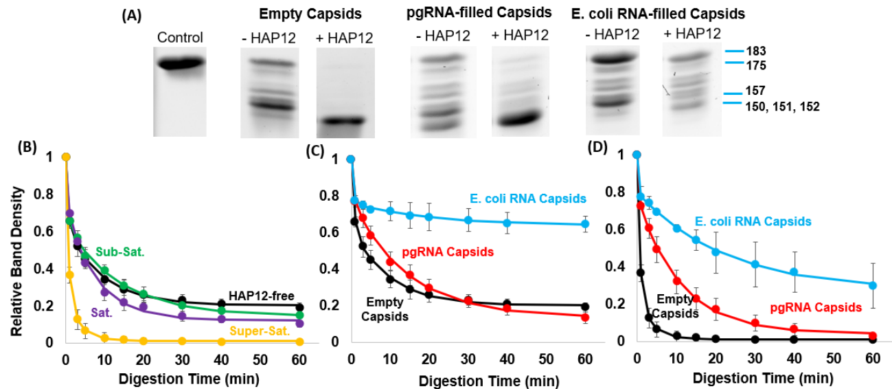
Figure 2. Excess HAP12 changed the proteolysis pattern and led to faster and more complete proteolysis of CTDs. CTD exposure was measured as a function of trypsin digestion. Empty, pgRNA-filled, and E. coli RNA-filled capsids were treated with HAP12 and then exposed to trypsin at room temperature. Capsid and trypsin concentrations were 7 \mu M and 0.04 \mu M, respectively. Reactions were quenched by acidification and analyzed by SDS-PAGE and LC-MS. (A) SDS-PAGE of proteolyzed, drug-free capsids (-HAP12) and capsids treated with super-saturating concentration of HAP12 (+HAP12) capsids; these samples were digested for 60 min. Prominent bands, identified by LC-MS, are labeled on the rightmost image. Untreated capsids retained substantive fractions of intact Cp183. With excess HAP12, the CTDs of empty and pgRNA-filled capsids were almost completely digested; E. coli RNA-filled capsids exhibited about equal distribution of different proteolyzed bands. (B, C, D) Time courses of cleavage at (B) varying HAP12 concentrations, (C) varying capsid content (empty, pgRNA-filled, and E. coli RNA-filled) without HAP12, and (D) varying capsid content with super-saturating HAP12. The relative band density is defined as the optical density of undigested Cp183 divided by the total optical density of the lane.
