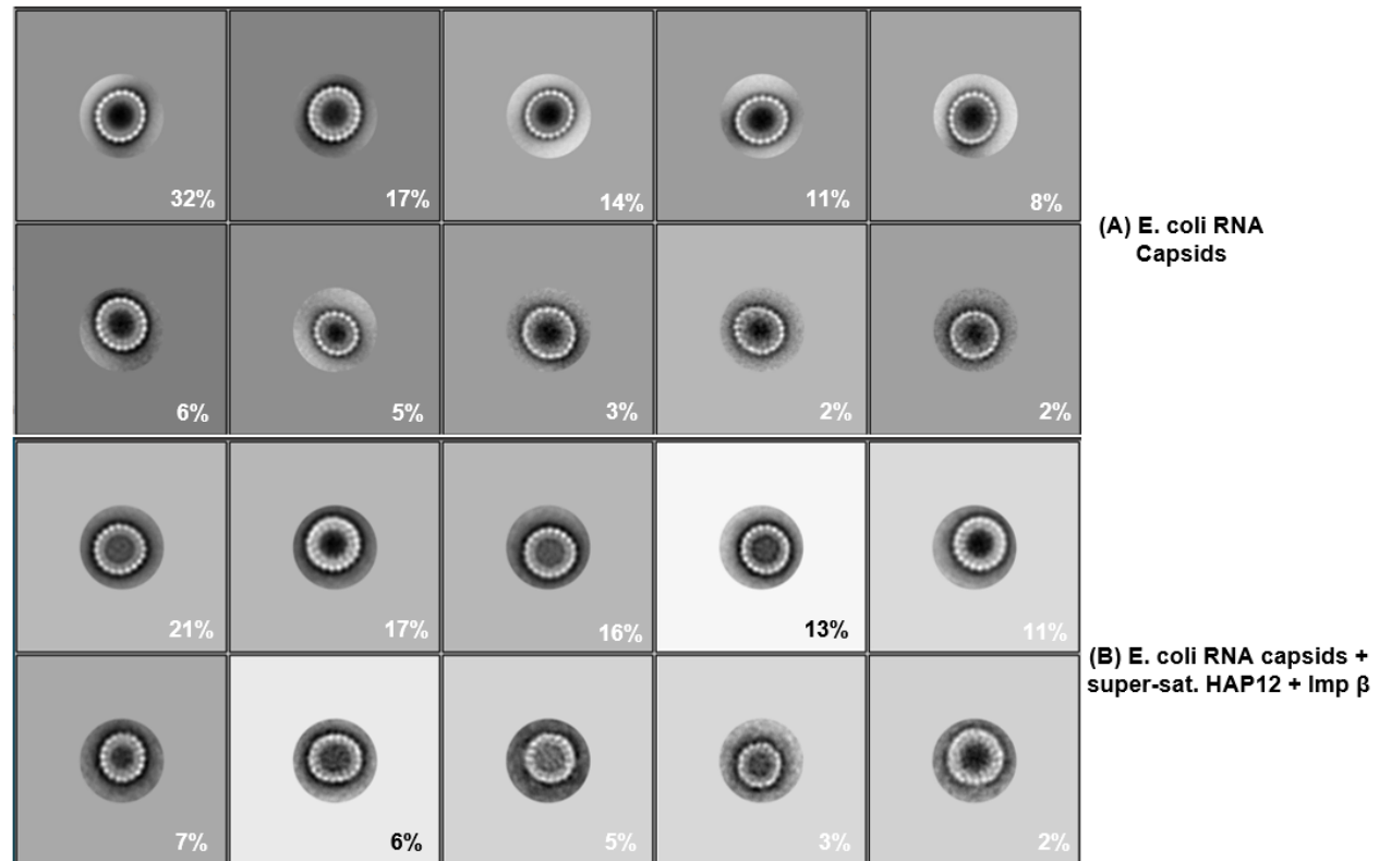
Supplementary Figure 3. After treatment with super-saturating HAP12 and Impβ, E. coli RNA-filled capsids appeared intact and spherical. Class averages of E. coli RNA-filled capsids with no HAP12 (4,319 particles) or with super-saturating HAP12 + Impβ (4,247 particles) were compared for differences on capsid morphology (A and B, respectively). E. coli RNA capsids were prepared as previously stated in Figure 4. Untreated E. coli RNA capsids appeared intact and round (A). Similarly, E. coli RNA capsids treated with super-saturating HAP12 and Impβ also appeared to be intact and spherical, suggesting that internal RNA prevented capsid deformation and disruption (B).
