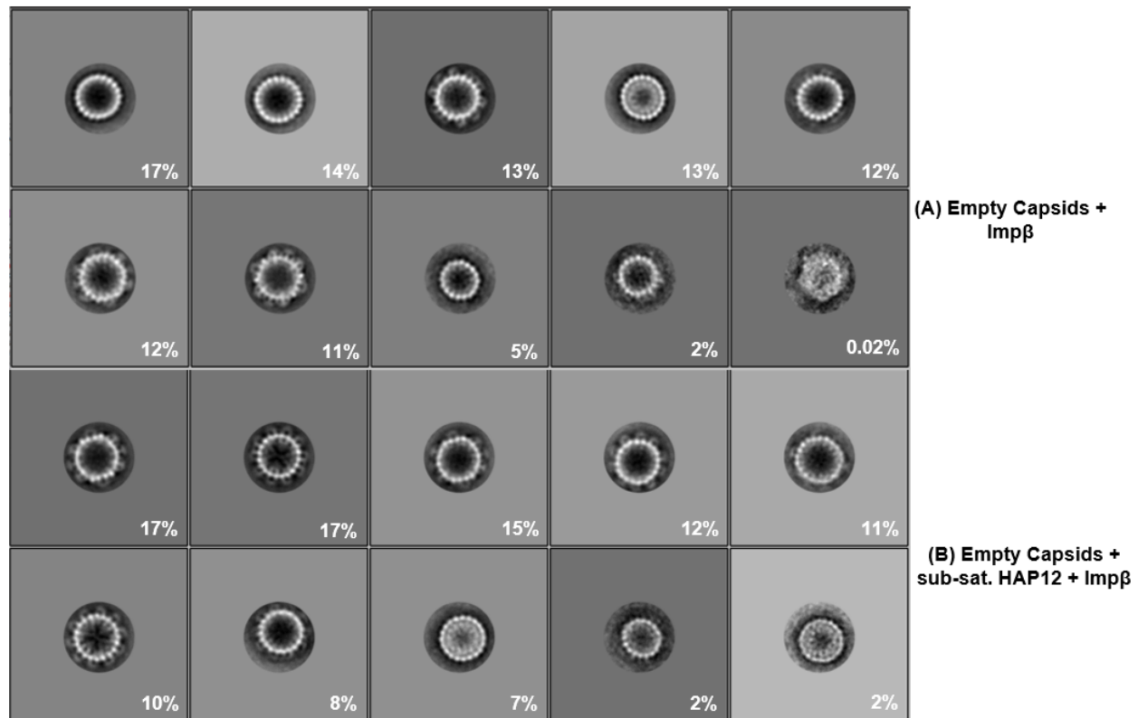
Supplementary Figure 2. Empty capsids treated with sub-saturating HAP12 appeared to have more externally bound Impβ than drug-free capsids. Class averages of HAP-free empty capsids + Impβ (4,718 particles) and empty capsids + sub-saturating HAP12 + Impβ (5,118 particles) were compared for differences on capsid morphology (A and B). Empty capsids were prepared as previously stated in Figure 4. HAP12-free empty capsids showed four classes (48% of total particles) with visible, externally bound Impβ (A). However, capsids treated with sub-saturating HAP12 showed seven classes (90% of total particles) with external Impβ (B). These observations suggested that sub-stoichiometric HAP12 stabilized Cp-Cp interactions, preventing breakage of dimer-dimer contacts and internalization of Impβ.
