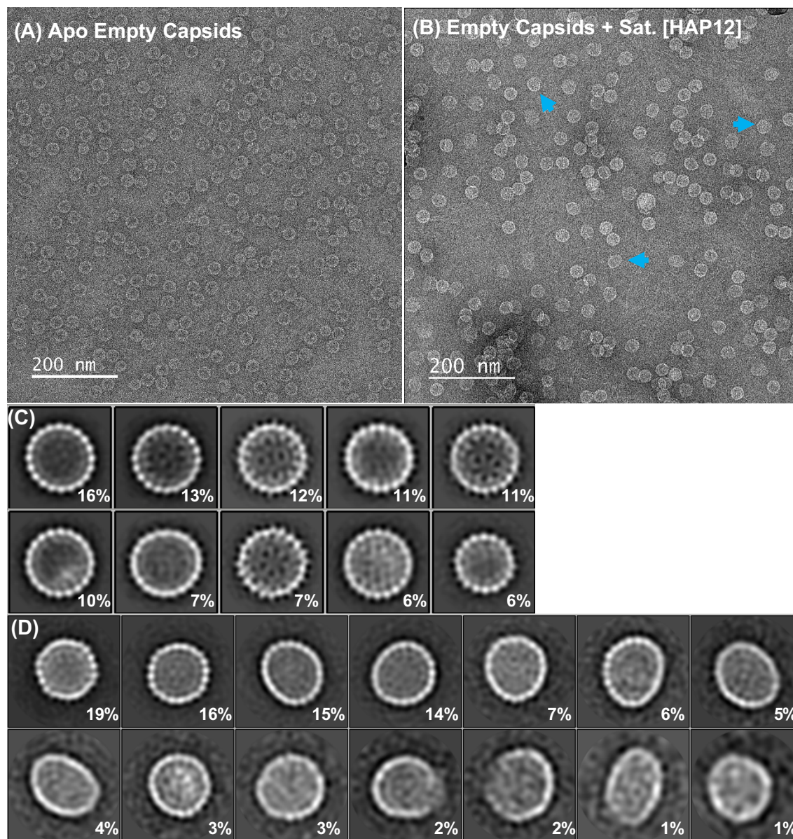
Figure 3. HAP12-treatment causes capsid deformation. Untreated (A,C) and treated (B,D) empty capsids were compared by negative stain EM. (A) A TEM of capsids with no HAP12 shows a narrow range of diversity. (B) A TEM of capsids in saturating HAP12 shows that damage to capsids is evident even without averaging. Blue arrows indicated deformed capsids. Samples were stained with ammonium molybdate with trehalose added to minimize sample flattening and distortion due to drying. (C) Class averages of 5,307 nontreated-capsids from negative stained TEM show a circular cross section. (D) Class averages of 1,160 capsids treated for 2 hours with saturating HAP12, at 25°C, show elliptical, faceted, and broken morphology; capsid deformation by HAP12 is nearly universal but irregular. Population of each class is shown in the bottom right corner.
