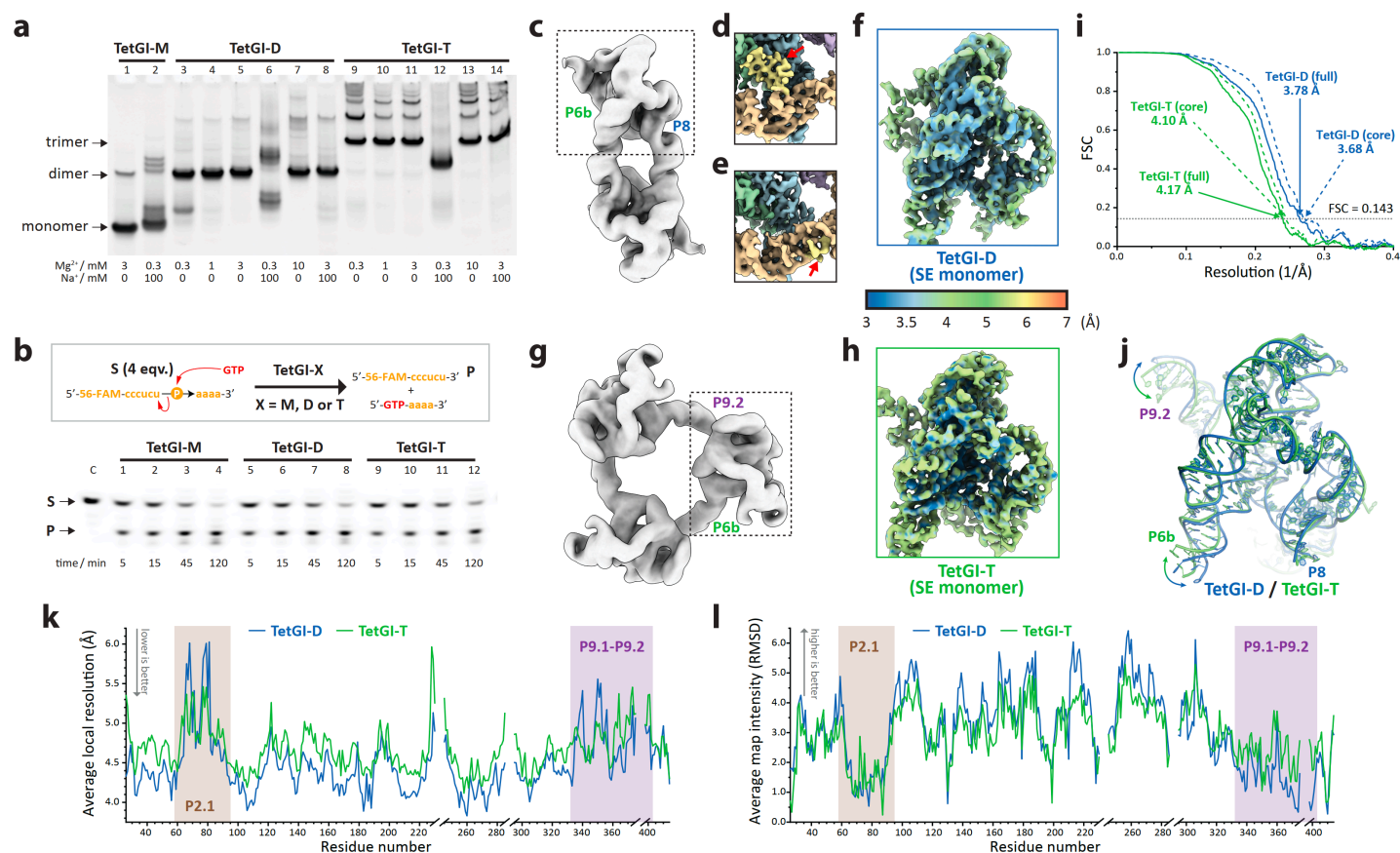
Figure 3 | Assembly, activity and cryo-EM analyses of the dimeric and trimeric post-2S TetGI constructs, TetGI-D and -T. a , Native PAGE analyses of the assembly products under different annealing buffers. TetGI-M is the corresponding monomer control. The bands for the target dimer and trimer, along with the monomer control, are marked on the left of the gel image. b , The TetGI-D and -T constructs are catalytically active as determined by the trans-acting endonucleolytic activity. In the presence of the intron constructs (0.5 \mu M of monomer unit), the substrate (S, 2 \mu M; that is 4 equivalents (eqv.) of intron monomer unit), a 10-nt single-stranded RNA 5' labeled with 6-fluorescein amidite (56-FAM), is cleaved by an exogenous GTP cofactor (1 mM) at 37 °C. c , Cryo-EM map of TetGI-D dimer refined with C_2 symmetry. d, e , 3D classification of the SE monomers of TetGI-D results in two distinct conformations with (d) or without (e) the binding of TetLEM. Red arrows point to the docked double-stranded P1 (in d) and the single-stranded IGS (in e) that interacts with the minor groove of P2.1. f , Local resolution map of the SE monomer of TetGI-D refined by combining the two classes in d and e. See Supplementary Figure 7 for details of the reconstruction workflow for TetGI-D. g , Cryo-EM map of TetGI-T trimer refined with C_3 symmetry. h , Local resolution map of the SE monomer of TetGI-T. The shown map is also refined by combining the two classes corresponding to the conformations with double-stranded P1 and single-stranded IGS (Supplementary Figure 8). i , FSC curves calculated for the full (solid lines) and the core (dashed lines) of the TetGI-D (blue) and -T (green) SE monomer. j , Overlay of the cryo-EM structures of TetGI-D (blue) and -T (green). Double-headed arrows mark the structural movement of P6b and P9.2 of the two structures. k, l , Plots of the atom-averaged local resolution (k) and map intensity (l) calculated for each residue of TetGI-D (blue) and -T (green). Though TetGI-T has an overall lower map quality (marked by higher values in k and lower values in l) than TetGI-D, it has comparable or better map quality in the regions of P2.1 and P9.1-P9.2 (highlighted by brown and purple shades, respectively) because these peripheral domains are geometrically restrained in TetGI-T.
