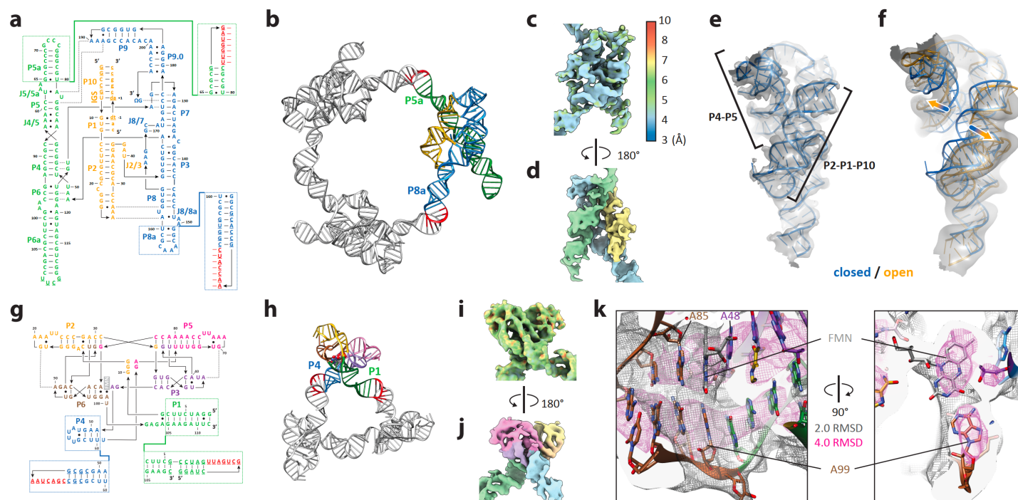
Figure 5 | The homomeric self-assembly strategy applied to two smaller structured RNAs. a , Sequence and secondary structure of the AzoGI. Dashed boxes mark the engineering of P5a and P8a in the construct for trimeric self-assembly, AzoGI-T. b , Computer model of the assembled homotrimer of AzoGI-T. c, d , Cryo-EM maps rendered by local resolution ( c ) and coloring based on the secondary structure in a ( e ). e, f , A comparison of the refined cryo-EM maps of the best-resolved (4.9 Å; the same as the map in c, d ) class of particles corresponding to the closed conformation ( e ) from 3D classification of the SE monomer and another less-resolved (~8.0 Å) one corresponding to the open conformation. In f , the fitted atomic model of the open conformation (orange) is overlaid with that of the close conformation (blue) and the arrows mark the structural movement of P2-P1-P10 and P4-P5. g , Sequence and secondary structure of the Fusobacterium nucleatum FMN riboswitch. Dashed boxes mark the engineering of P1 and P4 in the construct for trimeric self-assembly, FMNrsw-T. h , Computer model of the assembled homotrimer of FMNrsw-T. i, j , Cryo-EM maps rendered by local resolution ( i ) and coloring based on the secondary structure in g ( j ). The color keys for local resolution of i are the same as those shown in c . k , Clipped views showing the cryo-EM map of the FMN ligand and its binding environment. The cryo-EM map is rendered at two different contour levels (grey mesh at 2.0 RMSD and magenta mesh at 4.0 RMSD).
