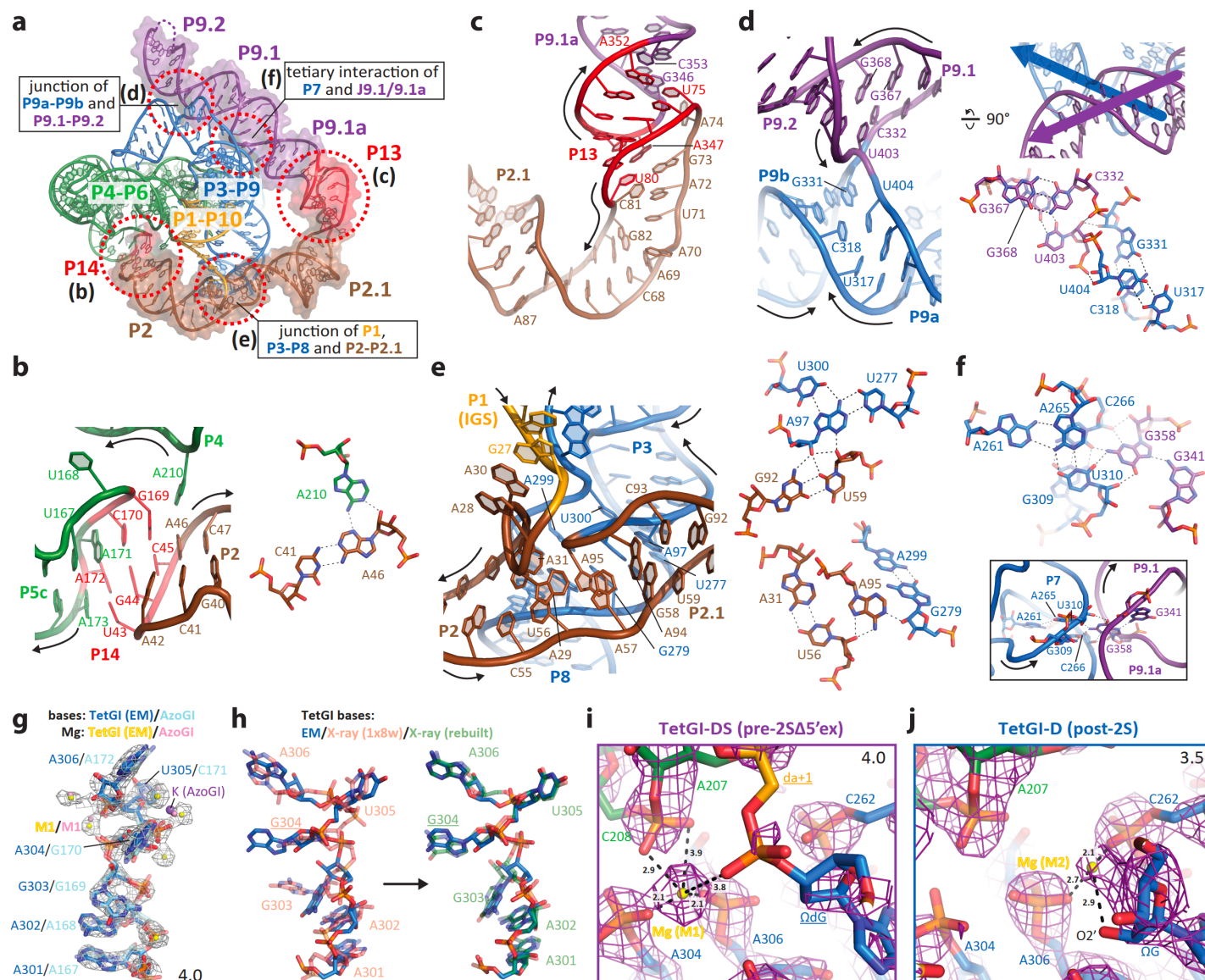
Figure 4 | Structural insights gained from the cryo-EM structures of the TetGI. a , An overview of tertiary interactions and junction structures involving the peripheral domains (highlighted by surface rendering) of the TetGI. Unless specified otherwise, the TetGI structural elements are from the atomic model of TetGI-DS. b , c , Structural details of the tertiary interactions P14 ( b ) and P13 ( c ). Right panel of b shows the base-triple formed by the bulged-out A210 from P4 and the noncanonical C41:A46 pair from P2. d , e , Structures of the four-way junction (4WJ) at P9a-P9b and P9.1-P9.2 ( d ), and the junction at P1, P3-P8 and P2-P2.1 ( e ). Insets of d show the strand directions of the continuous strands of the 4WJ (top-right), and the interaction details at the crossover site (bottom-right). Top-right and bottom-right insets of e show the details of two tertiary contacts between the P2-P2.1 and P3-P9 domains. f , The tertiary contact formed by the docking of G358 of J9.1/9.1a into the minor groove of P7. g , A comparison of the J8/7 region of the TetGI-DS cryo-EM structure and the Azoarcus group I intron (AzoGI) crystal structure 36 (PDB code: 1u6b) reveals close structural resemblance. Gray mesh is the EM map of the TetGI contoured at 4.0 RMSD level and carved within 2.0 Å of the displayed atoms. h , The high-resolution cryo-EM structure enables the rebuilding and re-refinement of J8/7 of the previous crystal structure of the TetGI core 35 (PDB code: 1x8w). The structures before (light red) and after (light green) rebuilding are overlaid with the TetGI EM structure (blue). Underlined nucleotides indicate the mutations introduced for the crystallographic study. i , j , Active-site Mg 2+ ions, M1 and M2, are observed in the EM maps (magenta meshes) of TetGI-DS ( i ) and TetGI-D ( j ), respectively. In the second step of splicing, M1 activates the attacking nucleophile and M2 stabilizes the leaving group. Dashed lines mark the distances (Å) between the Mg 2+ ions and RNA heteroatoms.
