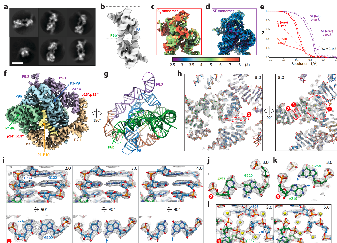
525 Figure 2 | Sub-3 Å resolution cryo-EM map of TetGI-DS, a dimeric pre-2SA5'ex construct of the TetGI, enabled by ROCK. a, 526 Representative 2D class averages of TetGI-DS dimer. Scale bar is 10 nm. b, Cryo-EM map of TetGI-DS dimer refined with C 2 symmetry. 527 c-e, Reconstruction with symmetry expansion (SE) improves the resolution as indicated by the local resolution maps of the monomer 528 from the C 2 dimer (C 2 monomer, c) and the monomer after SE (SE monomer, d), and by the Fourier shell correlation (FSC) curves (e) 529 calculated for the full (solid lines) and the core (dashed lines) of the C 2 monomer (red) and SE monomer (purple). f, g, Cryo-EM map 530 (f) and the derived atomic model (g) colored according to the secondary structure in Fig. 1b. h, Two clipped views of the map (grey 531 mesh) with the atomic model (sticks for RNA and yellow spheres for Mg 2+ ions) illustrating the quality of the high-resolution cryo-EM 532 map. Numbers in the corners of the figure panels (through all figures in this work) indicate the root mean square deviation (RMSD, 533 analogous to \sigma for X-ray crystallography maps) contour level of the raw EM map (without any zoning or carving applied unless specified 534 otherwise). Numbered (1 through 4) red dashed boxes mark the regions in i-l. i-l, Detailed views of an example WC bp (G100:C274, i), 535 a wobble bp (G220:U253, j), a non-canonical bp (A219:G254, k), and a region enclosing five Mg 2+ ions (l). Blue arrows point to the 536 feature in the map corresponding to exocyclic amino groups. In i, two views related by a rotation of 90° are shown with maps rendered 537 at three different contour levels to show the map features of base-to-base separation and sugar-phosphate backbone. In l, the same area 538 is shown with maps rendered at two different contour levels to show the strong map intensities of Mg 2+ ions.
