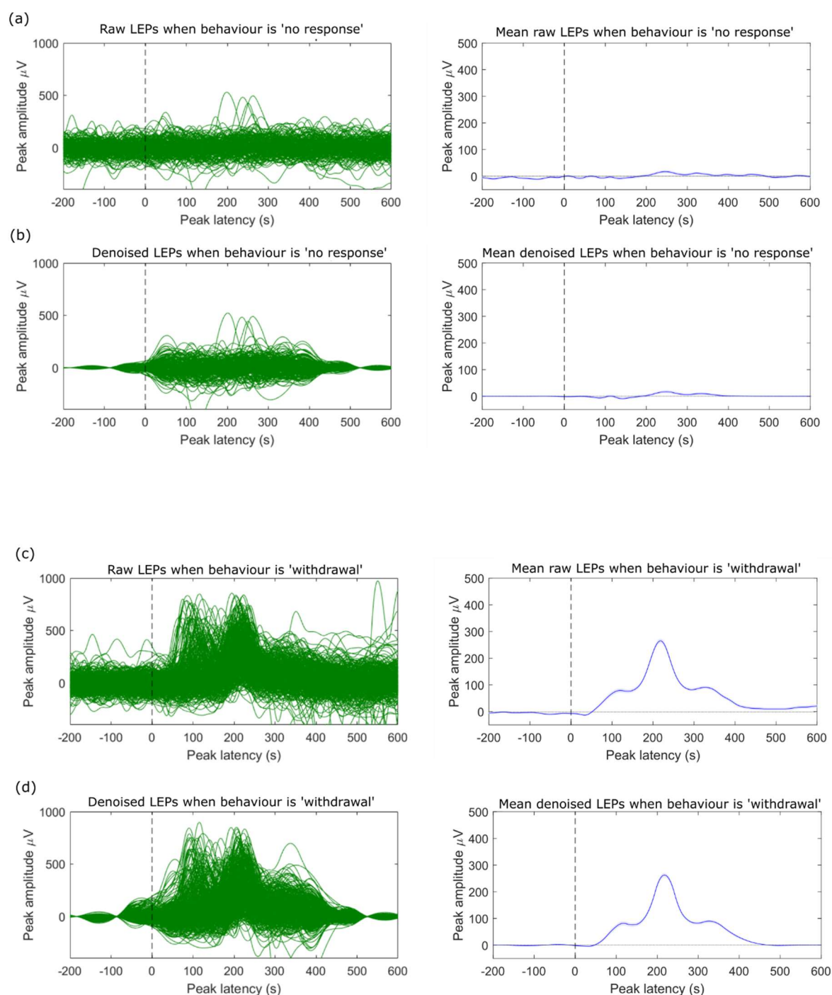
Supplementary Figure 2. (a-b) For behaviours classified as no response, most individual vertex LEPs do not rise above the noise (left hand plots). Little/no clear peak is apparent in the mean of either the raw or denoised data.(c-d) For the withdrawal responses, peaks rise clearly above the noise in both raw and denoised versions. Note that in the averaged data for these LEPs, the two groups of peaks have merged into one peak with 'shoulders' either side.
