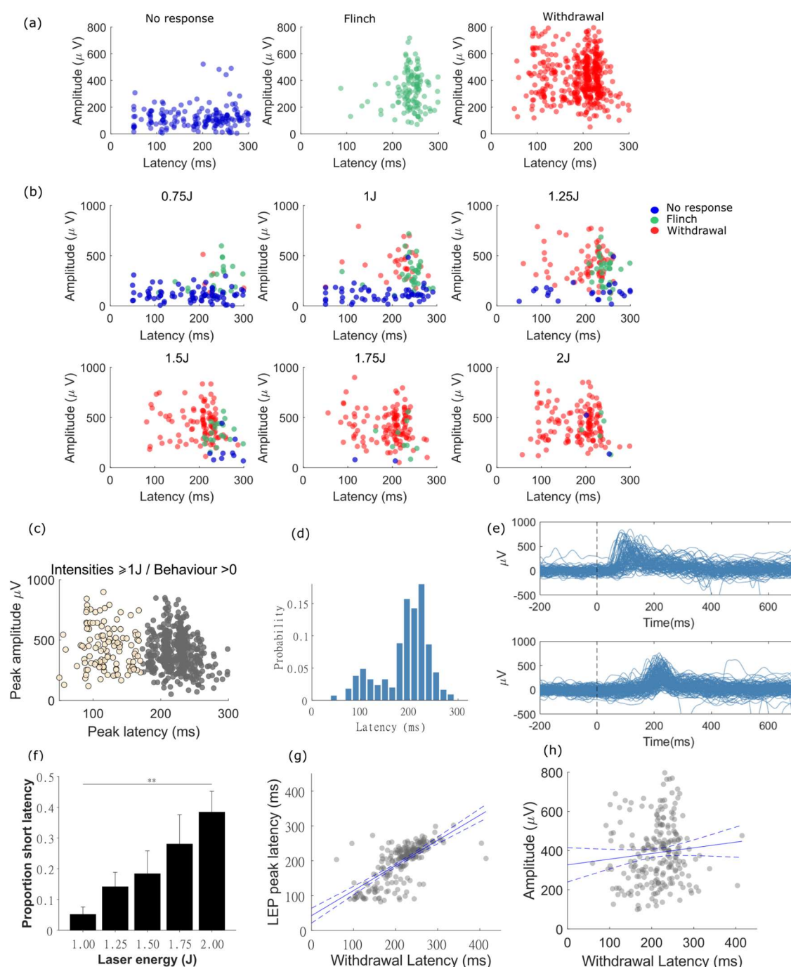
Figure 4 LEPs grouped by latency and amplitude. (a) denoised LEP peak amplitude and latency plotted by behaviour, and (b) laser energy (behavioural response indicated by colours, as used in (a)) showing the appearance of two groups at higher intensities/behavioural responses. (c) LEPs at energies \geq 1J and behavioural scores > 0 , can be split using k-means clustering to form two groups (d) a bimodal distribution is apparent in the probability histogram of latencies for this set reflecting the presence of responses with short and long latencies centred at \sim 120 and \sim 220 ms (e) 150 randomly selected examples of raw (non-denoised) LEPs identified as short (upper) or long (lower) latency using denoising and k-means clustering. Note that both groups have single peaks at either short or long latency and not both. (f) The proportion of short latency events increases with increasing laser energies (Repeated-measures Friedman test, Dunn's correction). (g,h) Relationships between withdrawal latencies and LEP latencies/amplitudes, with regression lines and 95% confidence intervals. ** p < 0.01 .
