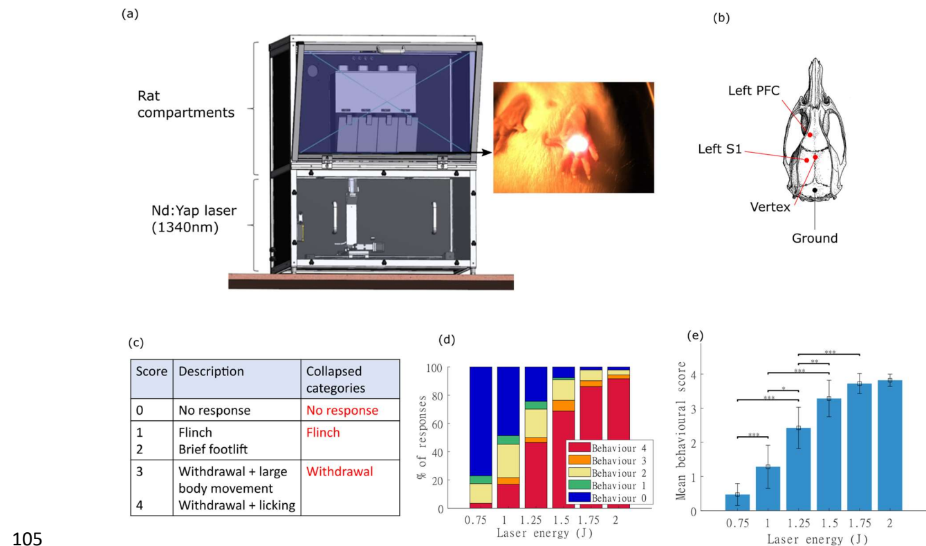
Figure 1 Overview of experiment and behavioural responses. (a) Apparatus overview. Four individual rat compartments were located on a glass floor above a fibre optic cable which transmitted the light from an infra-red Nd:YAP laser. With the aid of a camera in the lower compartment, a motorised xy-stage allowed remote targeting of the laser to the plantar surface. (b) Location of selected skull screws implanted in rats and used for recording EEG (c) Descriptions of behavioural score categories of the response to laser stimulation, with 'full' and 'collapsed' categories. (d) Proportions of behavioural responses in each category for each laser energy (across all animals) showing the increase in the behavioural response with laser energy. Note few responses were scored as '1' or '3'. (e) Distribution
