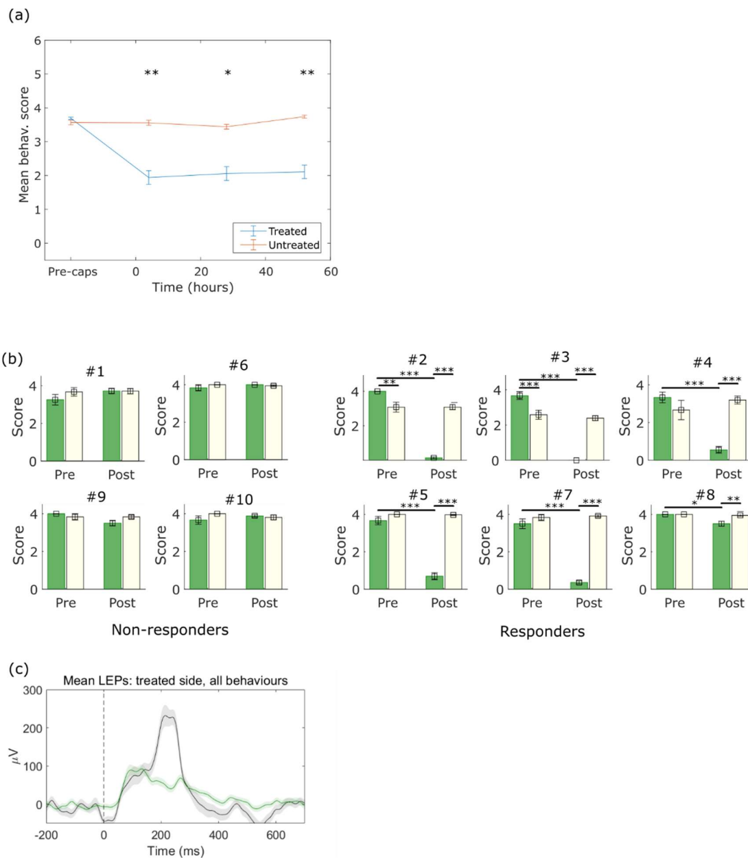
Supplementary Figure 4. (a) Mean behavioural responses at all timepoints (all animals), pre- and post-capsaicin. (b) Breakdown of behavioural responses by animal, categorized as responders and non-responders. (c) Mean LEP pre and post capsaicin over all behavioural responses for the responder group.
