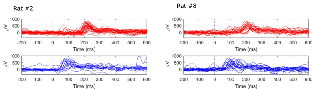
Supplementary Figure 3. Distinct sets of LEPs at short and long latency are seen within the datasets for individual animals.
