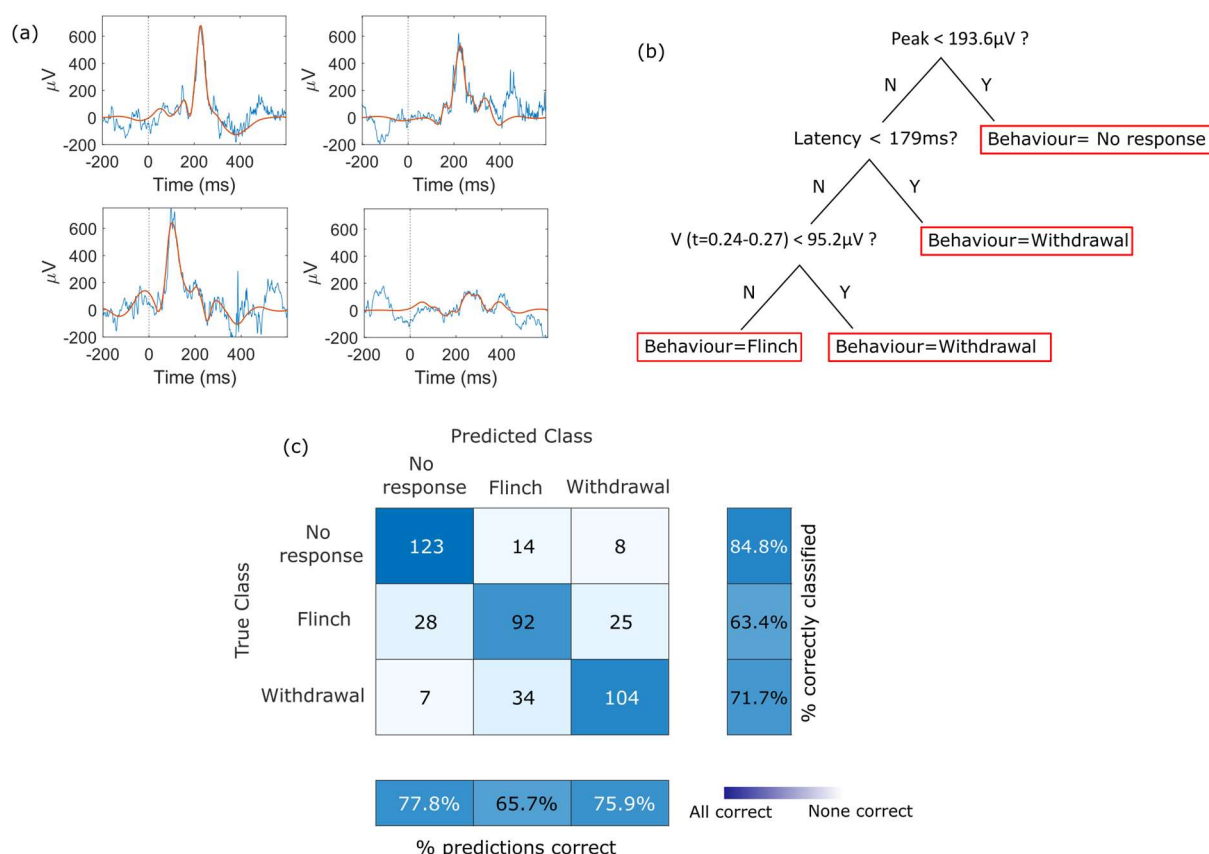
Figure 3 Decision tree classification of individual LEPs. (a) Examples of raw (blue) and denoised (red) single LEPs. (b) Final trained coarse decision tree model for classifying individual LEPs by behavioural response. (c) Matrix illustrating key performance indicators of the coarse decision tree, from 5-fold cross validation training (see main text). Raw values show the number of trials in specific combinations of predicted/true results, e.g. in the top middle square, there were 14 examples of events which were predicted to be in category ‘flinch’ but were actually in category ‘no response’. Summary statistics around the matrix represent the percentage predictions that were correct (bottom) and the percentage of actual results which were correctly classified (right).
