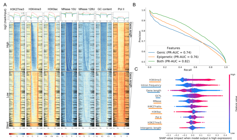
Figure 7. Prediction of gene expression by epigenetic marks
