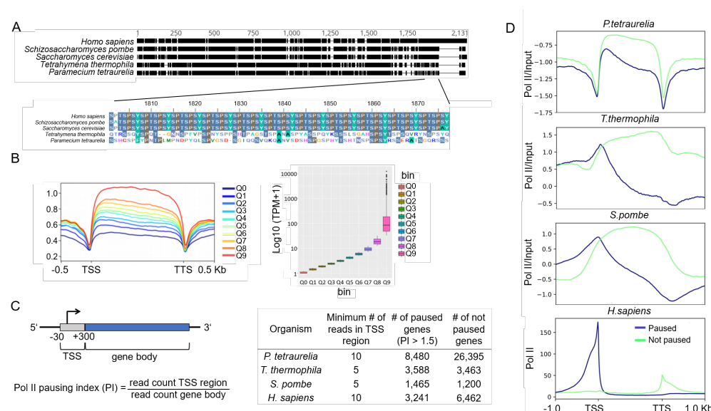
Figure 6. Analysis of RNA polymerase II pausing
