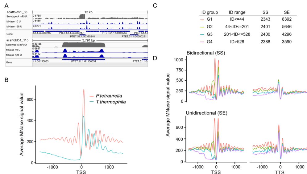
Figure 3. MNase - seq results reveal well positioned +1 nucleosomes.
