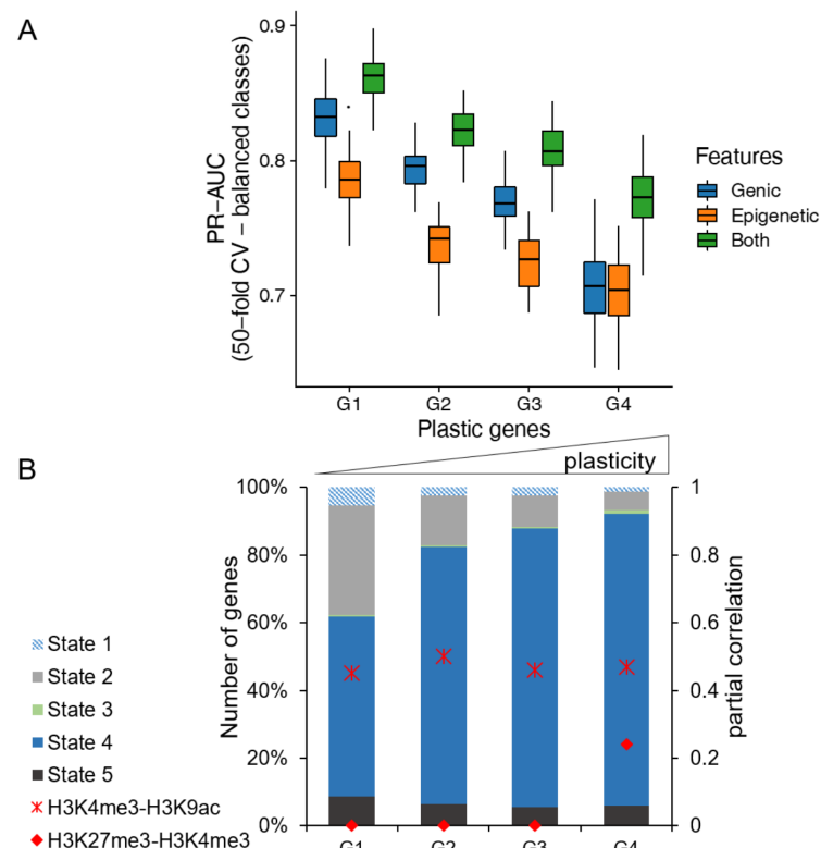
Figure 8. Prediction of gene expression for genes with high plasticity.
