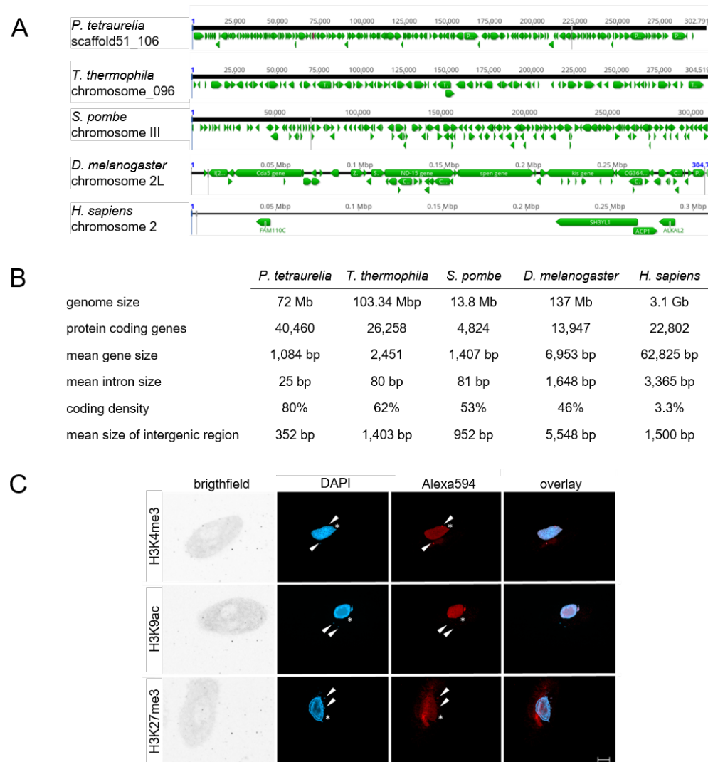
Figure 2. Features of the Parametium genome in comparison to other organisms.
