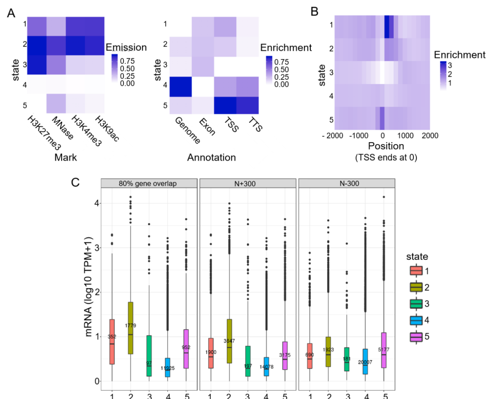
Figure 5. Segmentation analysis using ChromHMM.
