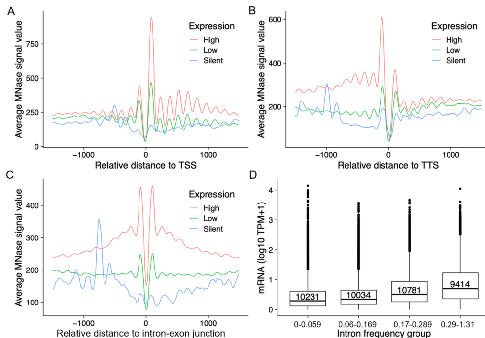
Figure 4. Positioning of nucleosomes in correlation to gene expression.
