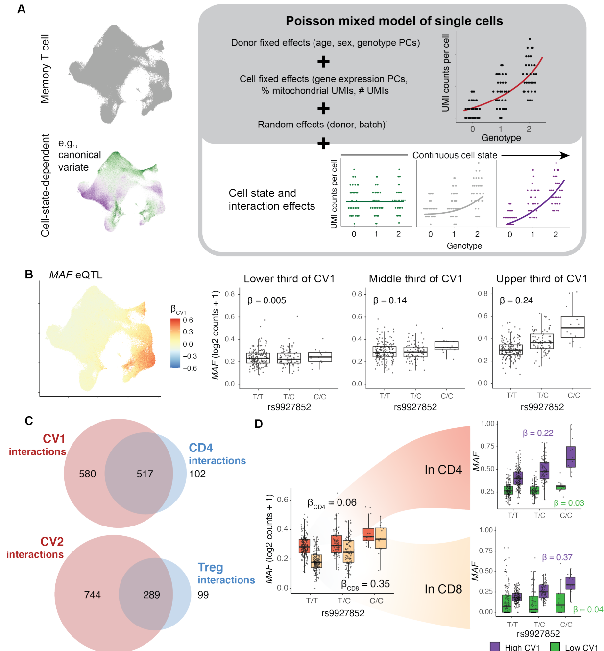
Fig. 3. Modeling eQTL interactions with continuous cell states across single cells. (A) Schematic of Poisson mixed effects model for cell-state-dependent single-cell eQTL analysis. After adjusting for covariates and modeling random effects, we can measure the interaction between a continuous cell state (shown here binned into low/medium/high for ease of visualization) and genotype. (B) Interaction of rs9927852 eQTL for MAF with CV1. UMAP of total effect size ( \beta_{total} = \beta_G + \beta_{CV1} \cdot CV1 \text{ score} ) per cell. Box plots show eQTL effect for cells in the bottom (left), middle (center), and top (right) thirds of CV1 scores. (C) Venn diagrams of the number of eGenes with significant CV
