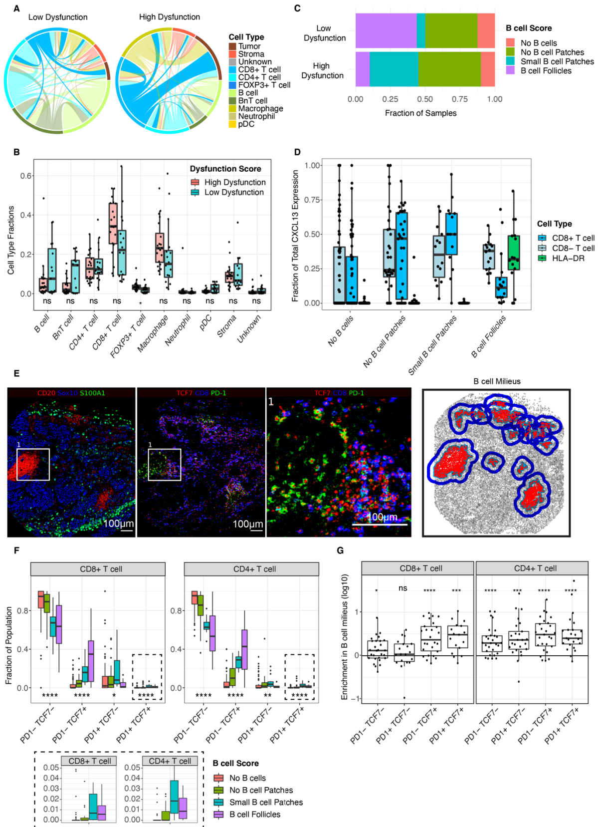
Fig. 5 – TLS are associated with lower levels of dysfunction and naïve, stem-like T cells
