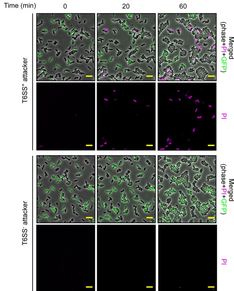
Figure 5. Operon-mediated toxicity results in prey cell lysis. Time-lapse microscopy of competition between V. parahaemolyticus \Delta hns (T6SS + ) or \Delta hns/\Delta hcp1 (T6SS - ) attackers and V. parahaemolyticus \Delta vp1389 prey that express GFP. Attacker and prey were mixed (2:1 ratio) and spotted on LB agarose pads supplemented with propidium iodide (PI; pink). Merging of the phase contrast, GFP (green), and PI (pink) channels, as well as the PI channel alone are shown. Scale bar = 5 \mu m.
