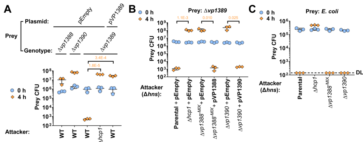
Figure 2. VP1388 and VP1390 are required for antibacterial toxicity, not immunity. A-C) Viability counts of the indicated V. parahaemolyticus (A-B) or E. coli (C) prey strains before (0 h) and after (4 h) co-incubation with the indicated V. parahaemolyticus attackers on media containing 3% NaCl at 30 °C. In A, prey strains contain either an empty plasmid (pEmpty) or a plasmid for arabinose-inducible expression of VP1389 (pVP1389). In B and C, prey strains contain an empty plasmid that provides a selection marker, and the attackers are derivatives of a \Delta hns mutant (parental). In B, the attackers contain an empty plasmid, or plasmids for the arabinose-inducible expression of VP1388 (pVP1388) or VP1390 (pVP1390). Data are shown as the mean \pm SD. Statistical significance between samples at the 4 h timepoint by an unpaired, two-tailed Student's t -test is denoted above. A significant difference was considered as P < 0.05 . DL, assay detection limit. \Delta hcp1 was used as a T6SS1 - control strain.
