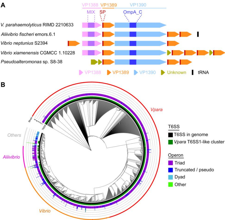
Figure 1. vp1388-90 homologous operons are widespread in T6SS-encoding marine bacteria. A) Selected examples of the genetic structure of vp1388-90 homologous operons. SP, signal peptide; MIX, Marker for type sIX effector. B) Distribution of vp1388-90 homologous operons in bacteria. A phylogenetic tree of bacteria encoding homologous operons, based on the DNA sequences of rpoB . The presence or absence of T6SS in each genome is denoted in the inner rings (black and dark green). Intermediate bars indicate the number of complete (triad) and partial (dyad or truncated) homologous operons identified in each genome. An external ring denotes the group to which the bacterial strains belong. V. parahaemolyticus ( Vpara ) were annotated separately (red), as were Aliivibrios (pink).
