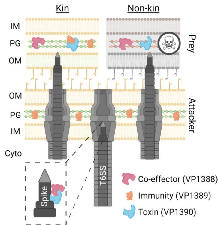
Figure 6. Model of T6SS binary effector delivery. The toxin, VP1390, and its co-effector, VP1388, are loaded together onto the T6SS spike and are delivered into the periplasm of a neighboring prey cell. If the prey cell expresses the cognate immunity protein, VP1389, then it can antagonize the attack (kin). Otherwise, the VP1390 toxin acts in the prey periplasm, leading to cell lysis (non-kin). IM, inner membrane; PG, peptidoglycan; OM, outer membrane; Cyto, cytoplasm. The figure was created using BioRender.com.
