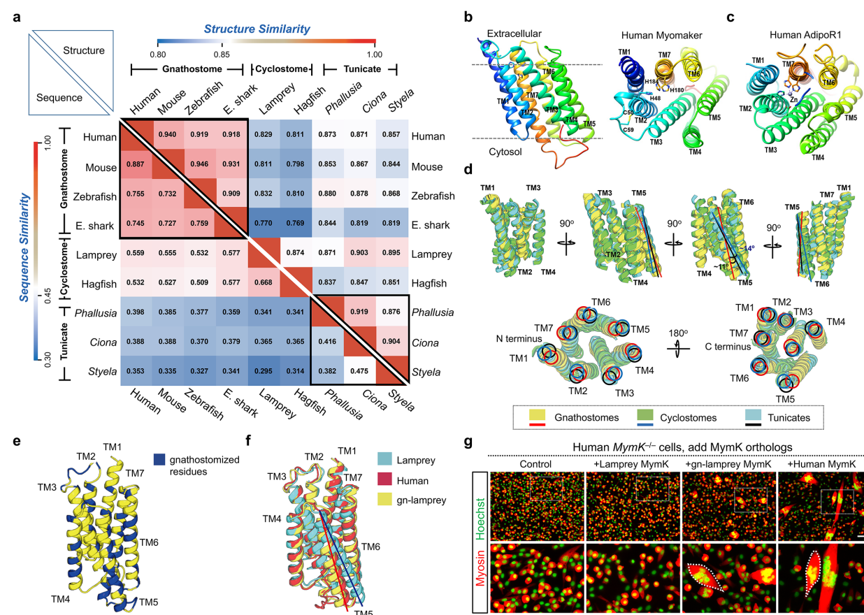
Figure 7: Modeling the structural evolution of MymK proteins.
