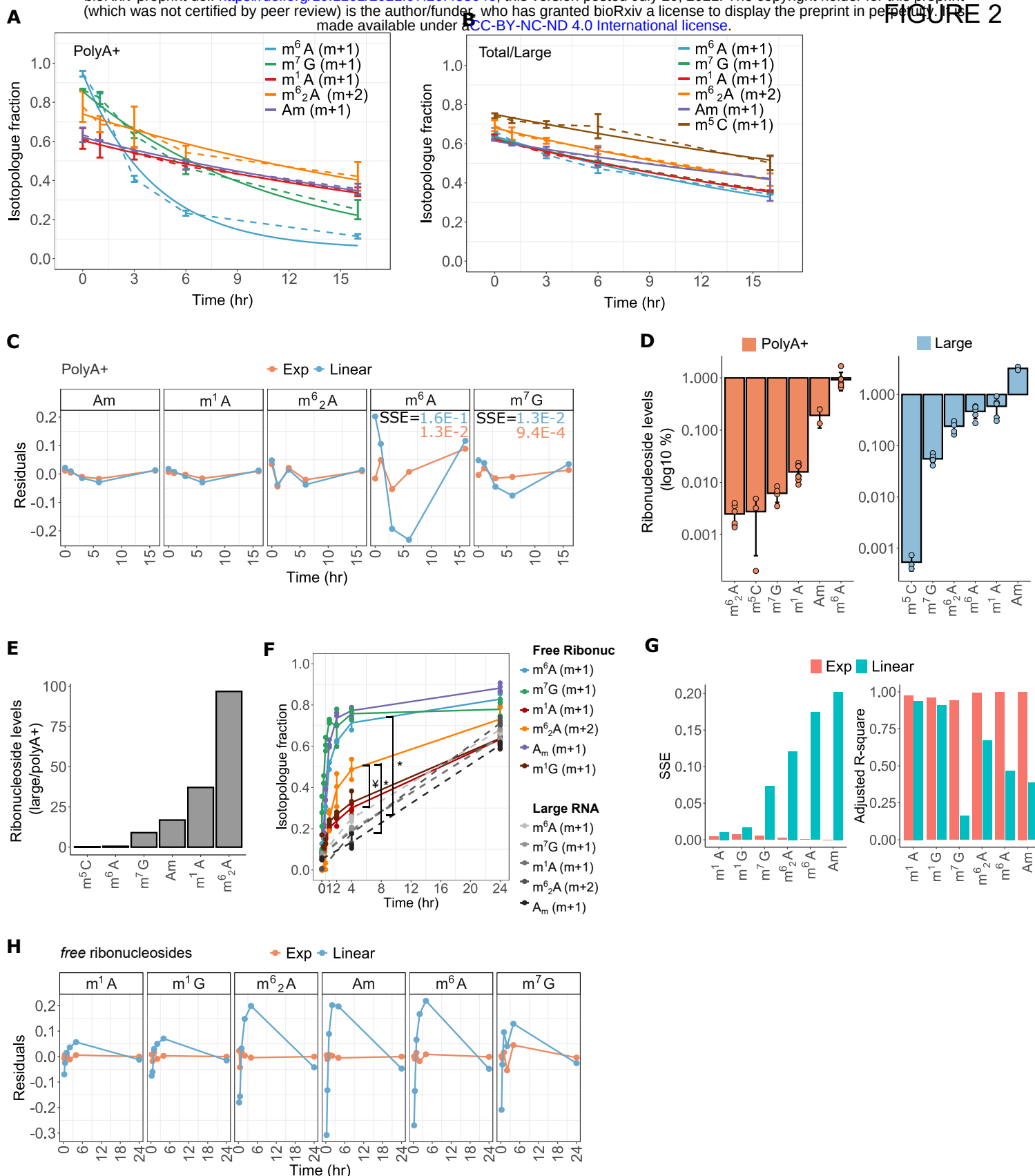
Figure 2. Turnover of modified ribonucleosides in polyA+, ncRNA and free ribonucleoside pool. (A-B) Isotopologue fractions during the ‘chase’ of ^{13}\text{C} -labelled modifications with naturally labelled methionine for 0, 1, 3, 6 and 16 hours, in polyA+ (A) and total/large RNA (B); dashed lines connect data points; solid lines, exponential (A) or linear (B) fit of isotopologue fractions. (C) Residuals of a linear vs. exponential regression of isotopologue fractions in polyA+ RNA in the chase experiment. (D) Normalized ion counts of modified ribonucleosides relative to the ion counts sum of all ribonucleosides, shown for polyA+ and large RNA. (E) Ratio of normalised ion counts between polyA+ and large RNA, as determined in (D). (F) Isotopologue fraction of free ribonucleosides analysed from metabolic extracts; grey datapoints refer to large RNA modifications (Fig. 1E) for comparison. (G-H) Goodness-of-fit of a linear vs. exponential fit of the isotopologue fractions in free modified ribonucleosides. SSE, sum of squared errors. \text{m}^6\text{A} , N6-methyladenosine; \text{m}^7\text{G} , 7-methylguanosine; \text{m}^1\text{A} , 1-methyladenosine; \text{m}^6_2\text{A} , N6,N6-dimethyladenosine; \text{A}_m , 2'-O-methyladenosine; \text{m}^5\text{C} , 5-methylcytidine; \text{m}^1\text{G} , 1-methylguanosine; A, adenosine; G, guanosine. Error bars represent 90% confidence intervals in (a-b), or standard deviation in (d, f) of at least three biological replicates with exception of \text{A}_m (two replicates). In all cases, each replicate is the average of two technical replicates. * denotes P < 0.005 , \ddagger denotes P < 0.05 , of a two-sided Student's t-Test comparing \text{m}^6_2\text{A} and \text{m}^6\text{A} in the free ribonucleoside pool (free ribonuc) to large RNA, or \text{m}^6_2\text{A} to \text{m}^1\text{A} in the free ribonuc pool.
