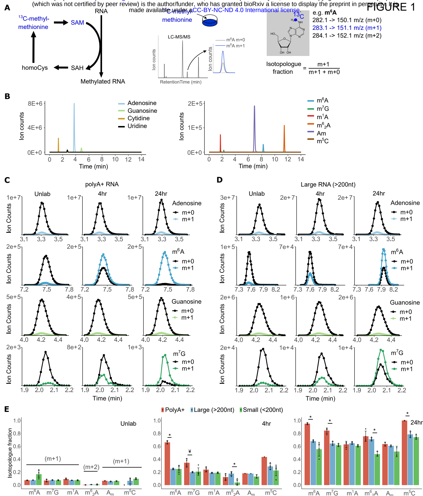
Figure 1. 13 C labelling of RNA modifications across RNA classes. (A) The 13 C-dynamods workflow shows the tracing of RNA methylation: cells are cultured with [ 13 C-methyl]-methionine, the RNA is isolated, digested to ribonucleosides and subjected to LC-MS/MS analysis. The isotopologues detected for m 6 A are shown. (B) Representative chromatogram of unmodified and modified ribonucleosides from total RNA. (C-D) The m+0 and m+1 isotopologues of modified and unmodified ribonucleosides (representative chromatograms) in polyA+ (C) and large RNA (D). (E) Quantification of the isotopologue fractions of each ribonucleoside in polyA+, large and tRNA under unlabelled ('Unlab') conditions, after 4 and 24 hours of culture with [ 13 C-methyl]-methionine. m 6 A, N 6 -methyladenosine; m 7 G, 7-methylguanosine; m 1 A, 1-methyladenosine; m 6 2 A, N 6 ,N 6 -dimethyladenosine; Am, 2'-O-methyladenosine; m 5 C, 5-methylcytosine; m 1 G, 1-methylguanosine; m 2 G, 2-methylguanosine. SAM, s-adenosylmethionine; SAH, s-adenosylhomocysteine; homoCys, homocysteine. Error bars represent standard deviation of three to four biological replicates, with the exception of m 5 C in polyA+-purified RNA (two replicates at 24hr, one replicate in the Unlab/4hr time points). In all cases, each replicate is the average of two technical replicas. * denotes P < 0.005, ¥ denotes P < 0.05, of a two-sided Student's t-Test comparing samples as indicated.
