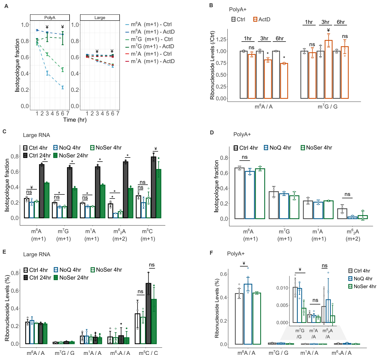
Figure 3. Dynamics of RNA modifications under stress conditions. (A) Isotopologue fractions of modified ribonucleosides in polyA+ and large RNA during a ^{13}\text{C} -dynamods chase experiment in 786O cells cultured with complete DMEM medium (ctrl) or DMEM supplemented with actinomycin D (ActD, 10 \mu\text{M} ); dashed lines connect data points. (B) Normalised levels of \text{m}^6\text{A} ( \text{m}^6\text{A}/\text{A} ) and \text{m}^7\text{G} ( \text{m}^7\text{G}/\text{G} ) in polyA+ RNA derived from ctrl and ActD-treated 786O cells, normalised relative to the ctrl data points in the chase experiment as indicated. (C-D) Isotopologue fractions of modified ribonucleosides in large RNA (C) and polyA+ RNA (D) following [ ^{13}\text{C} -methyl]-methionine labelling under control (ctrl), glutamine (NoQ), or serine (NoSer) deprived conditions. (E-F) Normalised levels of modified ribonucleosides in large RNA (E) and polyA+ RNA (F) in 786O cells cultured with ctrl, NoQ or NoSer DMEM medium for the times indicated. Error bars represent standard deviation of three or more biological replicates, with exception of (A-B), the NoQ condition in (C, E) and \text{m}^6\text{A} under NoSer (D, F) (two biological replicates). In all cases, each replicate is the average of two technical replicates. * denotes P < 0.005 , ¥ denotes P < 0.05 , ns denotes not significant, of a two-sided Student's t-Test comparing stress to ctrl samples, as indicated.
