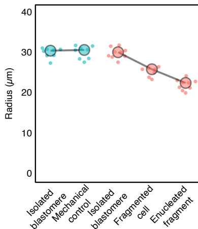
Supplementary Figure related to Figure 2: size of cells before and after fragmentation. Radius of 16-cell stage blastomeres before and after mechanical manipulation ( n = 8 ), fragmentation into fragmented cells ( n= 8 ) or enucleated fragments ( n=9 ). Larger circles show median values.
