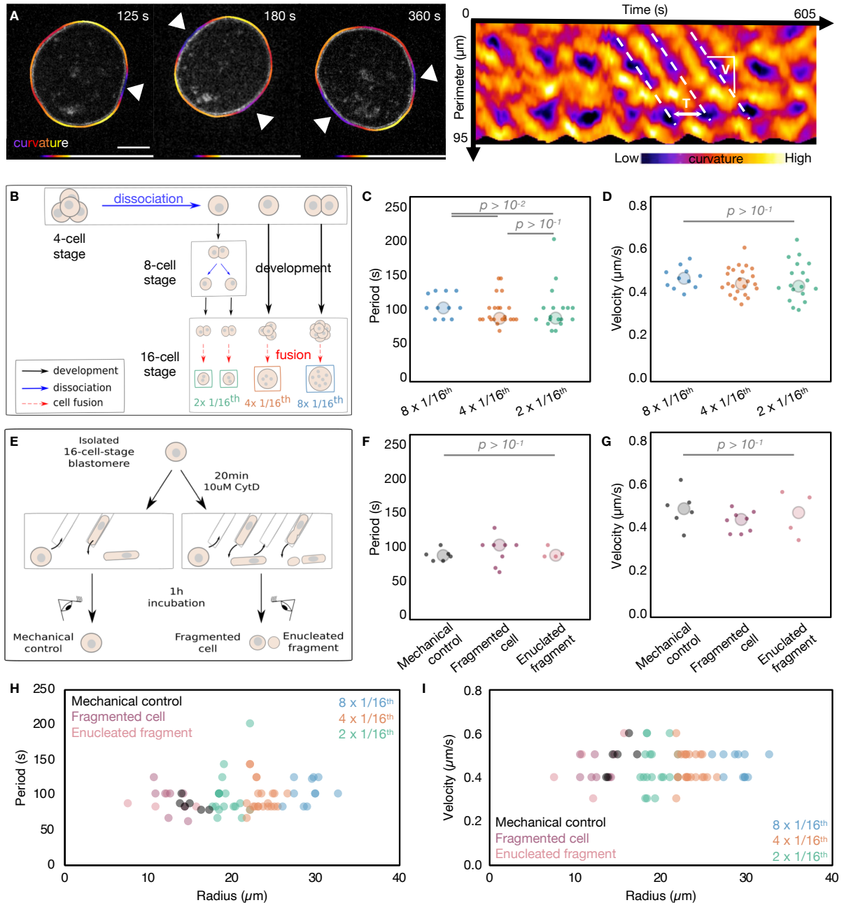
Figure 3: Period and velocity of PeCoWaCo are stable across a broad range of cell sizes. A) Surface deformation tracking for period detection and velocity measurements. Scale bar, 10 μm. B) Schematic diagram of fusion of 16-cell stage blastomeres. C-D) Oscillation period (C) and wave velocity (D) of fused blastomeres. 8 x 1/16 th (blue, n=6), 4 x 1/16 th (orange, n = 12) and 2 x 1/16 th (green, n=7) fused blastomeres are shown. Large circles show median. E) Schematic diagram of fragmentation of 16-cell stage blastomeres. F-G) Oscillation period (F) and wave velocity (G) of fragmented blastomeres. Control (black, n = 6), fragmented cell (magenta, n= 8), enucleated fragment (pink, n=4) are shown. H-I) Oscillation period (H) and wave velocity (I) for size-manipulated 16-cell stage blastomeres. Larger circles show median values. Student's t-test p values are indicated.
