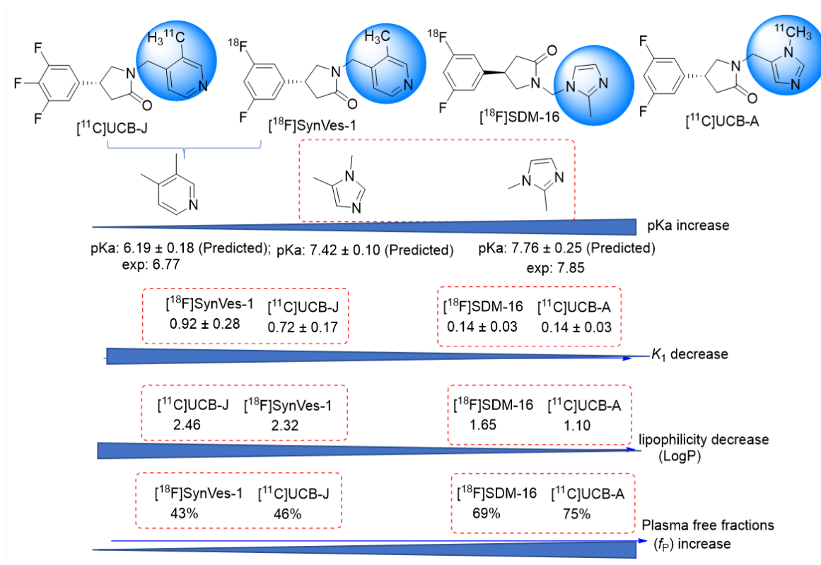
Figure 7: The influence of pK a on the properties of PET tracers.
