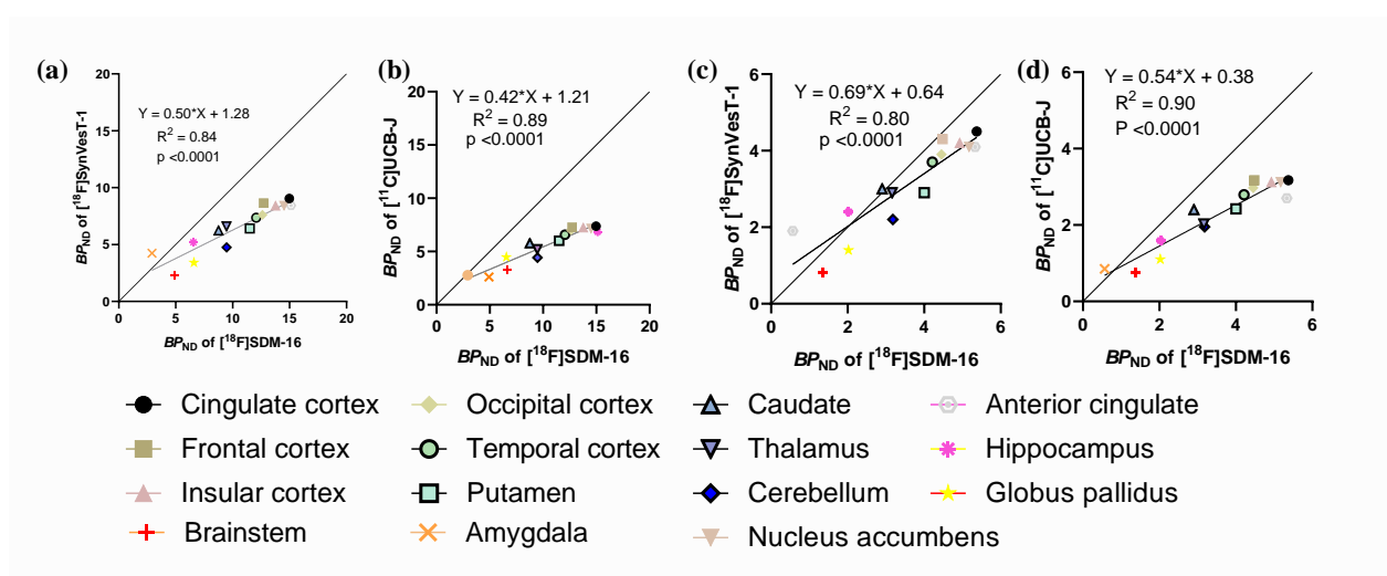
Figure 6: Correlation and linear regression analysis of the regional BP_{ND} values from baseline scans of [^{18}F] SDM-16 with [^{18}F] SynVesT-1 and [^{11}C] UCB-J, using V_{ND} (a, b) or centrum semiovale as reference region (c, d).
