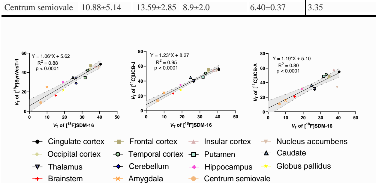
Figure 4: Correlation and linear regression analysis of the baseline 1TC V_T values of [^{18}\text{F}]\text{SDM-16} with that of [^{18}\text{F}]\text{SynVesT-1} [19], [^{11}\text{C}]\text{UCB-J} [26], and [^{11}\text{C}]\text{UCB-A} in monkey brain; dotted lines represent 95% confidence intervals.
