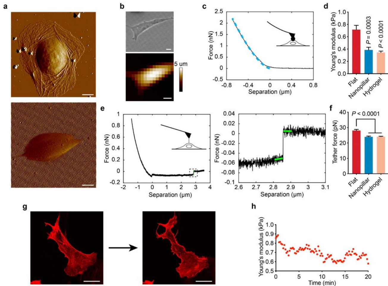
Figure 2. Quartz nanopography reduces cell stiffness and membrane tension in a manner similar to soft hydrogels. (a) Contact-mode AFM deflection images of U2OS cells show different cell shapes on flat quartz (upper) and d200p1h3 nanopillar quartz (lower) surfaces. (b) Optical image (upper) and AFM-obtained topography map (lower) of a U2OS cell on d200p1h3 nanopillar surface. (c) A representative AFM force-separation curve obtained by AFM indentation. The blue dashed line indicates the Hertz fit used to calculate Young's modulus. (d) Quantitative analysis of the Young's modulus of cells obtained by AFM indentation on flat quartz, d200p1h3 nanopillars, and 1 kPa hydrogel ( n = 20, 20 , and 21 cells in flat, nanopillar and hydrogel groups, respectively; mean \pm s.e.m.). (e) Representative AFM retraction curve for pulling membrane tethers (right) and zoom-in view of a tether rupture event (left) in the retraction curve. The difference in the force before and after the rupture (indicated by green lines) is used to calculate the tether force. (f) Quantitative analysis of tether force obtained from cells on flat quartz, nanopillar quartz, and 1 kPa hydrogel surfaces ( n = 21, 21, 22 cells in flat, nanopillar, and hydrogel groups, respectively; mean \pm s.e.m.). (g) Fluorescence images of stress fibers (transfected with LifeAct-RFP) in a U2OS cell before and after 20 min of blebbistatin treatment. (h) Young's modulus of a U2OS cell measured by AFM indentation over the 20 min blebbistatin treatment. P value in comparison to flat surfaces was determined by unpaired two-tailed t test (d, f). Scale bars, 10\ \mu\text{m} (a, b), 20\ \mu\text{m} (g).
