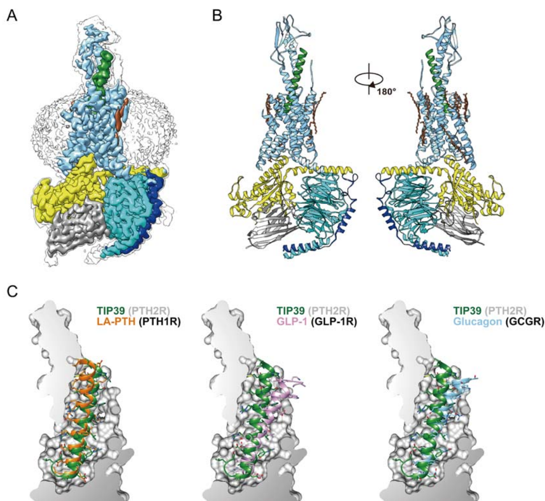
486 Figure 1. The overall cryo-EM structure of the TIP39-PTH2R-G s complex. (A) Cut-through view 487 of the cryo-EM density map that illustrates the TIP39-PTH2R-G s complex and the disc-shaped 488 micelle. The unsharpened cryo-EM density map at the 0.06 threshold shown as gray surface indicates a 489 micelle diameter of 11 nm. The colored cryo-EM density map is shown at 0.12 threshold. (B) Model of 490 the complex as a cartoon, with TIP39 as helix in green. The receptor is shown in blue, Gα s in yellow, 491 Gβ subunit in cyan, Gγ subunit in navy blue and Nb35 in gray. (C) The binding pocket of PTH2R 492 accommodates peptide ligands of class B1 receptors. TIP39 is compared with LA-PTH (left), GLP-1 493 (middle) and Glucagon (right), respectively.
