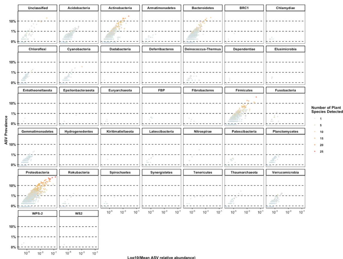
Figure S9: Abundance-occupancy curves for all prokaryotic phyla (Bacteria and Archaea) for the 16S rRNA gene - V4 dataset. Each point represents an ASV and the points are colored based on the number of plant species in which they were detected.
