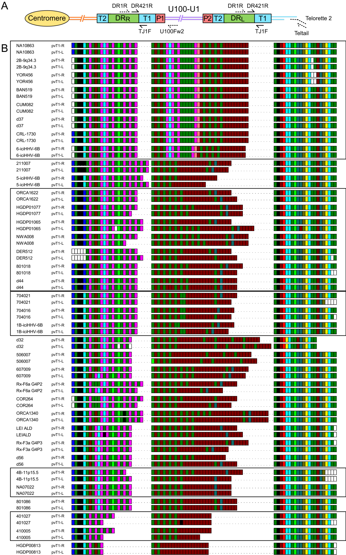
Figure 6 – figure supplement 1. Comparison of pvT1 repeat patterns in DR R and DR L pvT1-L
