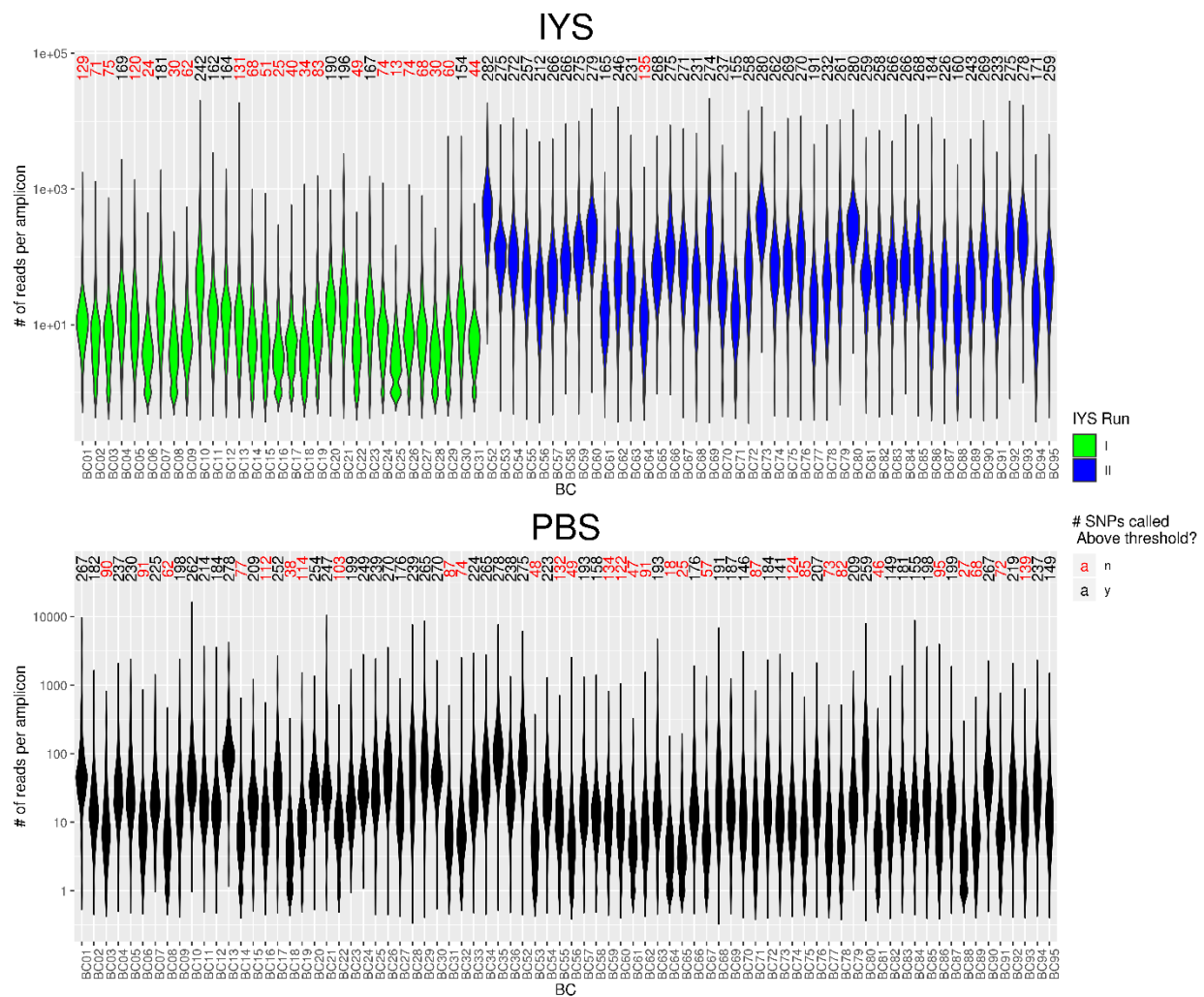
Figure 6: Number of reads per amplicon per individual (barcode) of Nanopore sequencing runs. The violin plot shows the distribution of number of reads assigned to unique SNP-containing amplicons within an individual. Green and blue colors denote the two separate sequencing runs during the IYS expedition (top), and black indicates the run at the laboratory (PBS; bottom). Above each individual violin plot is the total number of amplicons for that individual for which sufficient reads were present to call the genotype, color indicates if enough amplicons were called for downstream analysis (black) or not (red). The order of individuals is matched in the top and bottom plots.
