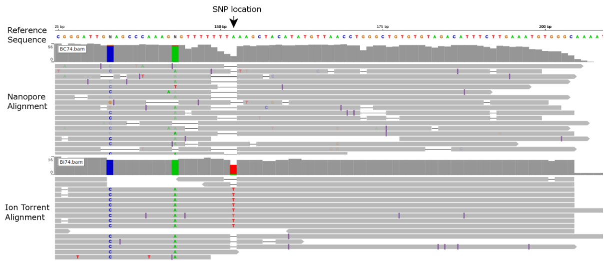
Figure 7: Comparison of sequence alignment of Nanopore and Ion Torrent sequences from the same individual against a SNP locus preceded by a homopolymer tract. Nanopore sequences show a higher number of indels, specifically associated with the poly-T homopolymer tract (145-151bp) directly preceding the SNP location (152bp). Alignment was visualized here using IGV (Robinson et al. 2011)
