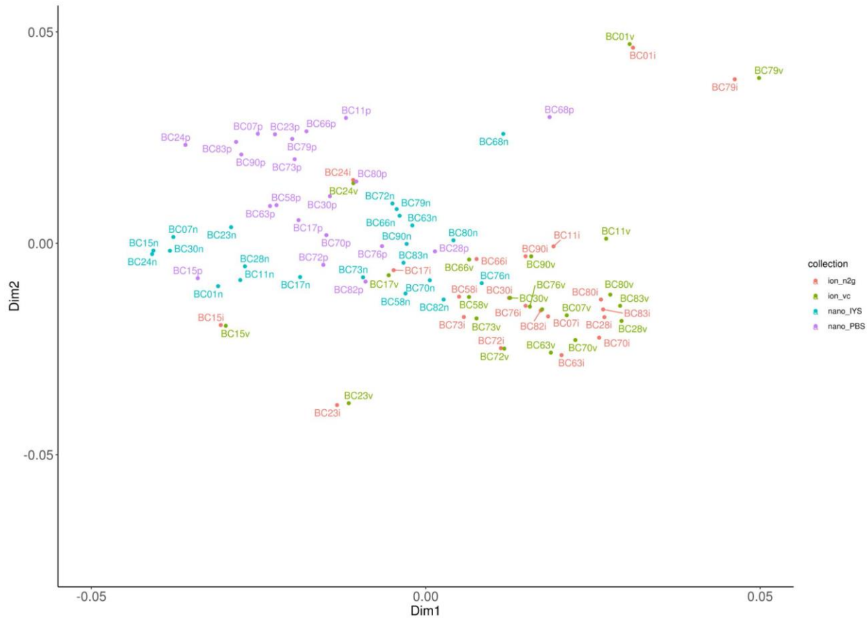
Figure 8: Principal coordinate analysis (PCoA) of SNP calls of individuals passing threshold in all datasets. SNP calls based on Nanopore sequences generated during the IYS expedition shown in blue ("nano_IYS"), and the same individuals reanalyzed upon return using the same workflow shown in purple ("nano_PBS"). Ion Torrent reads scored with the n2g pipeline are shown in red ("ion_n2g") and scores derived from the Ion Torrent variant caller are shown in green ("ion_vc").
