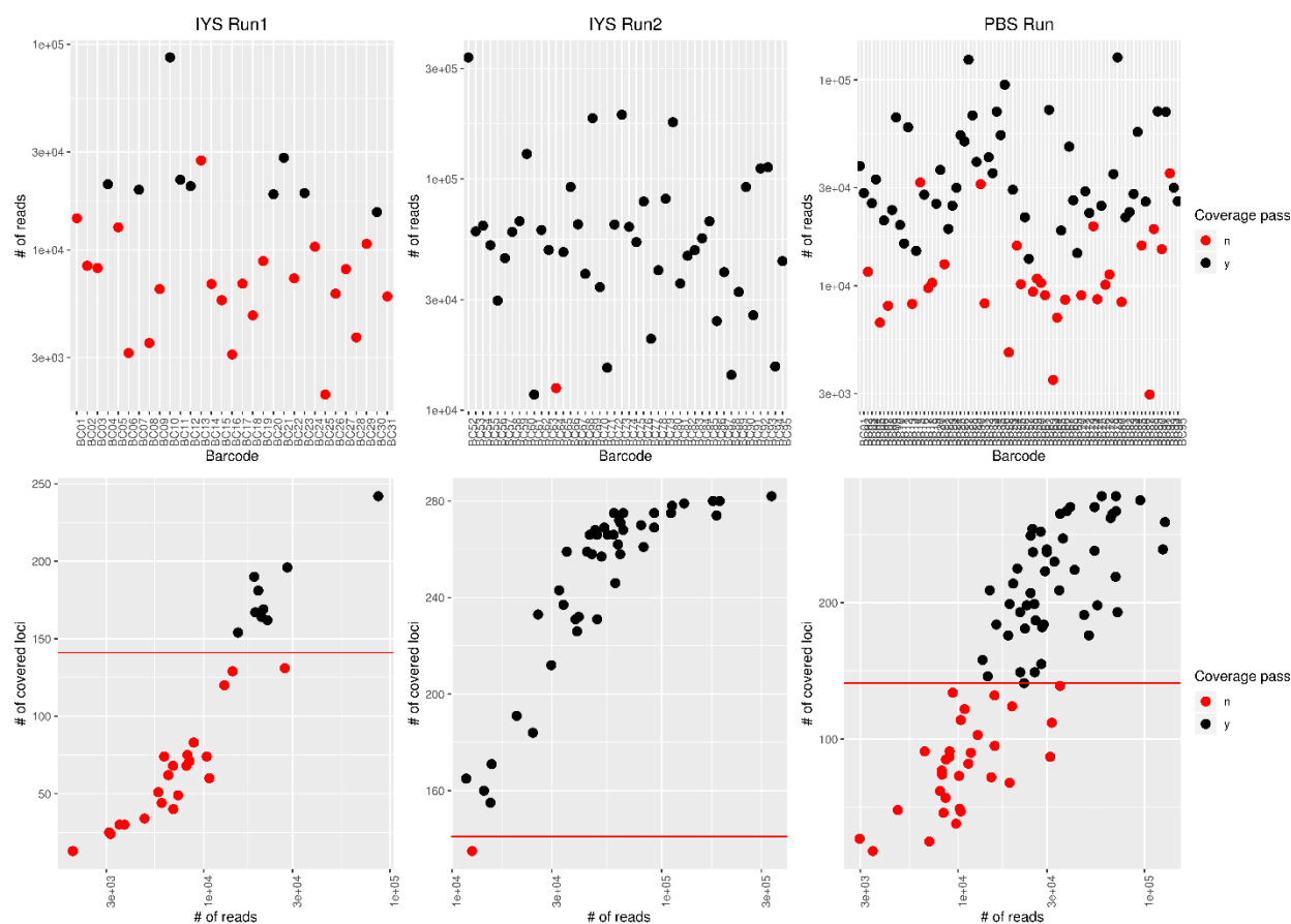
Figure 5: Nanopore sequencing statistics. The top row shows the number of reads binned by individual (barcode). The bottom row shows the number of loci with sufficient read depth ( \geq 10 reads) by the number of reads for each sample. The threshold for downstream analysis was set to 141 loci (50% of loci for this panel) and is indicated in the red line in the second row. Individuals (barcode bins) are coloured according to whether they passed this coverage threshold (black) or not (red).
