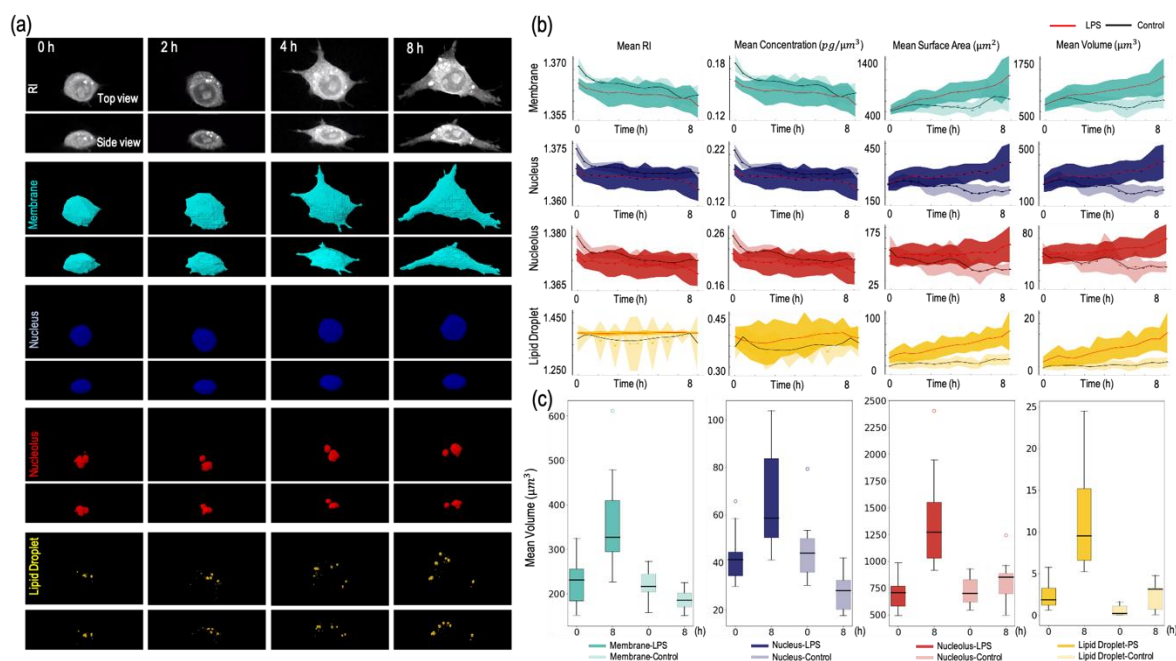
Figure 4. Application to time-lapse imagery of RAW 264.7 cells. (a) Horizontal plane and coronal plane view of RAW 264.7 cells overtime (0, 2, 4, 8 h). Each panel represents the RI tomogram and segmentation masks of the membrane, nucleus, nucleolus, and lipid droplet. (b) The black line and the light shades show the control, LPS-untreated RAW 264.7 cells (n=9), while the red line and the dark shades show LPS-treated, activating RAW 264.7 cells (n=12). The mean RI and mean protein concentration decreased by activation, while mean surface area and mean volume increased during activation. (c) Box plots representing the minimum to maximum and showing all points of the mean volume of subcellular organelles in the RAW 264.7 cells.
