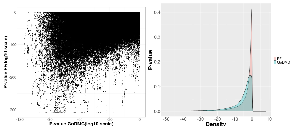
Figure 6: FFCWS meQTL replication in the GoDMC Study. (a) Scatterplot of the log10 p-values found in the FFCWS data versus the log10 p-values found in the GoDMC data from CpG-SNP pairs in common between the two studies. (b) Density plot of the p-values found in the FFCWS data on log10 scale (pink) and the p-values found in the GoDMC data (in blue) from CpG-SNP pairs in common between the two studies.
