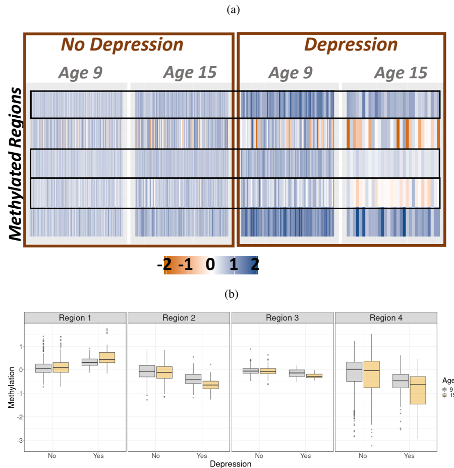
Figure 2: Interactions between age and depression for differential methylation. Residualized M-values are computed by removing the effects of the associated covariates that are not the phenotypes of interest. For visual purposes, we stratify the depression scores by those less than or equal to six versus those greater than six. (a) Heatmap of the methylation levels in DMRs for age-depression interactions (Table 2b). Methylation levels are quantified as residualized M-values. (b) Boxplots of the four highlighted DMRs (numbers 1, 5, 10, and 14 in Table 2b) as examples of differential methylation at these regions between ages 9 and 15 among one of the categories (depression or no depression) with no evidence of differential methylation among the other category. These regions show an interaction effect between age and depression on methylation.
