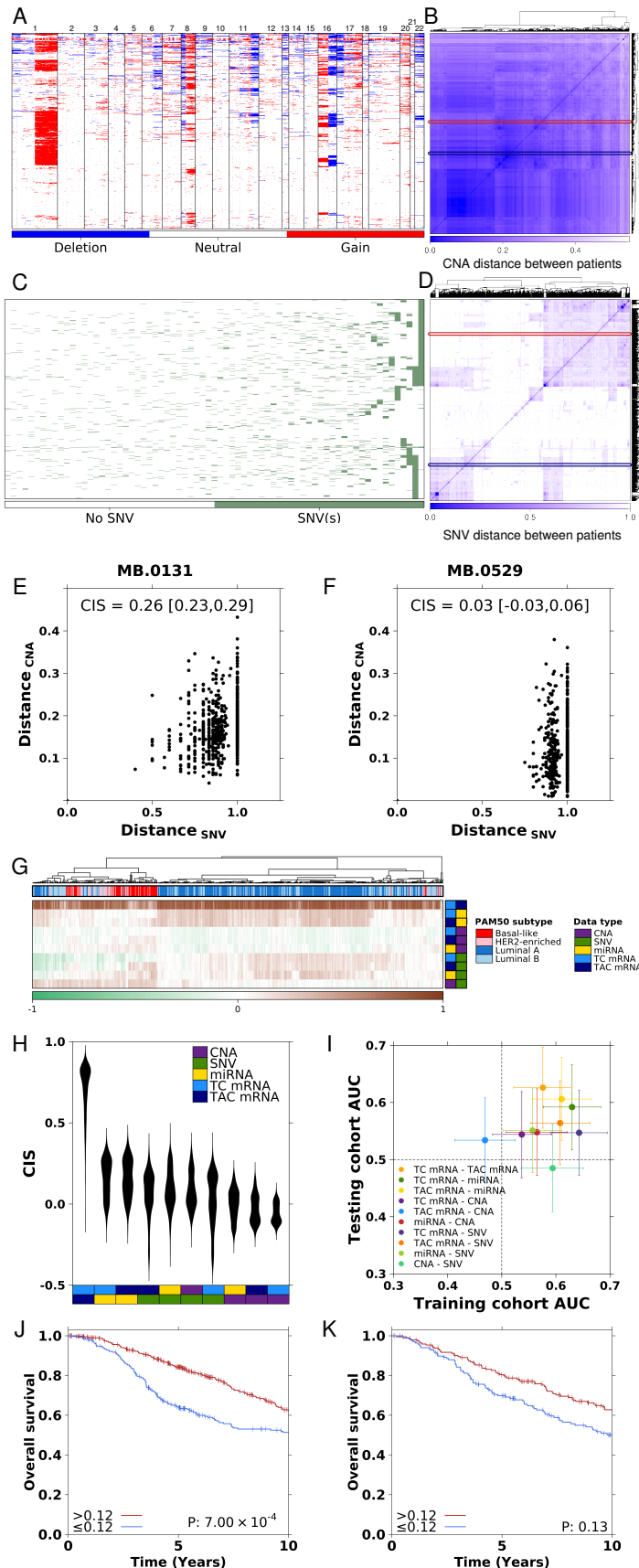
Figure 1 | Integrative similarities.
