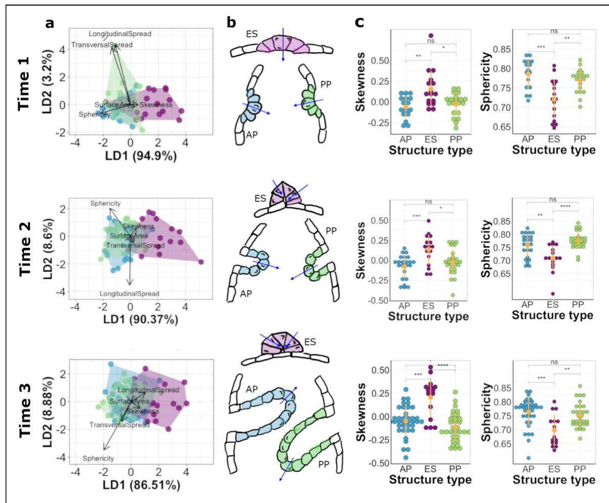
Fig 3.: Comparison of shape dynamics in developing structures of the zebrafish inner ear. Rows represent each time point analysed. Data in blue represent cells from AP, green represent cells from PP and magenta represent ES. a. Linear discriminate analysis (LDA) biplots illustrate multivariate clustering of data – data from AP and PP show considerable overlap indicating similar shape signatures while data from ES show less overlap with the former. b. Schematic illustrations of cell shape signatures at the time points analysed showing cells in the ES having skew in the opposite direction to those in the projections and having less rounded shapes. Arrows indicate apico-basal polarity. c. Plots showing differences in skewness and sphericity between the structures at the time points analysed. Yellow dots with error lines represent mean and standard deviation for the data. p values for paired comparisons depicted are from Table 1.
