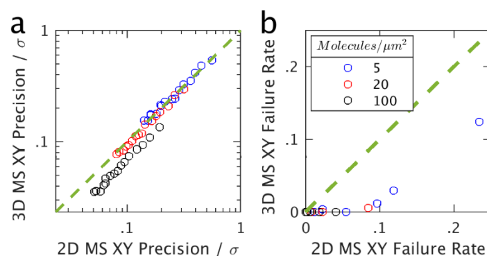
Supplementary Figure 6. 2D projections of 3D data degrade mean shift (MS) shift estimation performance. Lateral (x-y) precision (a) and failure rate (b) when MS shift is determined in 3D or in 2D after projecting the localizations into the x-y plane.
