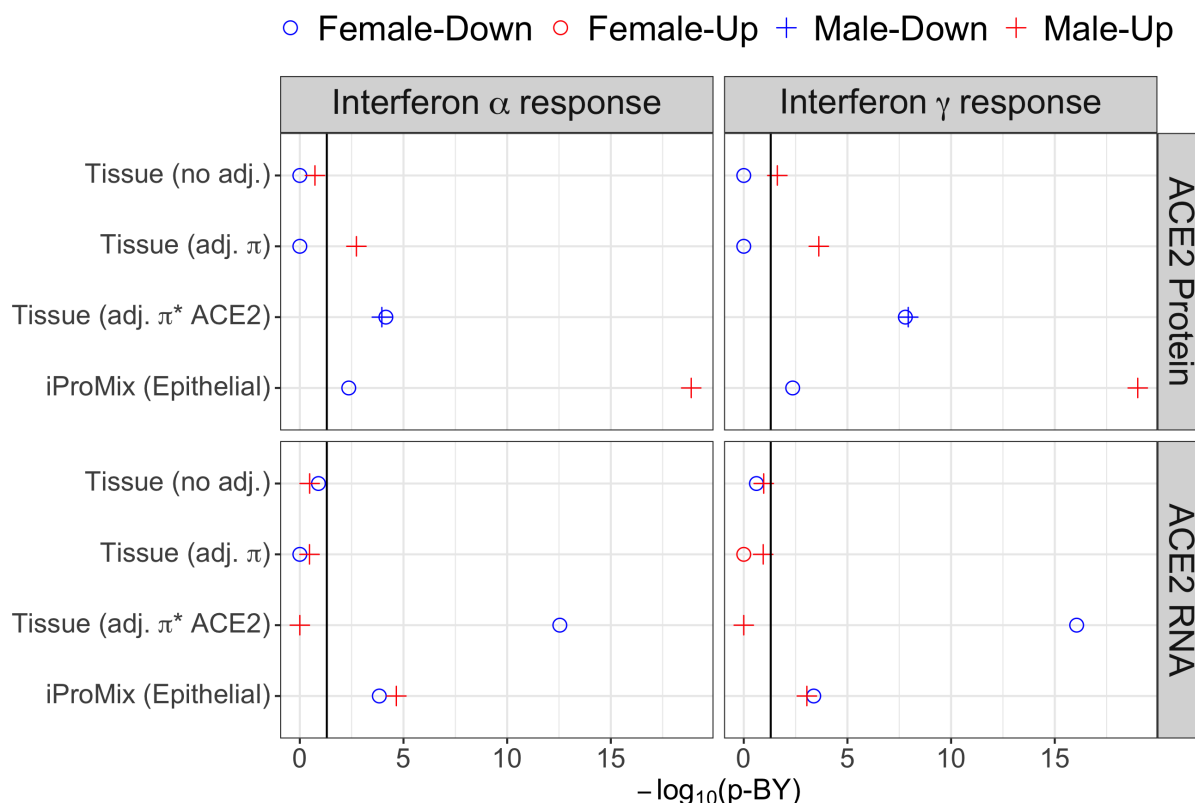
Figure 4: Pathway enrichment results for IFN \gamma and IFN \alpha pathways using tissue-level models and iProMix for men and women. Sex differences in immune responses was observed. Both IFN \gamma and IFN \alpha pathways were significantly positively associated with both ACE2 expression and protein levels in epithelial cell component in men. These two pathways were negatively associated with ACE2 expression and protein levels in epithelial cell component in women.
