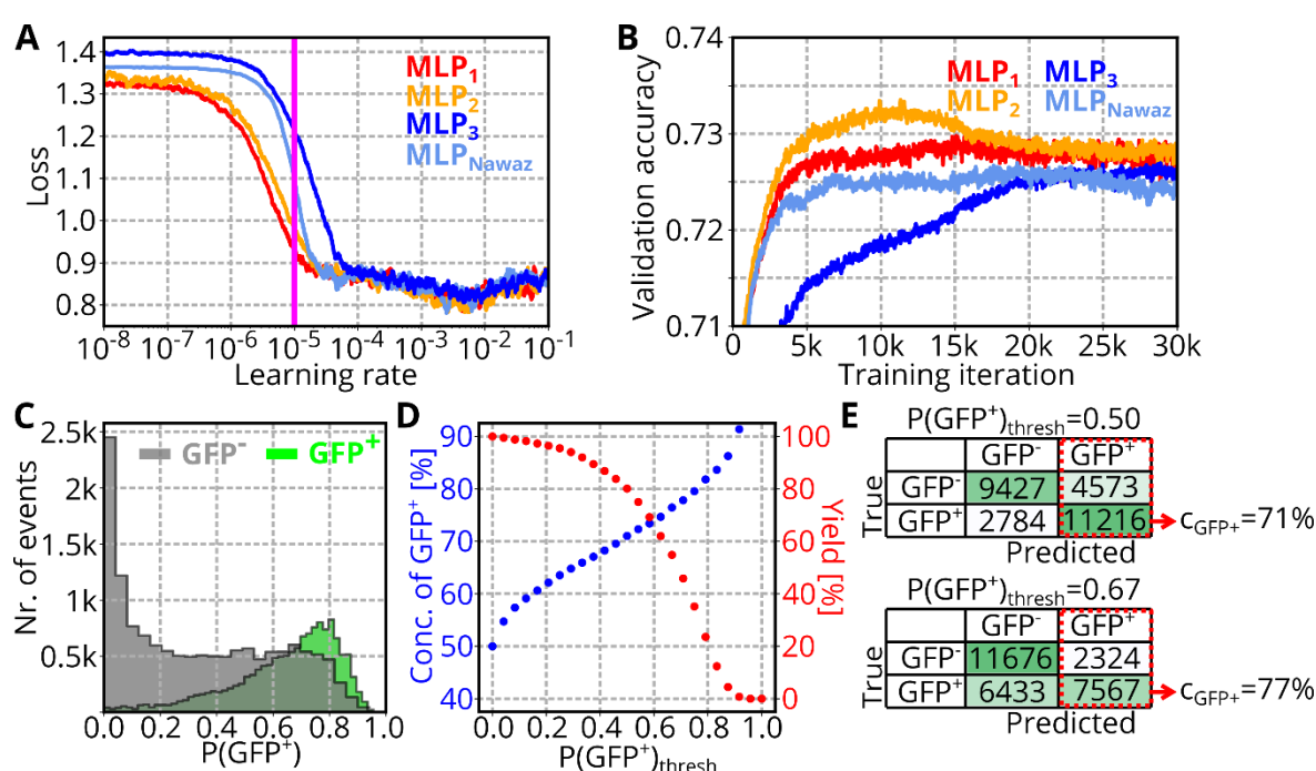
Figure 6: MLP training and assessment
