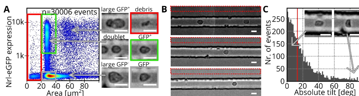
Figure 5: Dataset assembly
