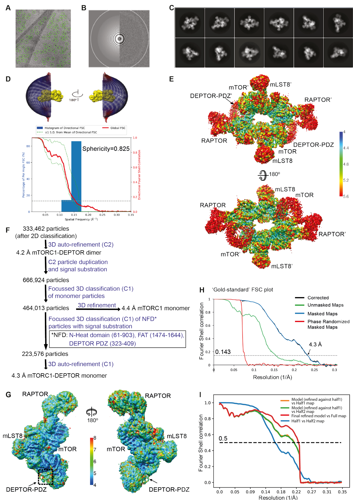
Figure 3-figure supplement 2. Cryo-EM data of the mTORC1/DEPTOR complex.
