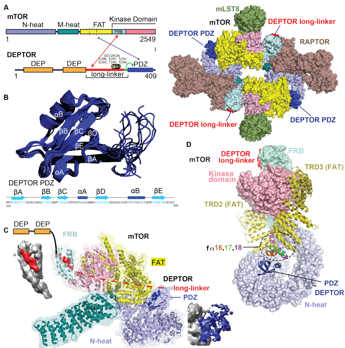
Figure 3. Cryo-EM structure of mTORC1/DEPTOR reveals bipartite binding mode of DEPTOR linker-PDZ to mTOR.
