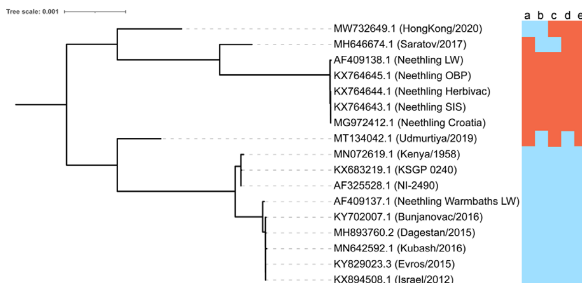
Figure 3. Core gene phylogenetic tree. The phylogenetic tree was built using the core genes (including intergenic regions between consecutive core genes) using RAxML and midpoint rooted. For accessory genes, isolates that grouped with either vaccine strains or wildtype strains in the network analysis are highlighted with red and blue respectively (panel on right). Different patterns of grouping are seen for 39 accessory genes: a) LD006, LD007, LD143, LD148, b) LD030, LD133, LD144, LD145, LD147, c) LD009, LD135, LD136, LD137, LD138, d) LD015, LD017, LD034, LD035, LD127, LD141, LD142, LD146, LD150, LD151, e) LD008, LD010, LD018, LD020, LD021, LD023, LD066, LD067, LD122, LD125, LD126, LD128, LD129, LD130, LD152.
