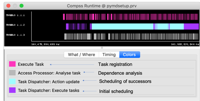
Fig. 8. Paraver timeline view of the runtime behaviour
