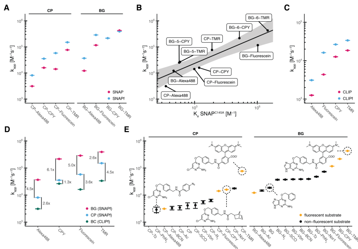
Figure 4: Characterization of SNAP- and CLIP-tag labeling kinetics.
