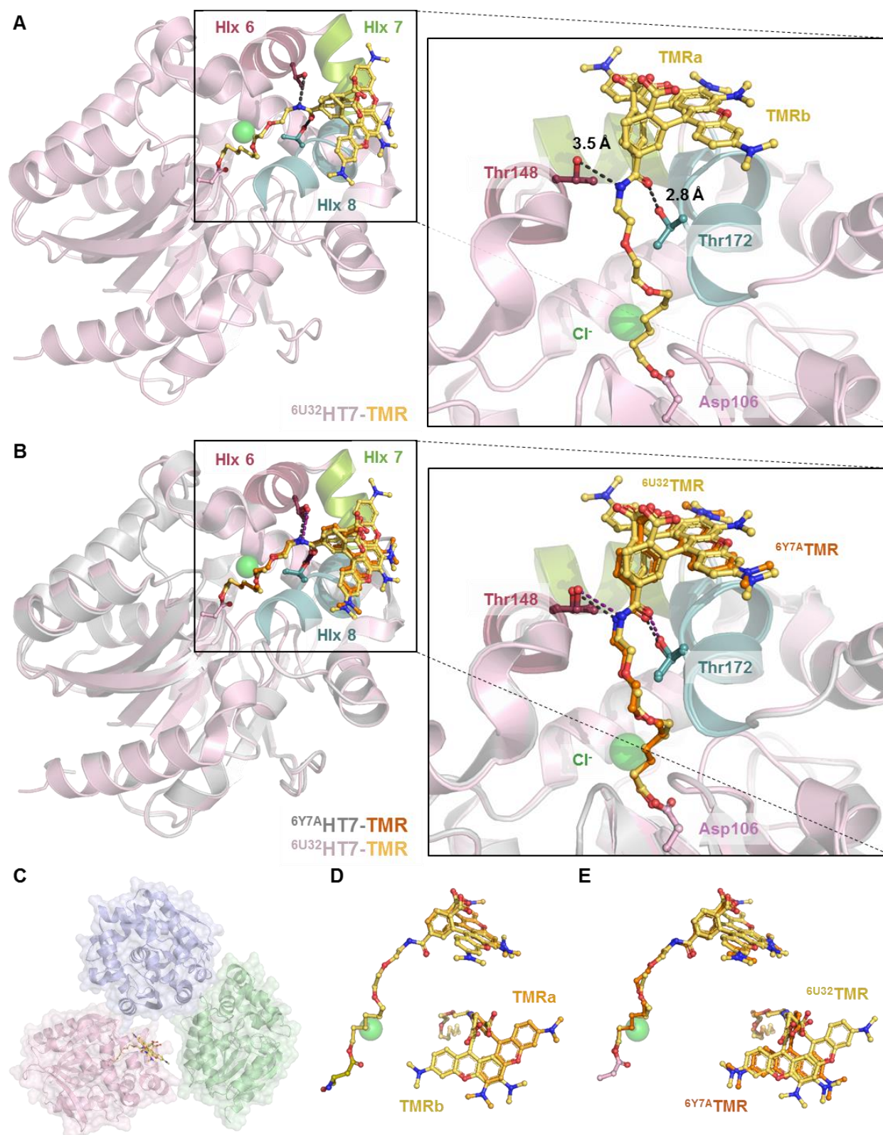
Figure S10: Structural comparison between HT7-TMR structures from PDB IDs 6U32 and 6Y7A.
