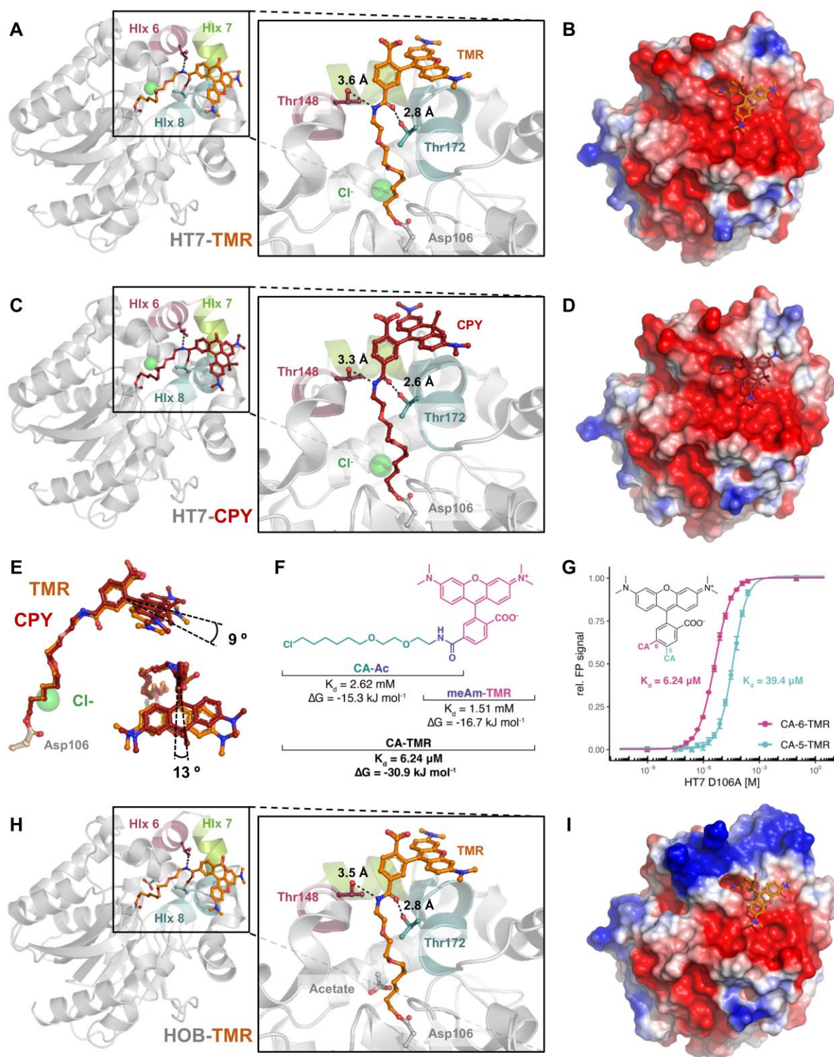
Figure 3: Structure-function analysis of HaloTag7 substrate interactions.
