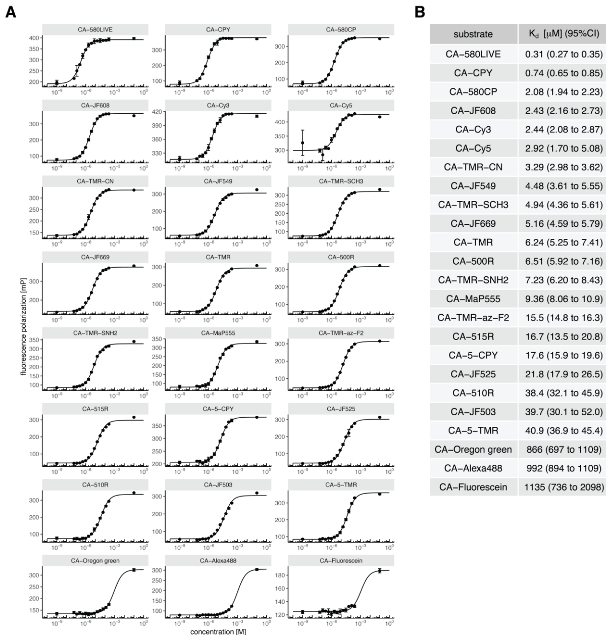
Figure S7: Affinity of the dead mutant HT7 D106A to fluorescent CA substrates.
