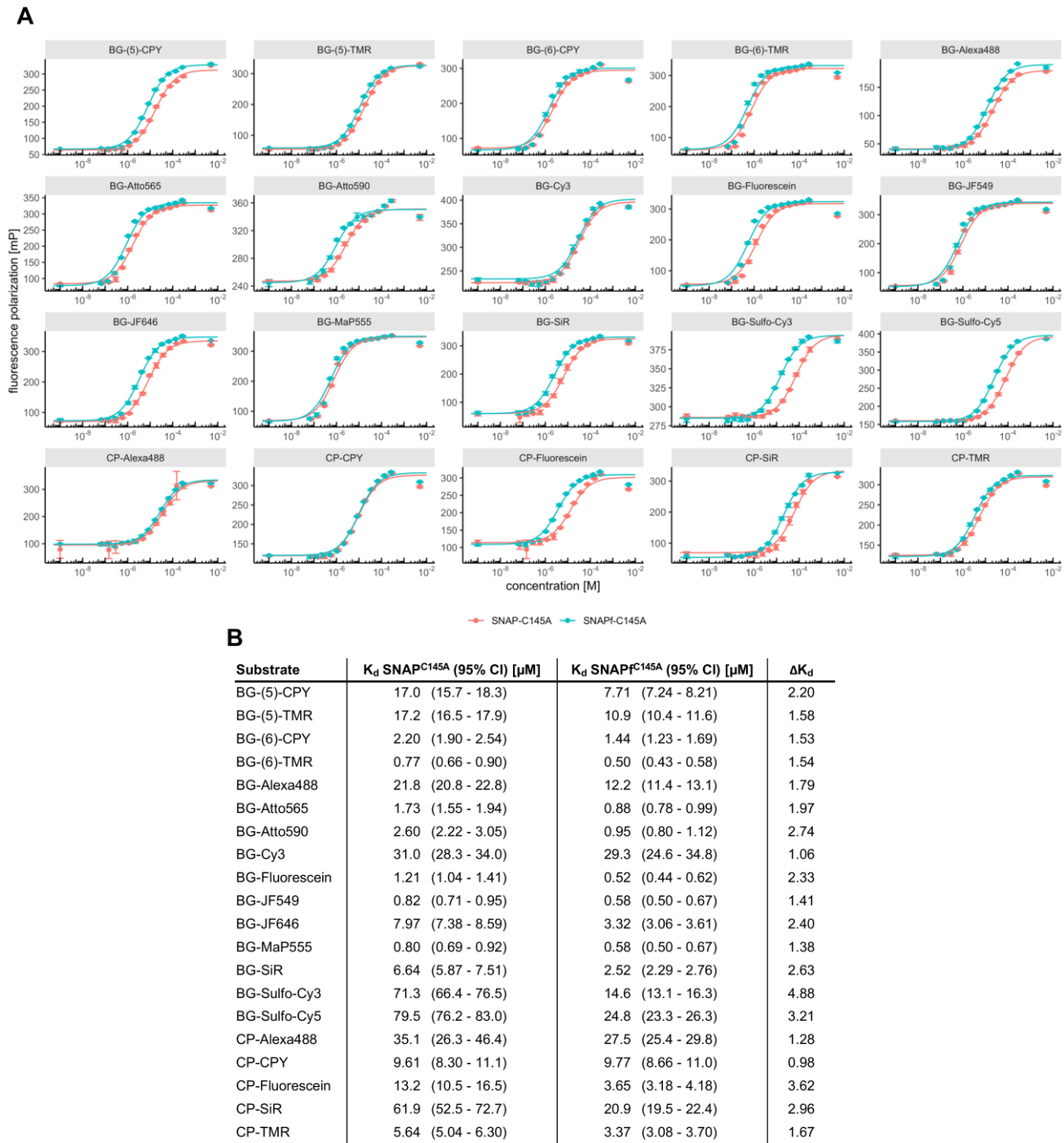
Figure S15: Comparison of fluorophore substrate affinities between the dead mutants SNAP C145A and SNAPf C145A .
