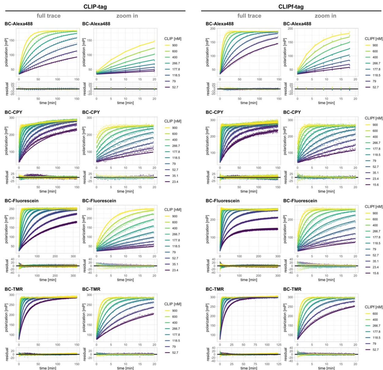
Figure S19: Labeling kinetics of CLIP and CLIPf with fluorescent BC substrates.
