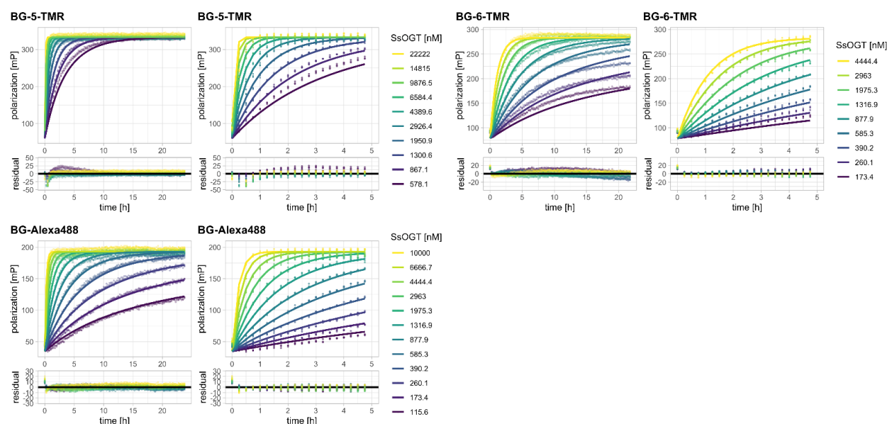
Figure S26: Labeling kinetics of SsOGT-H 5 with BG-Alexa488 and BG-TMR.
