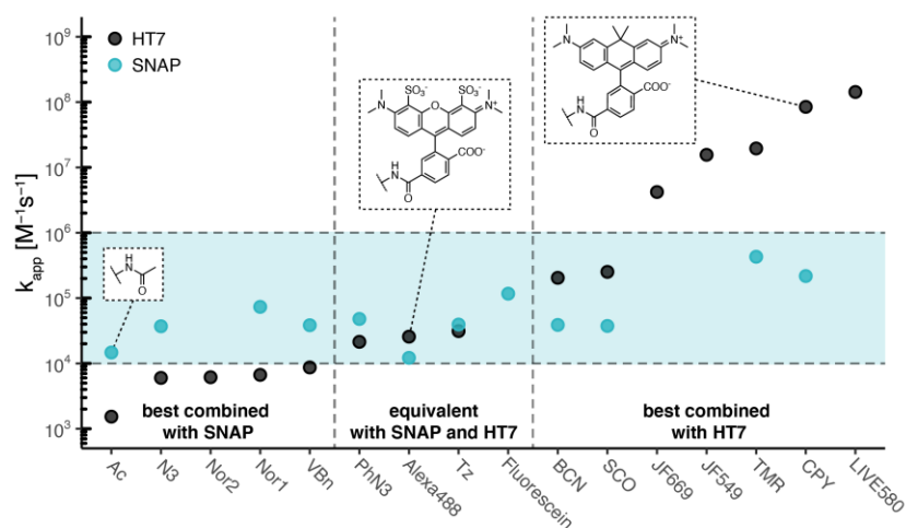
Figure 6: Labeling kinetics comparison between SNAP-tag and HaloTag7.
