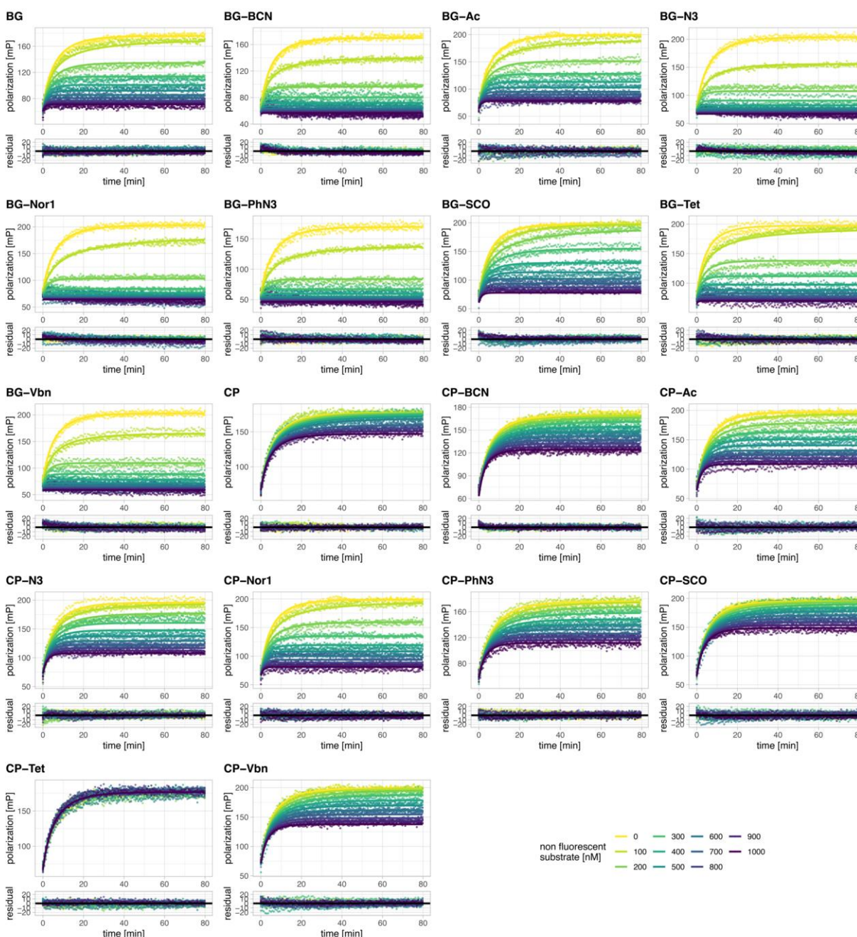
Figure S21: Labeling kinetics of SNAP with non-fluorescent BG and CP substrates.
