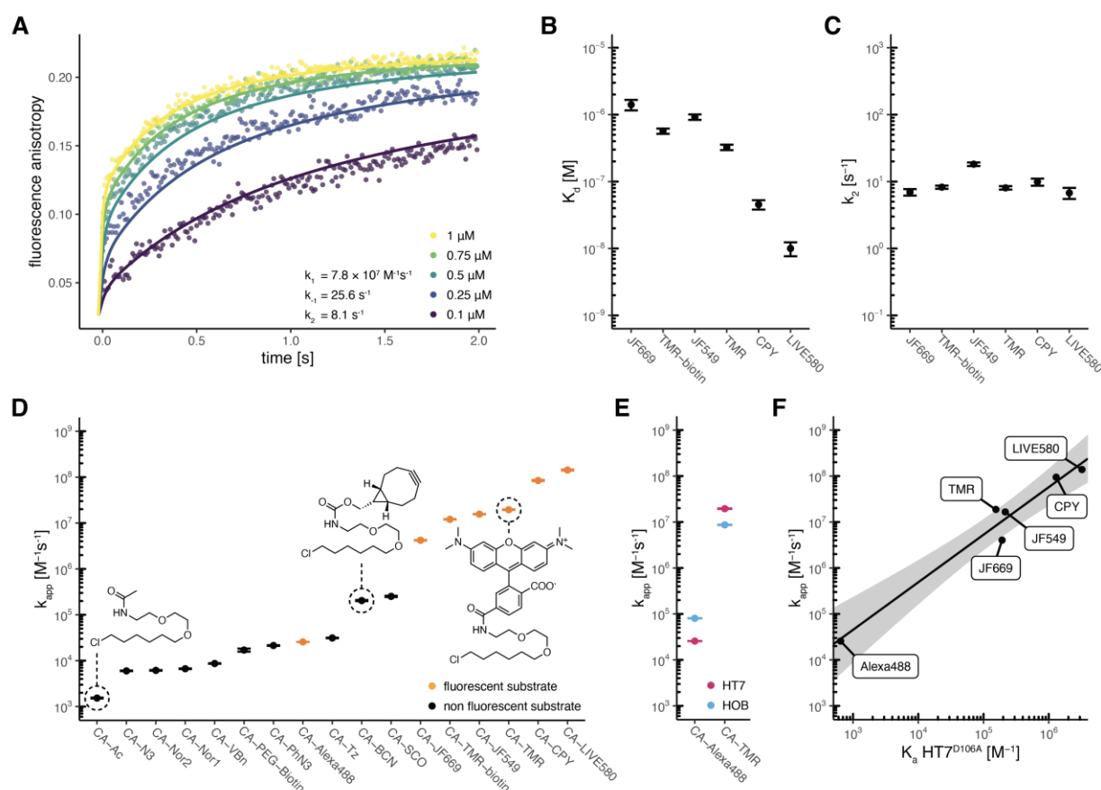
Figure 2: Characterization of HaloTag7 labeling kinetics.
