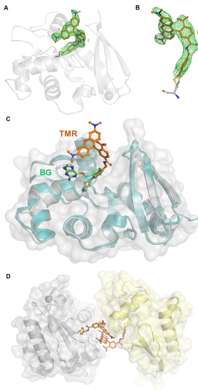
Figure S22: Validation and analysis of the SNAP-TMR X-ray structure.
