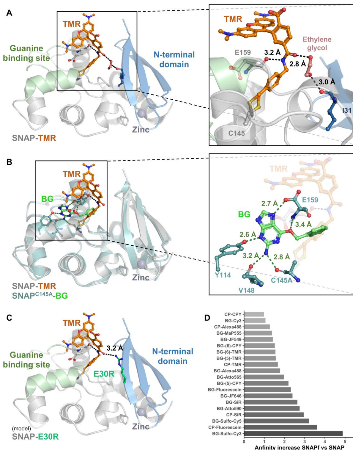
Figure 5: Structure-function analysis of SNAP-tag fluorophore substrate interactions.
