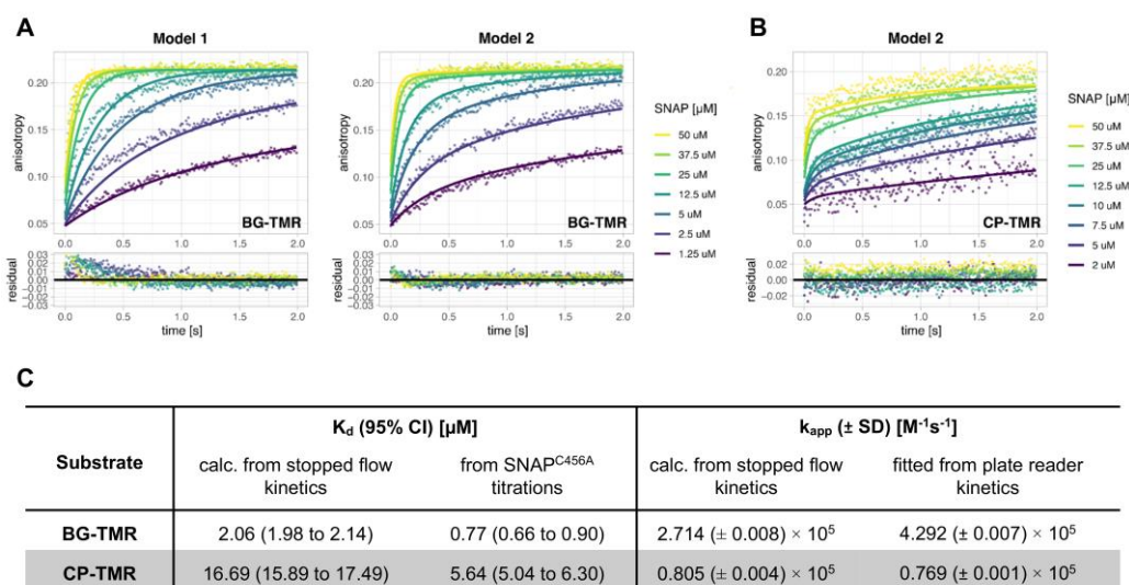
Figure S14: Labeling kinetics of SNAP measured by stopped flow fluorescence anisotropy.
