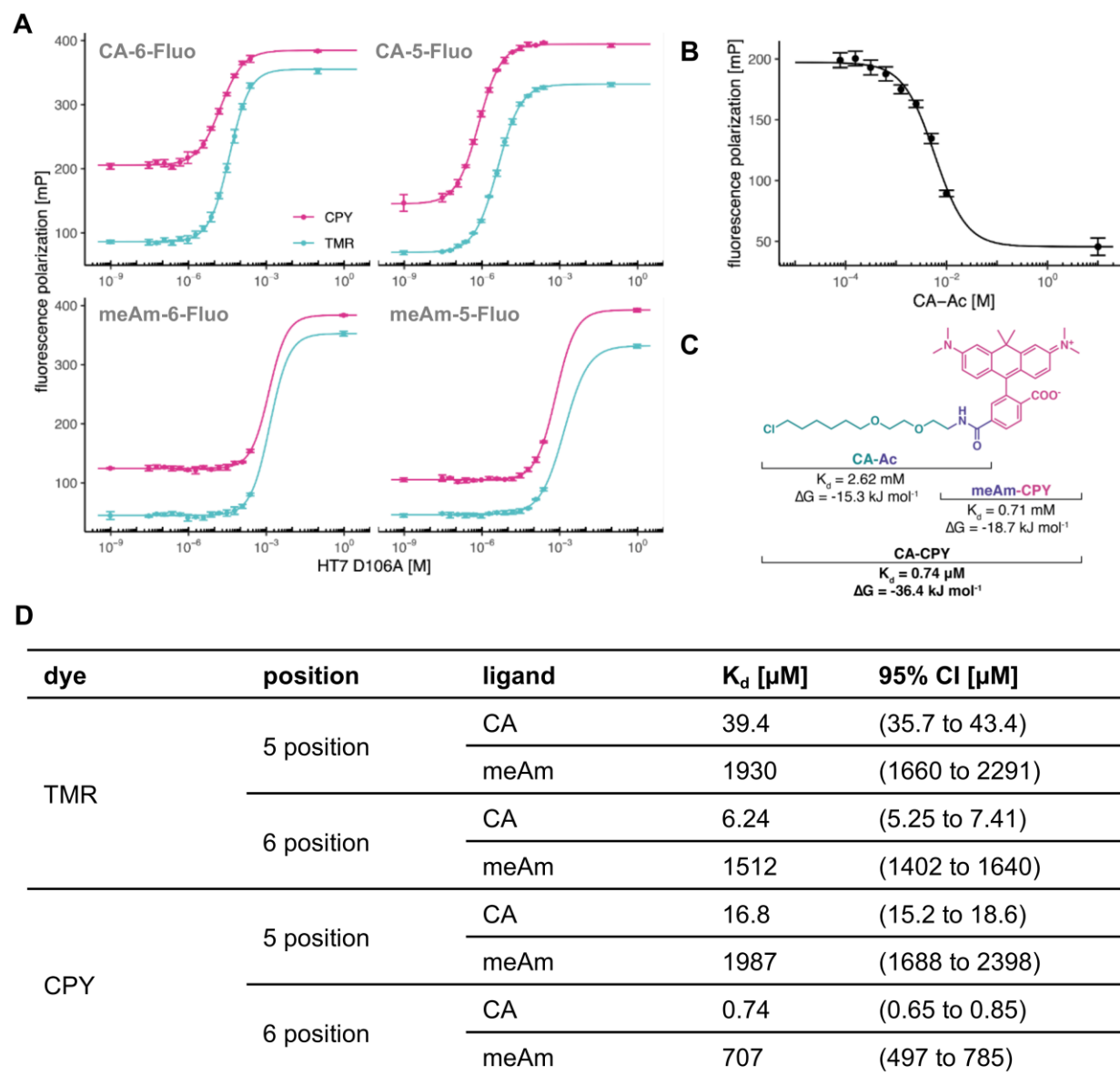
Figure S12: Biochemical study of the interaction of HT7 with CA-fluorophores.
