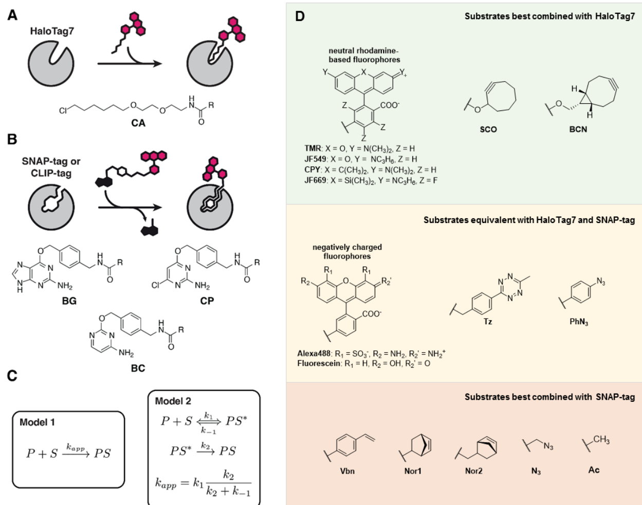
Figure 1: Self-labeling reaction, substrates and kinetic models.
