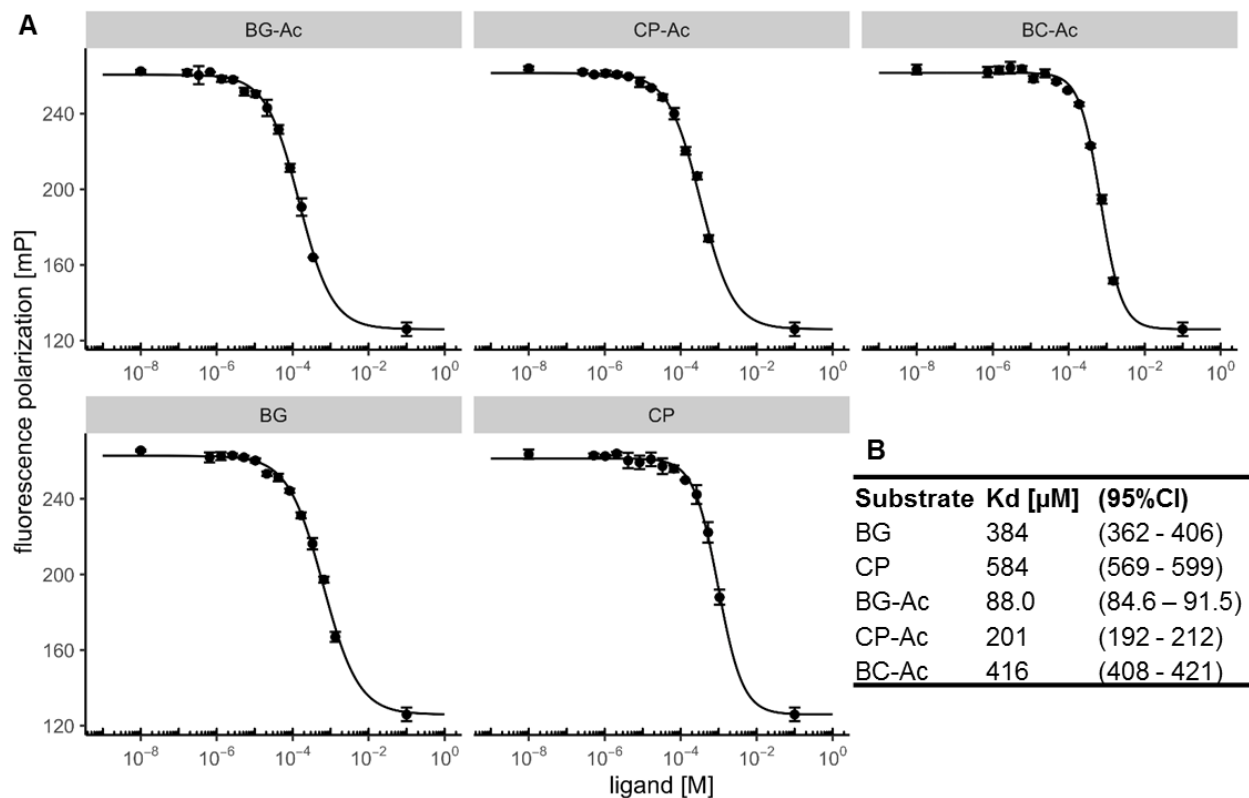
Figure S16: Comparison of non-derivatized core substrate affinities with the dead mutant SNAP C145 . A. Titration curves obtained for the dead mutant SNAP C145A measured via competitive fluorescence polarization. The FP value of free dye was added at c = 0.1 M to improve fitting of the lower plateau. (See corresponding methods section for more details) B. Table summarizing fitted K d values with 95% confidence intervals. For structures of substrates see Fig. S1 .
