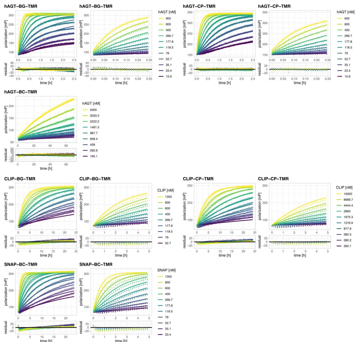
Figure S20: Labeling kinetics of hAGT, SNAP and CLIP with the non-respective BG-, CP- and BC-TMR substrates.
