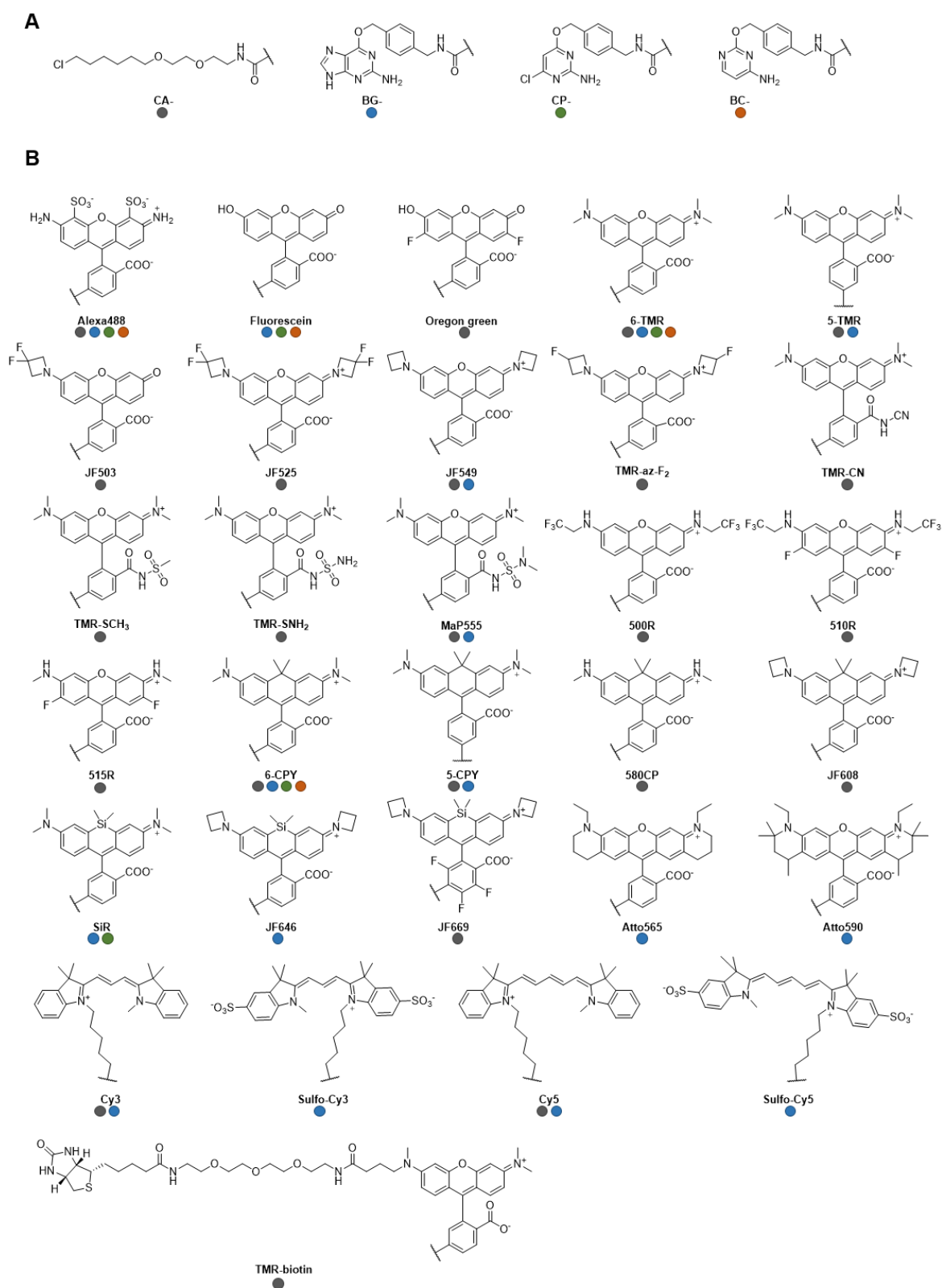
Figure S1: Chemical structures of SLP substrates. (continued on the next page)
