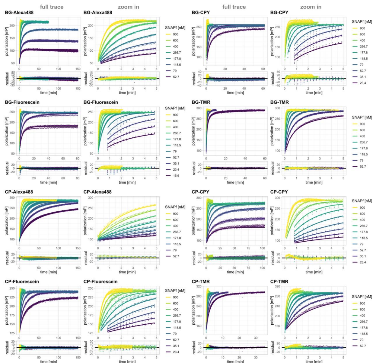
Figure S18: Labeling kinetics of SNAPf with fluorescent BG and CP substrates.
