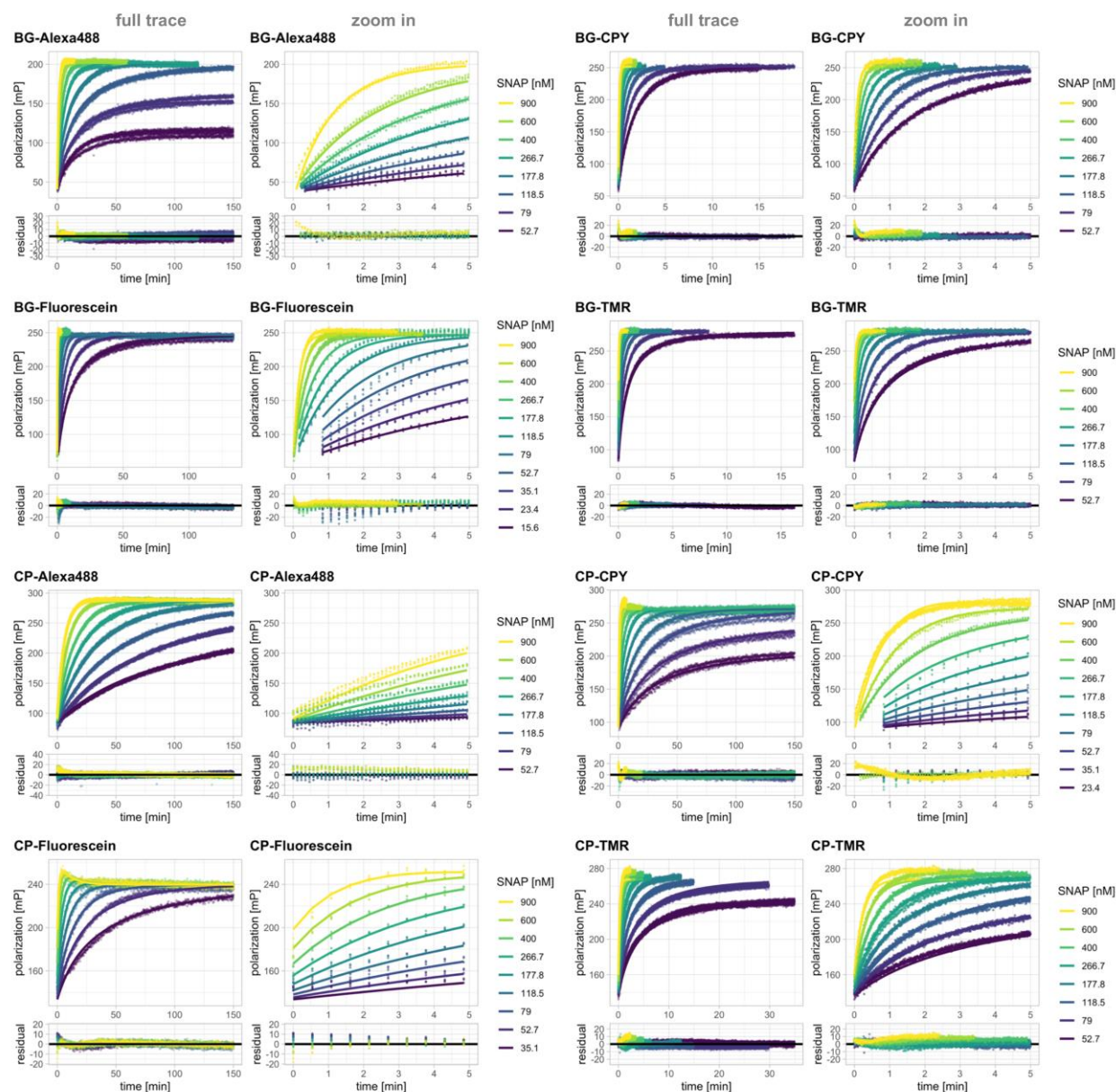
Figure S13: Labeling kinetics of SNAP with fluorescent BG and CP substrates.
