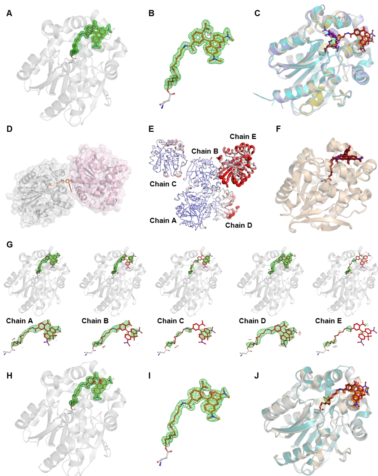
Figure S9: Validation of HT7-TMR and HT7-CPY X-ray structures.
