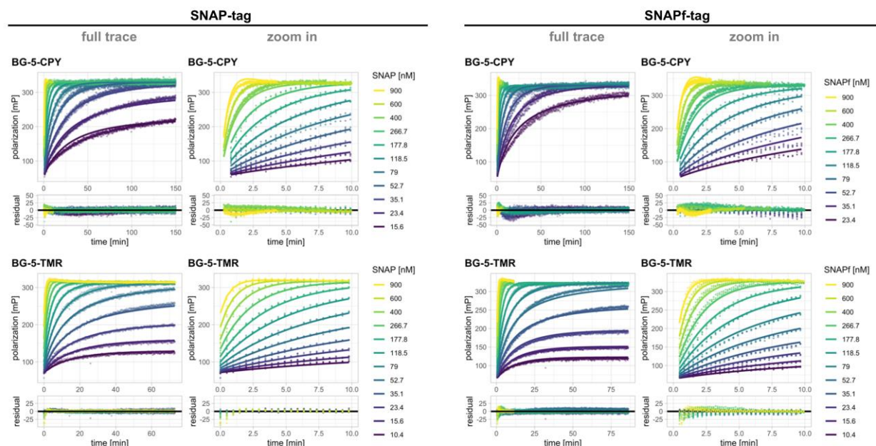
Figure S23: Labeling kinetics of SNAP and SNAPf with BG-5-TMR and BG-5-CPY.
