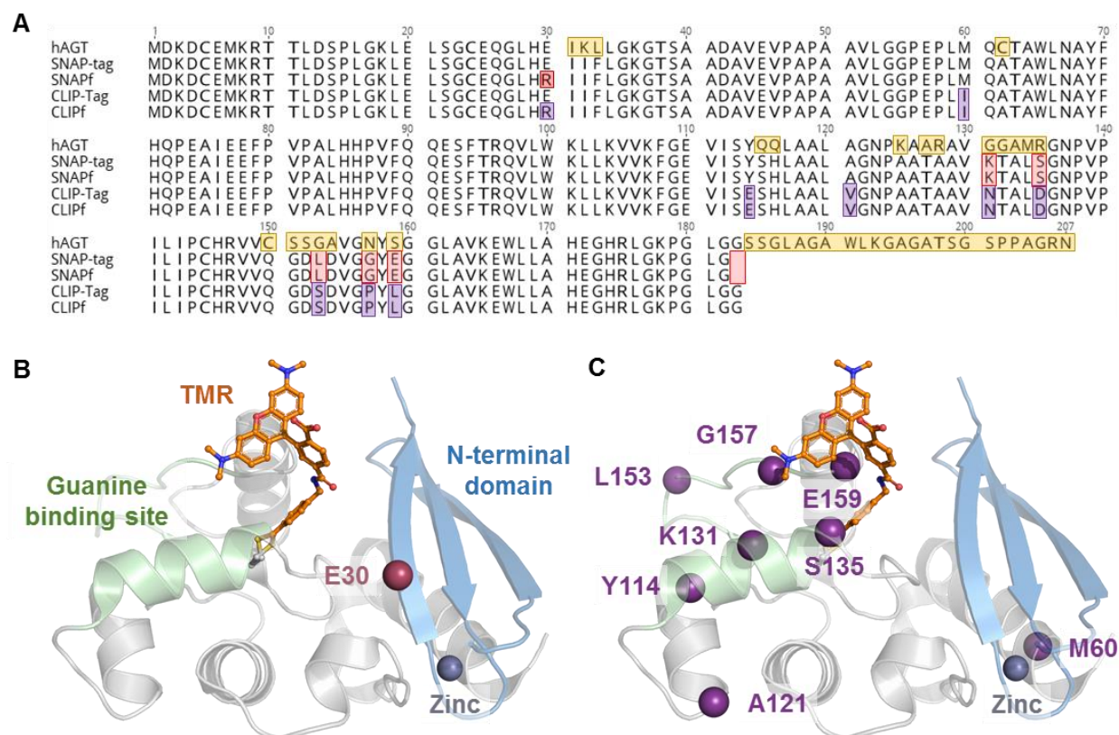
Figure S17: Sequence alignment and structural comparison between SNAP and CLIP variants.
