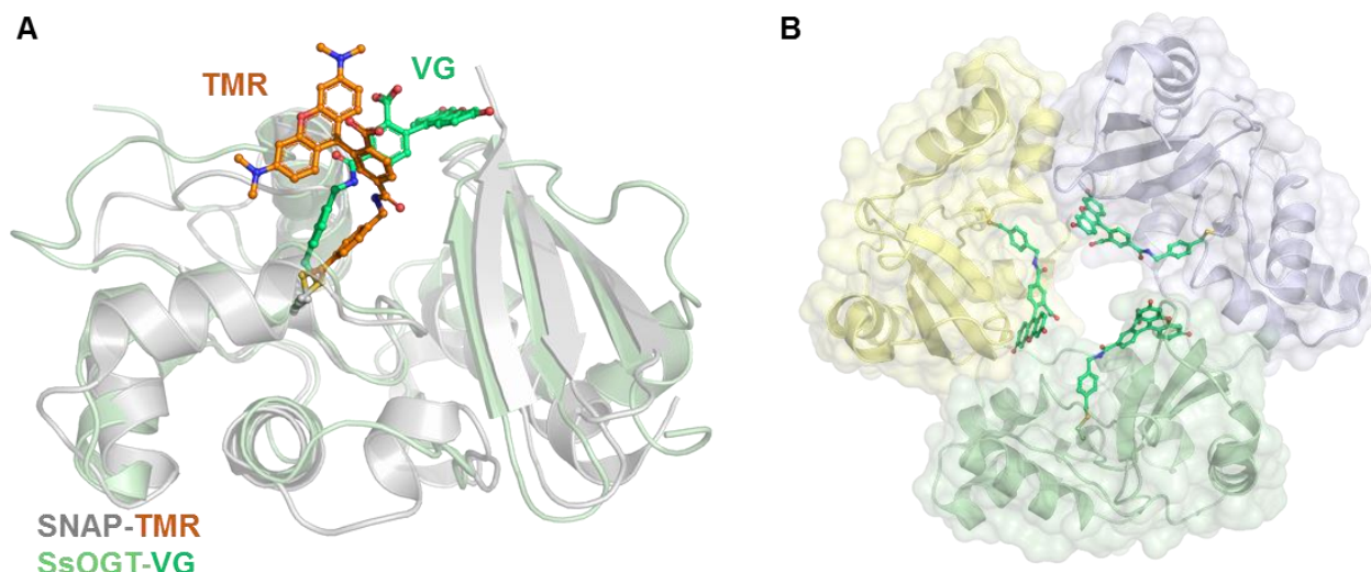
Figure S25: SsOGT-H 5 -VistaGreen alternative fluorophore conformation.
