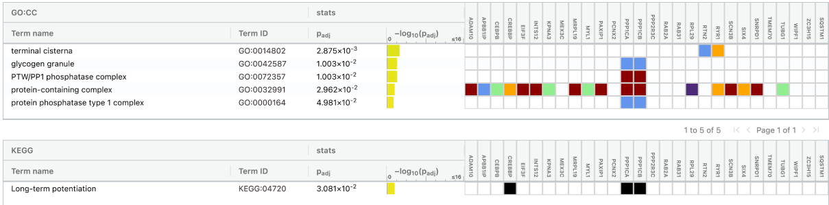
Supplement Figure 1b: g:profiler gene set enrichment analysis of genes listed in Table 3.
