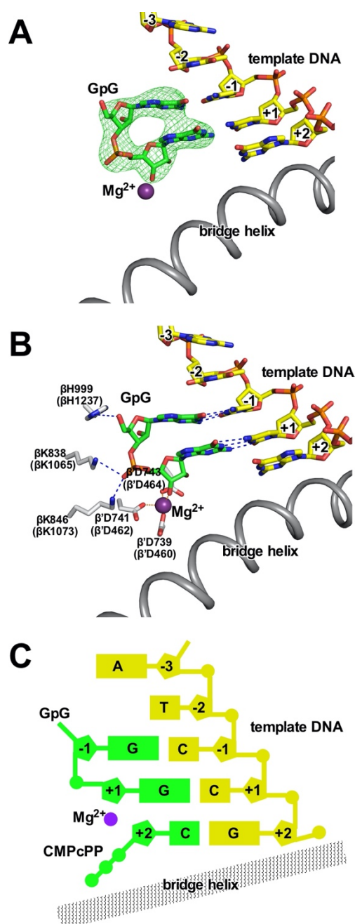
Figure S7. Structural basis of promoter-sequence dependence of primer-dependent initiation at position TSS-2
