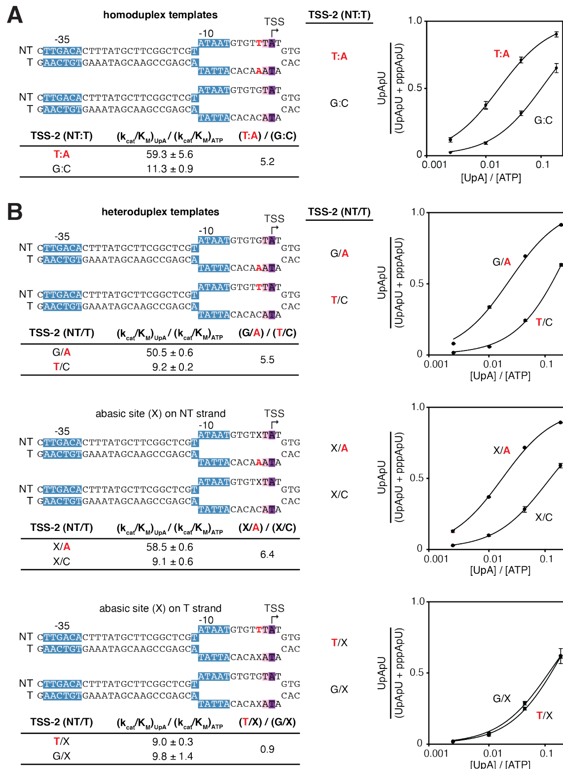
Figure 5. Promoter-sequence dependence of primer-dependent initiation in vitro : position TSS-2. A. Relative efficiencies of primer-dependent initiation vs. primer-independent initiation depends on promoter sequence at position TSS-2. Top left: homoduplex DNA templates containing consensus or
