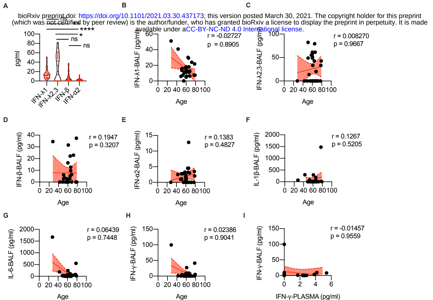
SUPPLEMENTARY FIGURE 2. (A) Protein levels of IFN-λ1, IFN-λ2,3, IFN-β, IFN-α2 measured in the BALF of COVID-19 patients. Each dot represents a patient. Violin plots are depicted. (B-H) IFN-λ1 (B), IFN-λ2,3 (C), IFN-β (D), IFN-α2 (E), IL-1β (F), IL-6 (G) and IFN-γ (H) protein levels in the BALF of COVID-19 patients are plotted over age. (I) IFN-γ protein levels in the BALF are plotted against protein levels in the plasma of each COVID-19 patient. (B-I) Each dot represents a patient. Linear regression lines (continuous line) and 95% confidence interval (dashed line and shaded area) are depicted in red. Spearman correlation coefficients ( r ) and p -value ( p ) are indicated. Statistics: (A) Kruskal-Wallis test with Dunn's post-hoc test: ns, not significant ( P > 0.05 ); * P < 0.05 , ** P < 0.01 , *** P < 0.001 , and **** P < 0.0001 .
