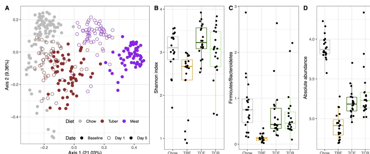
Figure 5: SparseDOSSA correctly models the effects of diet and time on the murine gut microbiome by reproducing effects from amplicon sequencing profiles. A) SparseDOSSA 2 was fitted to subsets of samples from [23] that included up to three time points each from collections of mice fed chow, raw or cooked tubers, and meat. The resulting models were then used to simulate controlled microbial community profiles, which correctly reproduced the beta-diversity structures present in the original study (MDS ordination by Bray-Curtis dissimilarities). The SparseDOSSA model was also able to model and synthetically replicate changes in "Bacteroidetes" and "Firmicutes" phyla in response to raw vs. cooked diets, including B) overall community alpha-diversity (Shannon index), C) the resulting "Firmicutes" vs. "Bacteroidetes" ratio, and D) overall whole-community effective biomass. TRF = raw tuber (free-fed); TCF = cooked tuber (free-fed); TCR = cooked tuber (restricted ration).
