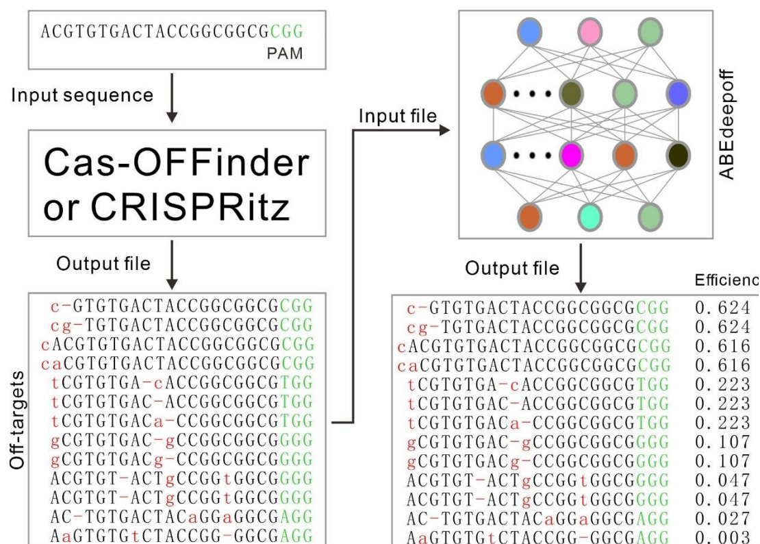
Figure 3. Example of ABEddeepoff for off-target identification.
