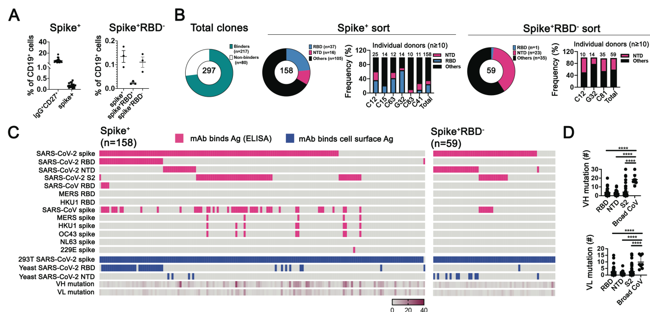
Fig. 1. SARS-CoV-2 surface glycoprotein (spike) specificities of memory B cells from convalescent subjects. (A) Cells recovered from two sorting strategies, shown in dot plots as percentages of total CD19 + cells. Left: IgG + CD27 + cells from 18 donors (one dot per donor) and the subset of those that expressed spike-binding BCRs. Right: cells from 3 donors expressing spike-binding BCRs and sorted to recover principally those that did not bind recombinant receptor-binding domain (RBD). Sorting protocols as described in Methods and shown in Fig. S1. (B) Summary of all antibodies (expressed as recombinant IgG1) screened by ELISA (with recombinant spike ectodomain trimer) and cell-surface expression assays (both 293T and yeast cells). Total numbers in the center of each of pie chart; numbers and color codes for the indicated populations shown to next to each chart. To the right of the charts for the two alternative sorting strategies are bar graphs showing frequencies of SARS-CoV-2 RBD and NTD binding antibodies for those subjects from whom at least 10 paired-chain BCR sequences were recovered. (C) Binding to a panel of spike proteins and SARS-CoV-2 subdomains, listed on the left, as determined by both ELISA (with recombinant spike ectodomain) and by association with spike expressed on the surface of 293T cells or with RBD or NTD expressed on the surface of yeast cells, for cells sorted just for spike binding (left) and for those sorted for positive spike binding but no RBD binding (right). The rows with pink highlighting are from the ELISA screen; those with blue highlighting, from the cell-based screens. Each short section of a row represents an antibody. The rows labeled VH mutation and VL mutation are heat maps of counts (excluding CDR3) from alignment by IgBLAST, with the scale indicated. (D) Dot plots of heavy- and light-chain somatic
