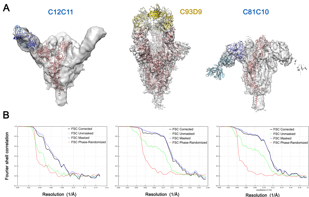
Fig. S8. Low- and moderate-resolution structures for C12C11, C93D9 and C81C10 complexes.
