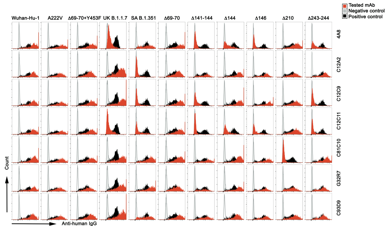
Fig. S12. Representative flow plots for mAb binding to the indicated variants. Flow plots for binding of 7 mAbs to Nextstrain cluster 20A.EU1 (A222V), Danish mink variant ( \Delta 69-70 and Y453F), UK B.1.1.7 ( \Delta 69-70, \Delta 144, N501Y, A570D, P681H, T716I, S982A, D1118H) and SA B.1.351 (L18F, D80A, D215G, \Delta 241-243, K417N, E484K, N501Y, A701V) and NTD deletion variants. Plasmids with variant S co-expressed with pmaxGFP in HEK 293T cells. Cells were gated on DAPI - GFP + . mAb C81E2 was used as positive control, and PBS, as negative control.
