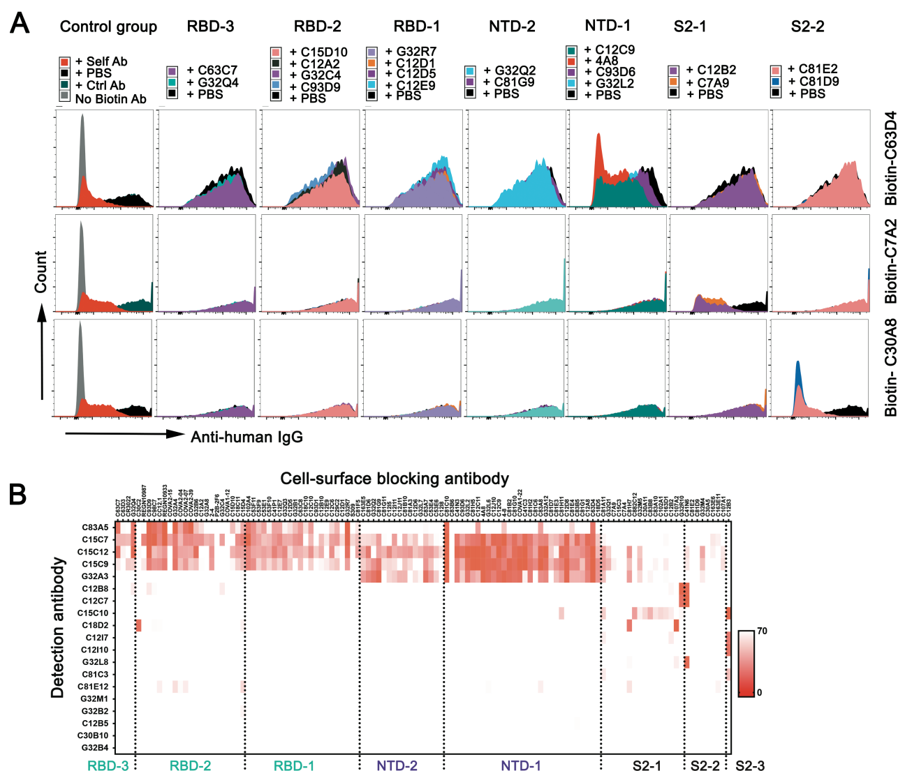
Fig. S4. Cell-based competition assay. (A) Representative flows plot for competition, by 20 blocking antibodies representing each of the seven principal clusters (from ELISA: Fig. 2A), for binding cell-surface expressed spike protein by 3 biotinylated antibodies. A non-COVID-19 related antibody and a self-blocking antibody were used as negative and positive controls. (B) Heat map of 19 mAbs with hierarchical clustering from cell-based competition assay with 118 blocking antibodies. See Fig. 2B for procedures, heat-map color scheme, etc.
