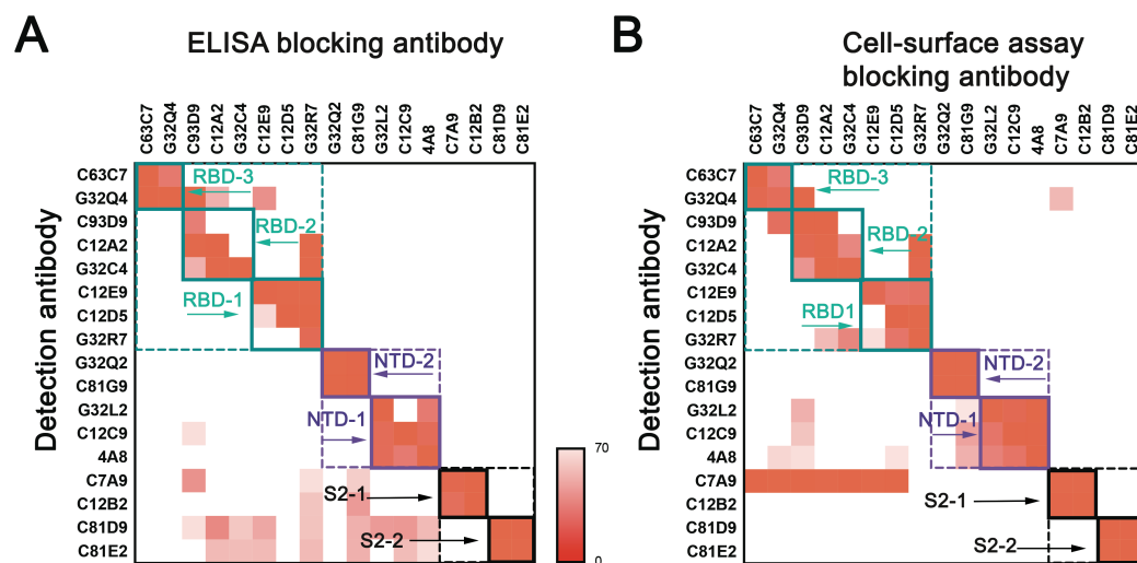
Fig. S5. Comparison of ELISA-based and cell-based competition assay. (A) Heat map of 17 mAbs with hierarchical clustering from ELISA-based cross-competition. (B) Heat map of 17 mAbs in (A) with hierarchical clustering from cell-based cross-competition. See Fig. 2B for procedures, heat-map color scheme, etc.
