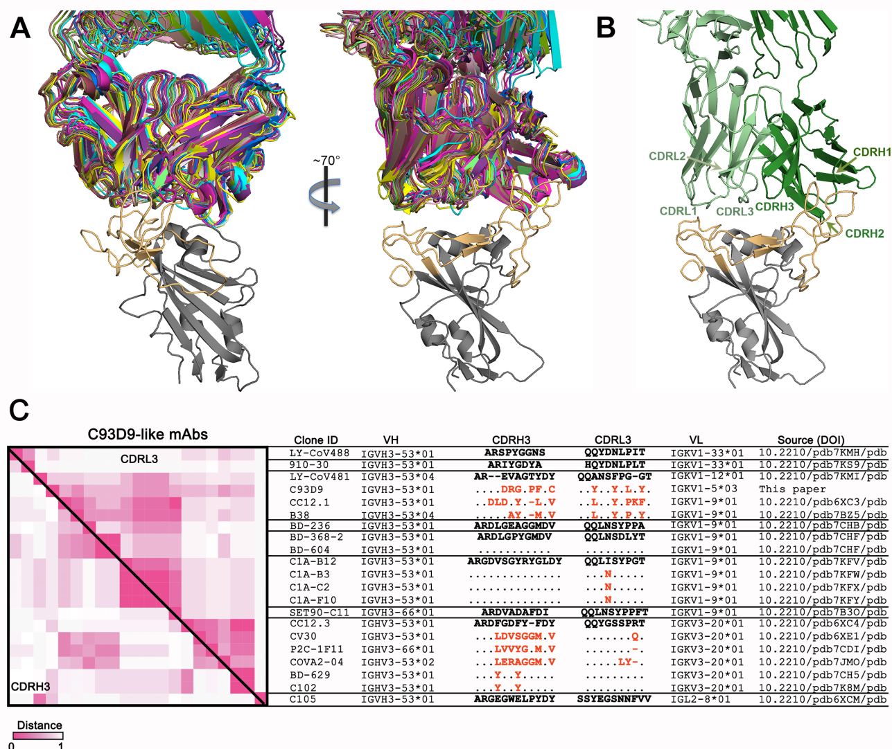
Fig. S11. The C93D9 class of antibodies. (A) Two views of 20 Fab structures, listed in (C), bound with SARS-CoV-2 RBD. Structures all superposed on the RBD; heavy-and light-chains of each Fab in a distinct color. The figure includes only the RBD from 6YZ5 (not one of the 20), with the RBM in light orange and the rest of the chain in gray. (B) View as in the right-hand panel in (A), but showing only the FAB from 7B30 (the closest in sequence to C93D9), with CDRs labeled. The most intimate contacts with RBM residues are from CDRH1, CDRH2 and CDRL1, many with residues constrained in potential variability by ACE2 interaction. (C) Maps of pairwise distances of CDRH3 (lower left triangle) and CDRL3 (upper right triangle) for the 21 C93D9 class antibodies in (A) and (B). Pairwise distances analyzed by Mega X. Intensity of color shows the distance, from 0 (identical) to 1 (no identity). The VH and VL genes encoding the antibodies are shown in the indicated groups. Differences in CDR3s from the reference sequences (bold) are in red; dashes indicate missing amino acids; dots represent identical amino acids. IGHV3-66 and IGHV3-53 are very similar VH gene segments, differing by only one encoded amino-acid residue.
