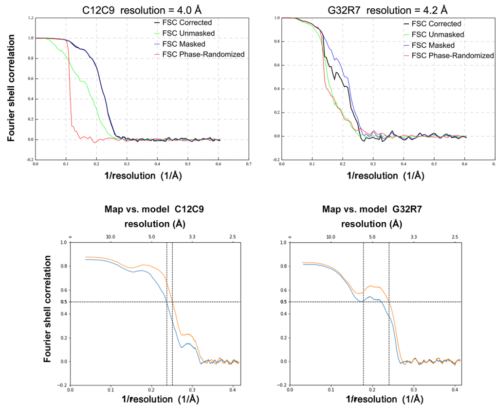
Fig. S7. Fourier shell correlation plots for the C12C9 and G32R7 complexes.
