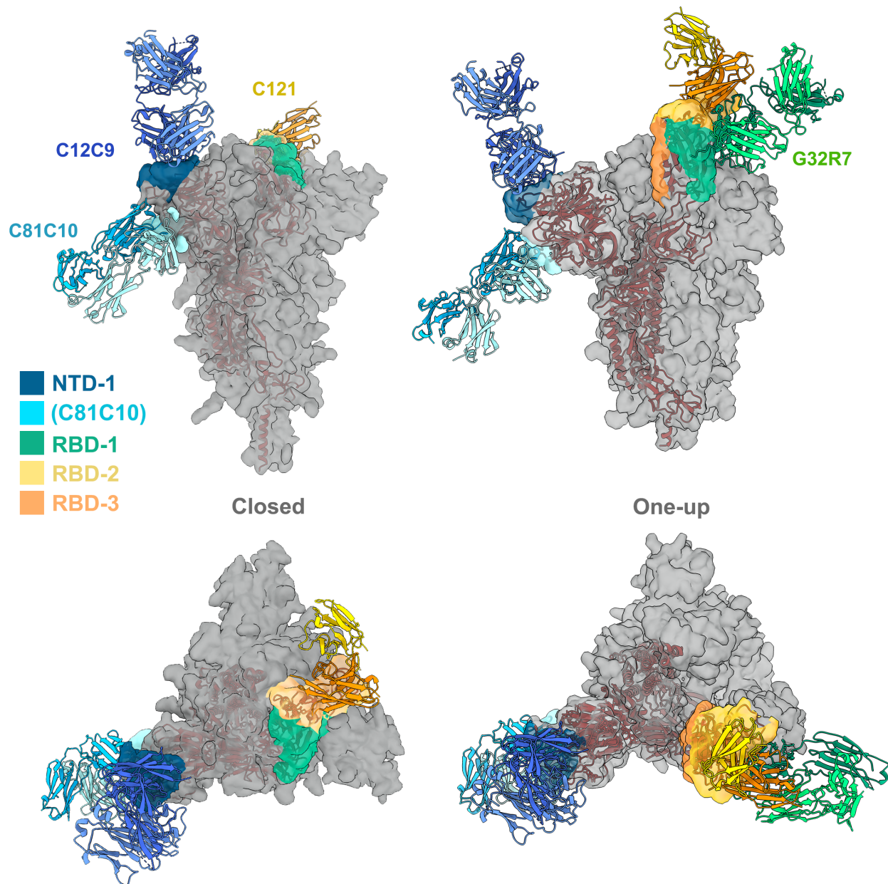
Fig. 3. Ab contact regions. Surface regions of the SARS-CoV-2 spike protein trimer contacted by antibodies in four of the seven principal clusters, according to the color scheme shown (taken from the color scheme in Fig. 2), with a representative Fab for all except RBD-3. The C81C10 Fab defines an epitope just outside the margin of NTD-1, but it does not compete with any antibodies in RBD-2. The RBD-2 Fv shown is that of C121 (PDB ID: 7K8X: Barnes et al, 2020), which fits most closely, of the many published RBD-2 antibodies, into our low-resolution map for C12A2. Left: views normal to and along threefold axis of the closed, all-RBD-down conformation; right: similar views of the one-RBD-up conformation. C121 (RBD-2) can bind both RBD down and RBD up; G32R7 (RBD-1) binds only
