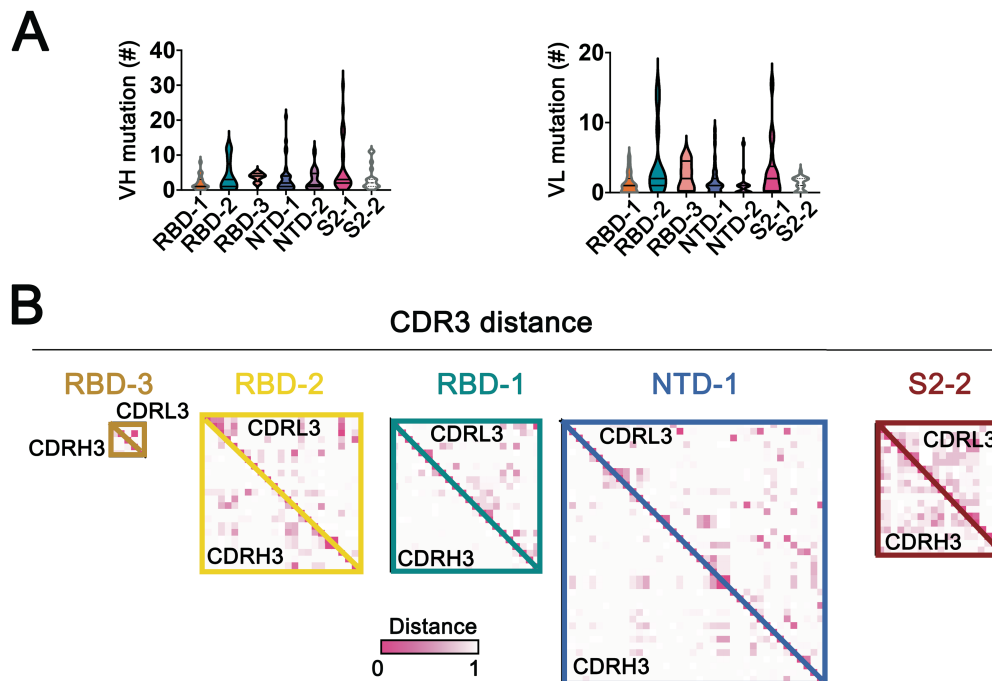
Fig. S10. Antibody sequence analyses. (A) V(D)J and VJ mutation levels in each of the 7 principal competition groups. Mutations in VH and VL (excluding CDR3) counted by IgBLAST. (B) Maps of pairwise distances of CDRH3 (lower left triangle) and CDRL3 (upper right triangle) for the RBD-1, RBD-2, RBD-3, NTD-1 and S2-2 cluster antibodies related to Fig 4B.
