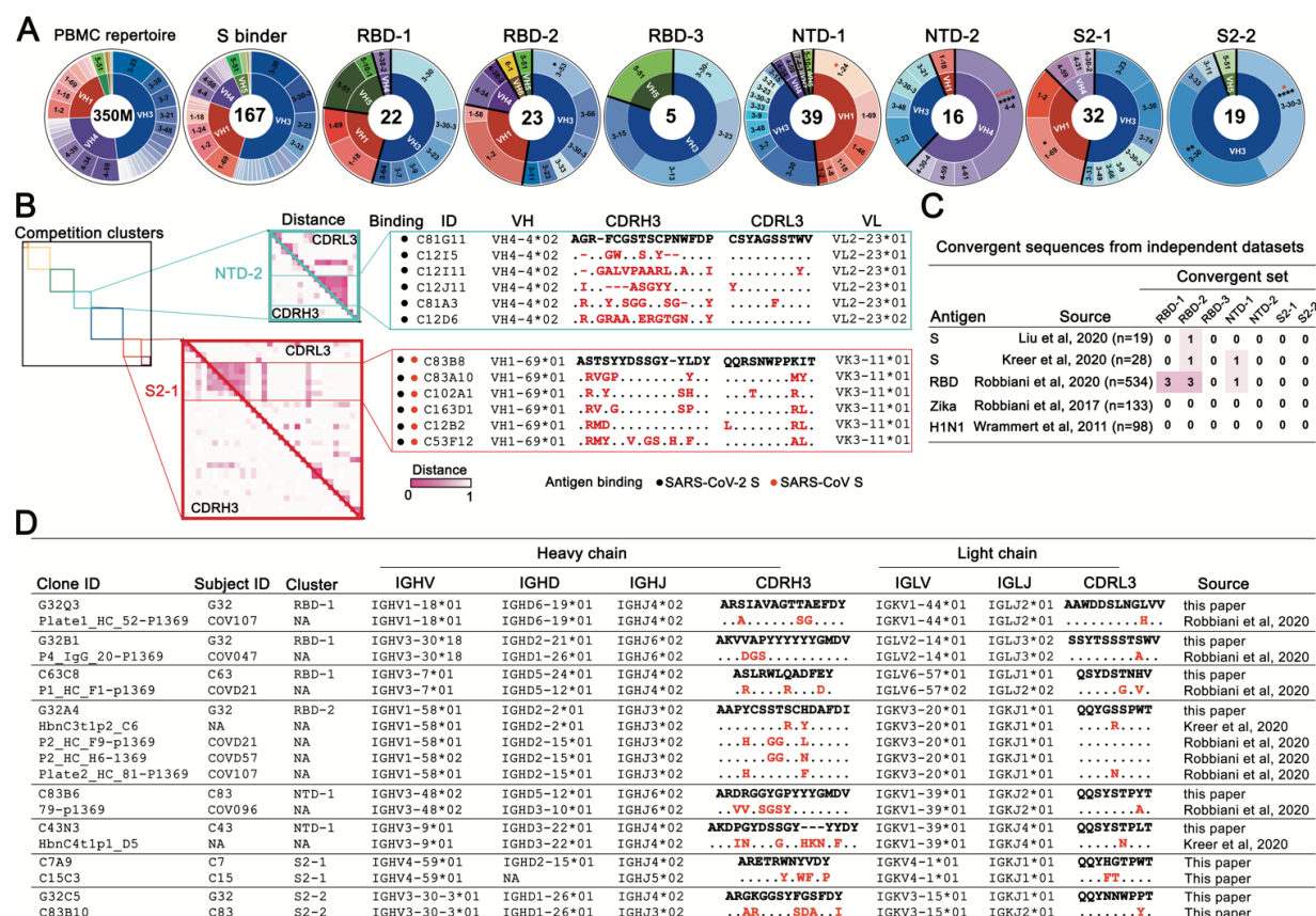
Fig. 4. Antibody sequence analyses. (A) Heavy-chain variable-domain genes of the 167 mAbs characterized by binding SARS-CoV-2 spike in either ELISA or cell-surface expression format. The inner ring of each pie chart shows the VH family and the outer ring, the gene. PBMC repertoire is from 350 million reads of deep sequencing (37). S binders include 167 clones in Table S2. * P < 0.05 , ** P < 0.01 , *** P < 0.001 , **** P < 0.0001 ; Bonferroni correction. Red asterisks: comparing to S binders; black asterisks: comparing to a non-selected B cell repertoire from PBMCs. (B) Maps of pairwise distances of CDRH3 (lower left triangle) and CDRL3 (upper right triangle) for the NTD-2 and S2-1 cluster antibodies from (A). Antibodies in both clusters arranged by VH usage. Clones converging on identical VH/VL alleles and closest distance of CDRL3 from the same cluster are shown. Pairwise distances analyzed by Mega X. Intensity of color shows the distance, from 0 (identical) to 1 (no identity). Sequence alignment for the antibodies from the indicated clusters with identical VH and VJ and similar CDR3s. Differences in CDR3s from the reference sequence (bold) are in red; dashes indicate missing amino acids; dots represent identical amino acids. (C) Summary of convergent sequences of anti-SARS-CoV-2 S and RBD antibodies from independent datasets. Ig
