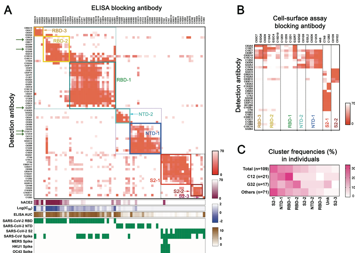
Fig. 2. Competition epitope mapping. (A) Cross competition matrix for 73 antibodies from the spike + sort in Fig. 1 with affinity sufficient for detection by ELISA. Blocking antibodies (columns) added at 100 µg/ml; detection antibodies (rows), at 1 µg/ml. Intensity of color shows strength of blocking, from 0 signal (complete blocking) to 70% full signal (top gradient at right of panel: orange). Hierarchical clustering of antibodies by cross competition into 7 groups (plus a singleton labeled S2-3), enclosed in square boxes, with designations shown and in colors from dark blue (NTD-1) to dark red (S2-3). Green arrows on the left designate antibodies newly reported here. The lower parts of the panel show: competition of blocking antibody with soluble, human ACE2 (second gradient at right: dark red); log(IC 50 ) in pseudovirus neutralization assay (third gradient at right: violet); area under the curve for ELISA binding (bottom gradient at right: brown); binding (ELISA) to recombinant domains and heterologous spike proteins. (B) Competition in cell-based assay for 36 antibodies with binding in ELISA format too weak for reliable blocking measurement (rows). Blocking antibodies (columns) selected from each of the 7 clusters in the ELISA assay (fig. S2). Strength of blocking shown as intensity of orange color, as in (A). (C) Distribution of antibodies from three individual subjects
