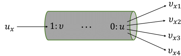
Fig 7. The template bond graph module for intermediate vessels in our version of the ADAN open-loop model. The number of v_x variables depends on the maximum number of branches occurring in any segment. Here, four auxiliary variables corresponding to four branches are demonstrated.
