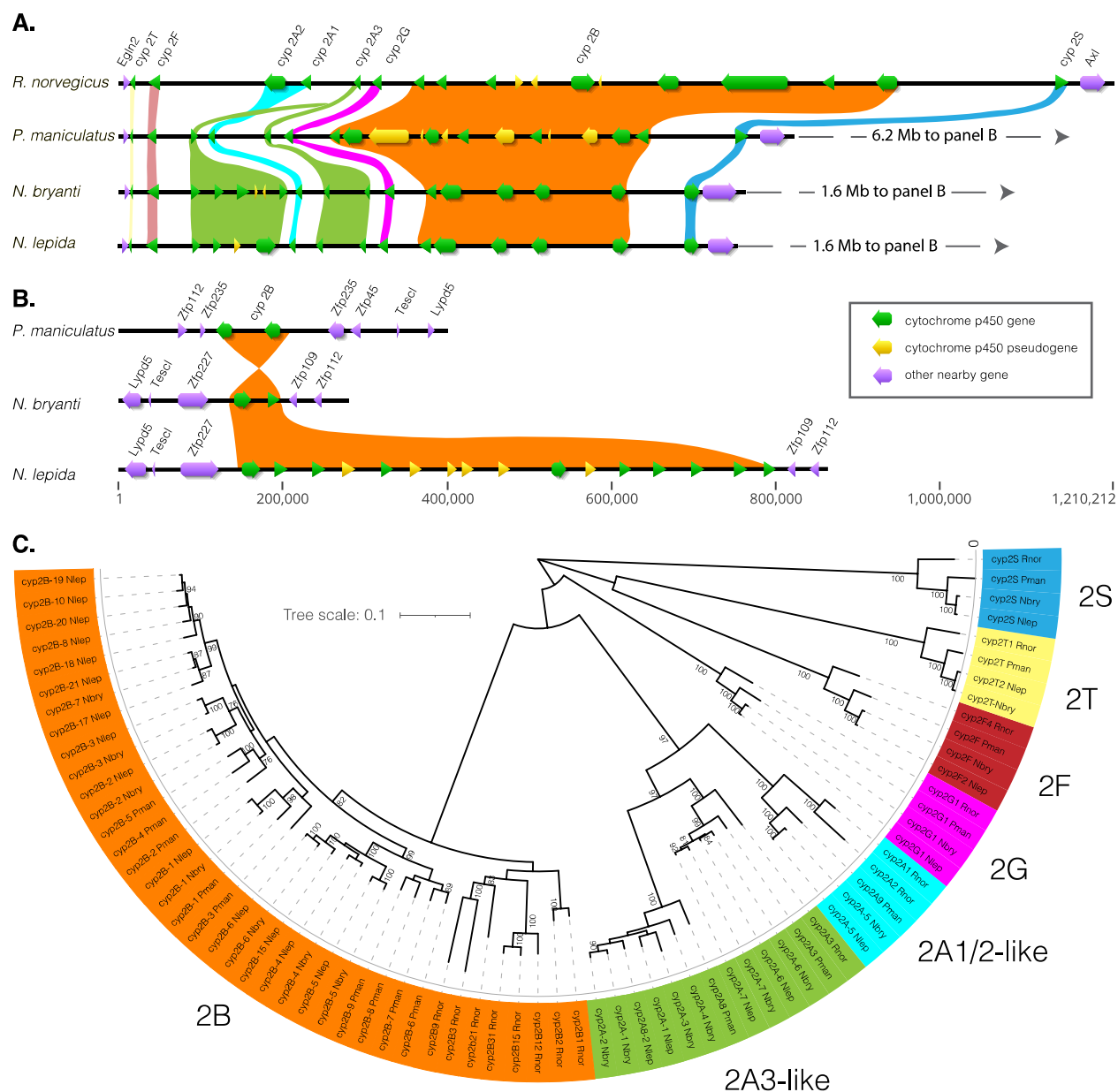
Figure 3: Genomic architecture and evolution of the cyp2ABFGST gene islands in four rodents. Visualization of the contigs containing these genes was based on annotations for the Norway rat ( Rattus norvegicus ; mRatBN7.2) and deer mouse ( Peromyscus maniculatus ; HuPman2.1), and manual annotation of these regions for Neotoma bryanti and N. lepida . (A) A highly conserved gene island is bounded by Egln2 and Axl and retains subfamily order in Neotoma and Peromyscus ; gene order is also similar to that of other vertebrates. (B) A second gene island composed of variable numbers of cyp2B genes arose in the New World rodents only, and underwent further expansion in N. lepida . (C) A tree of the inferred functional genes from each
