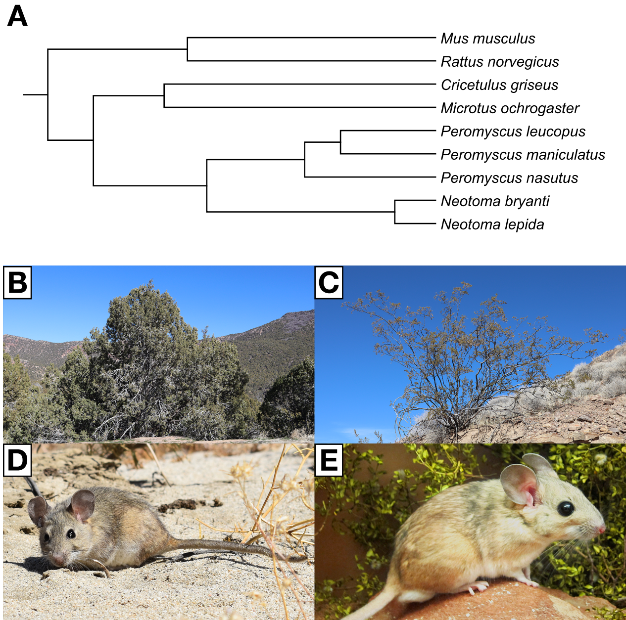
Figure 1: Phylogeny of Cricetidae rodents, common dietary items, and photographs of Neotoma bryanti and Neotoma lepida . (A) Neotoma woodrats are closely related to deer mice of the genus Peromyscus and more distantly related to other members of the family Muridae. The phylogeny for this panel was downloaded from http://www.timetree.org and visualized in MEGA X (Stecher et al. 2020). (B, C) Images of juniper ( Juniperus spp.) (B), an ancestral Neotoma food source, and creosote bush ( Larrea tridentata ) (C), the shrub that replaced it in many low elevation
