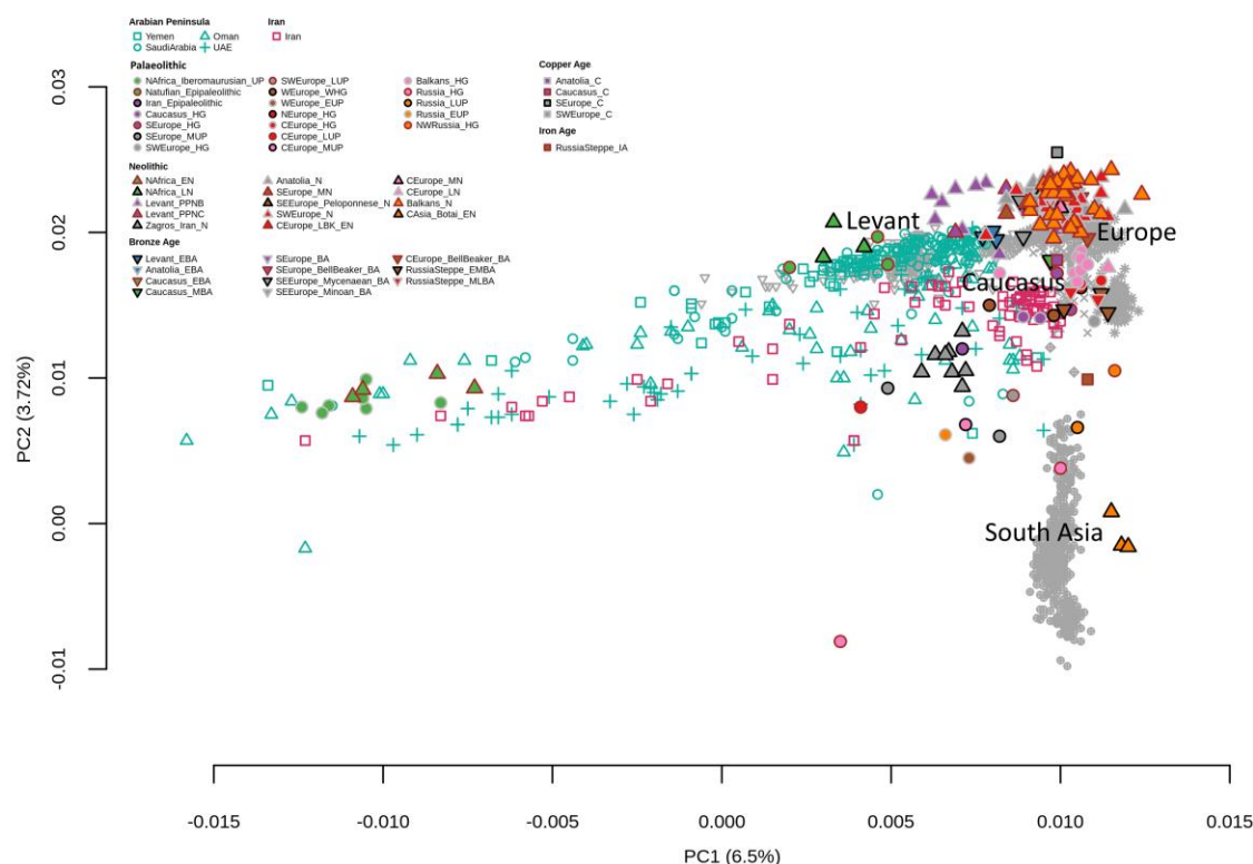
Figure 1: Principal components analysis of present-day samples from the Arabian Peninsula (blue), Iran (red) and neighbouring populations (grey, to avoid visual clutter) with projected ancient samples in different colours and formats according to the legend. Abbreviations are as follows: E, Early; M, Middle; L, Late; HG, hunter-gatherer; N, Neolithic; C, Chalcolithic; BA, Bronze Age; IA, Iron Age; UP, upper Palaeolithic.
