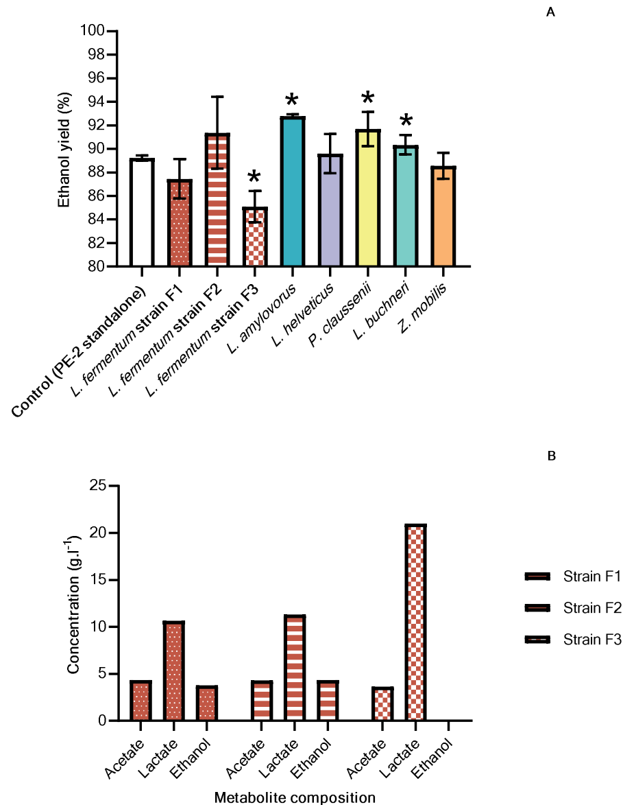
Figure 5: Specific L. fermentum strains cause reduction in bioethanol fermentation yield. A:
