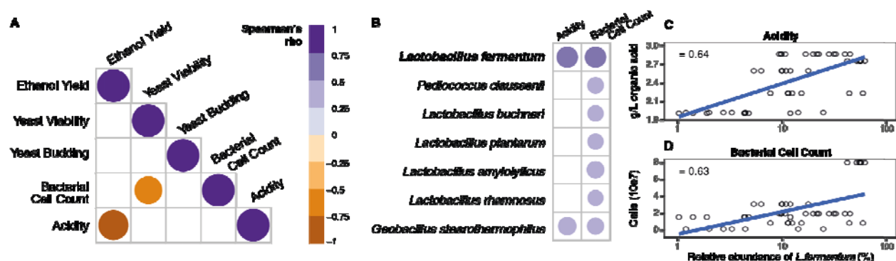
Figure 2: Microbial species and other factors that influence industrial fermentation performance. A: Fermentation parameters that showed strong associations throughout the production season. Positive correlations are depicted as purple, whereas negative correlations are depicted as orange. Size of each point denotes the strength of correlation. Increased acidity is linked with lower ethanol yield, and increased number of bacterial cells reduces yeast viability. B: Microbial species associated with fermentation performance. Increased L. fermentum during fermentation is strongly linked to higher acidity titres. Species are ordered by decreasing relative abundance. C: Correlation between relative abundance of L. fermentum and acidity ( \rho=0.64 ;
