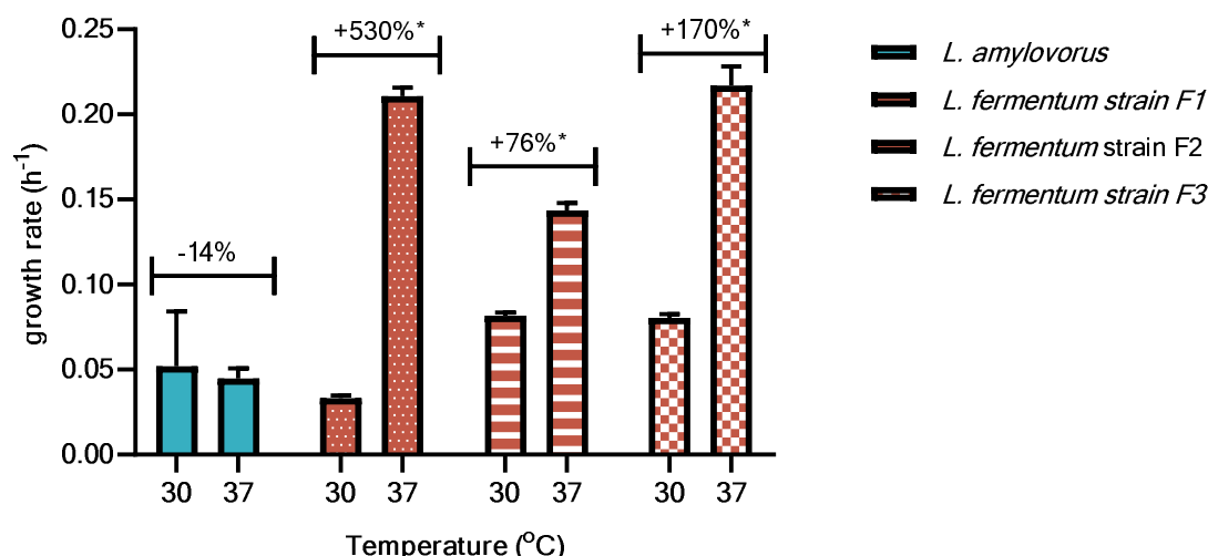
Figure 4: The influence of temperature in the growth rate ( \text{h}^{-1} ) of different industrial isolates. Higher fermentation temperatures favours L. fermentum in detriment of L. amylovorus , which has its growth rate reduced in 14% (from 0.052 \pm 0.026 to 0.045 \pm 0.005 ). Within L. fermentum , different strains display diverse responses to the increase of temperature. Strain F1 shows an average increase in its growth rate of 530% (from 0.33 \pm 0.001 to 0.211 \pm 0.004 ). Strain F2 grows 76% faster (from 0.082 \pm 0.002 to 0.143 \pm 0.004 ), and strain F3, 170% (from 0.08 \pm 0.002 to 0.217 \pm 0.009 ). * p < 0.05 .
