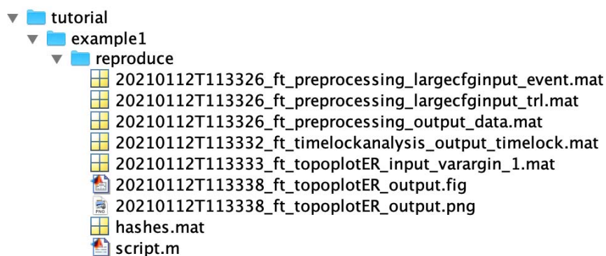
Figure 2. reproducescript creates the reproduce folder and its contents: input and output data files with unique file identifiers, a MATLAB script, and a hashes data file. See text for further explanation.
