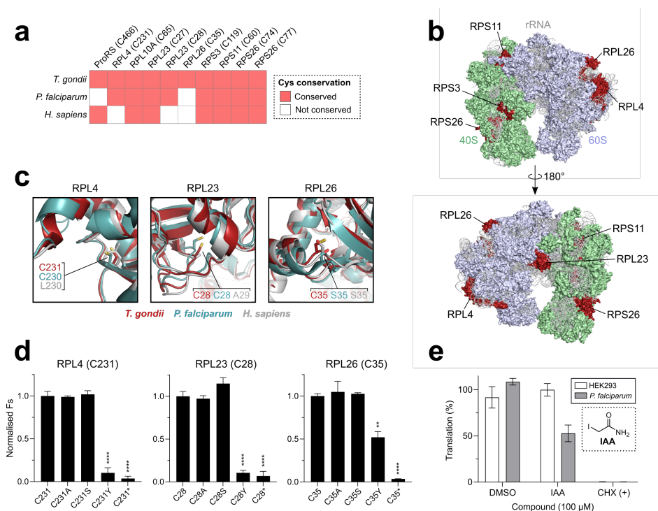
Figure 4. The apicomplexan translation machinery contains unique essential cysteines and is
