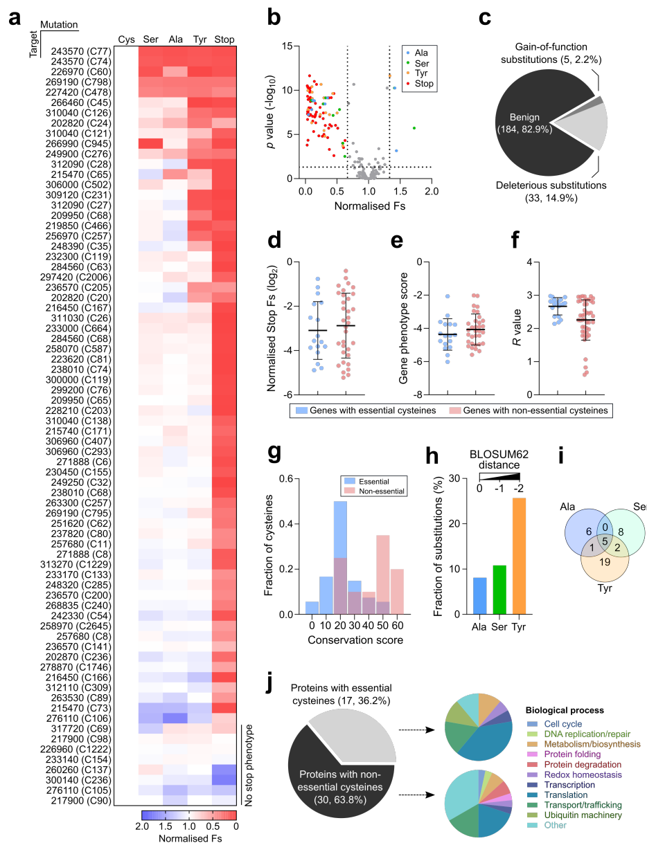
Figure 3. CORE prioritises apicomplexan protein translation as a target for covalent inhibition.
