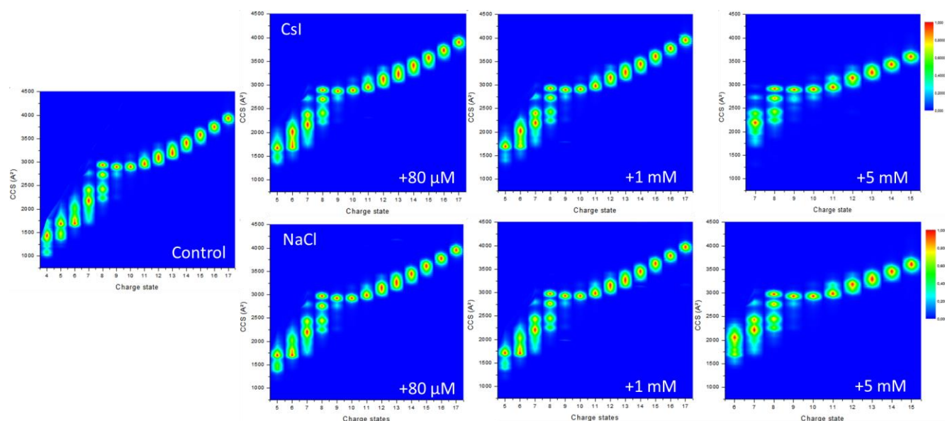
Supplementary Figure 8. aSyn is compact at lower charge states and extended at higher charge states in the absence of and with increasing concentrations of NaCl and Csl CCS plots of nano-ESI-IM-MS spectra of aSyn at all charge states detected. aSyn in 20 mM ammonium acetate with no salts (Control) and in the presence of 80 μM, 1 mM or 5 mM Csl and NaCl. Higher CCS values show more extended structures and extended structures are favoured at higher charge states. Shown are representative CCS plots from three injections of aSyn.
