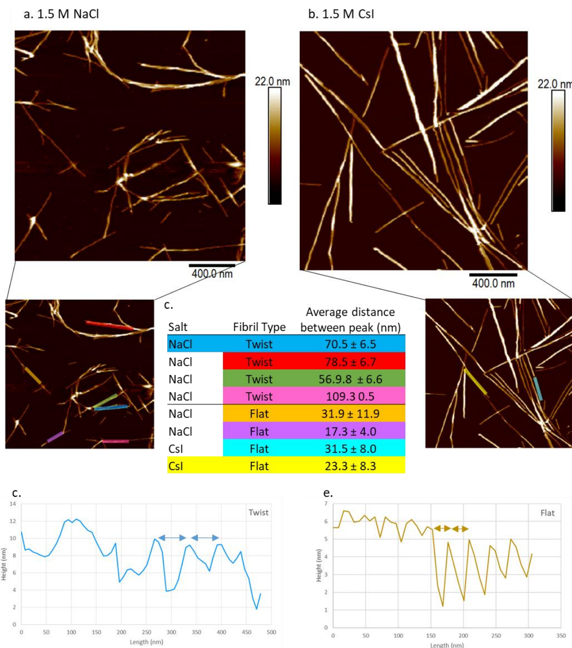
Supplementary Figure 2. Identification of flat and twisted aSyn fibril polymorphs by AFM aSyn fibrils formed during ThT-based assays were imaged on freshly cleaved mica and representative images are shown for different fibril polymorphs, 'twisted' containing a helical pitch and 'flat' with no visible helical pitch in (A.) 1.5 M NaCl in D 2 O and (B.) flat only 1.5 M CsI in D 2 O. Insets with coloured lines correspond to the colours in the table and show regions where fibril height was analysed. (C.) Table listing salt conditions, fibril type and distance measured between fibril peaks. Distances between peaks were calculated based on height profiles determined in the Nanoscope analysis software and are represented in (D.) for twisted fibrils with peak distances between 57-109 nm and (E.) flat fibrils with peak distances between 17 – 32 nm. The colours of the graph of peak heights in (D. + E.) correspond to the top blue twisted fibril and the bottom yellow flat fibril highlighted in table C and in the inserts of A and B.
