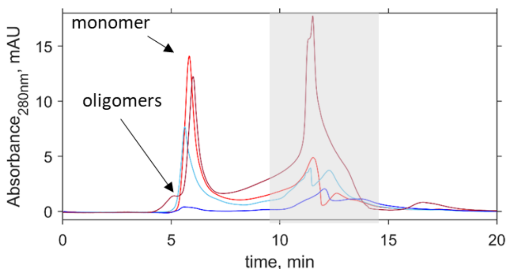
Supplementary Figure 3. Representative analytical size exclusion chromatograph of remaining aSyn monomer after ThT-based assays The content of each well after ThT-based assays was centrifuged and the remaining monomer analysed by analytical SEC-HPLC on an AdvanceBio 130Å column at a flow rate of 1 mL/min in 20 mM Tris pH 7.2 and monitored by absorbance at 280 nm. The area under the curve of the monomeric aSyn, which eluted ~ 5.2 minutes, was used to calculate the remaining monomer from known concentrations of aSyn. Representative chromatographs for aSyn in 150 mM NaCl (light blue), 1.5 M NaCl (dark blue), 150 mM CsI (red), 1.5 M CsI (dark red) are shown. Oligomeric species eluted before the monomer and can be detected in the 1.5 M CsI trace (dark red). Elution time for aSyn shifts slightly dependent on the salt and concentration present. The presence of salt is also detected in the grey region.
