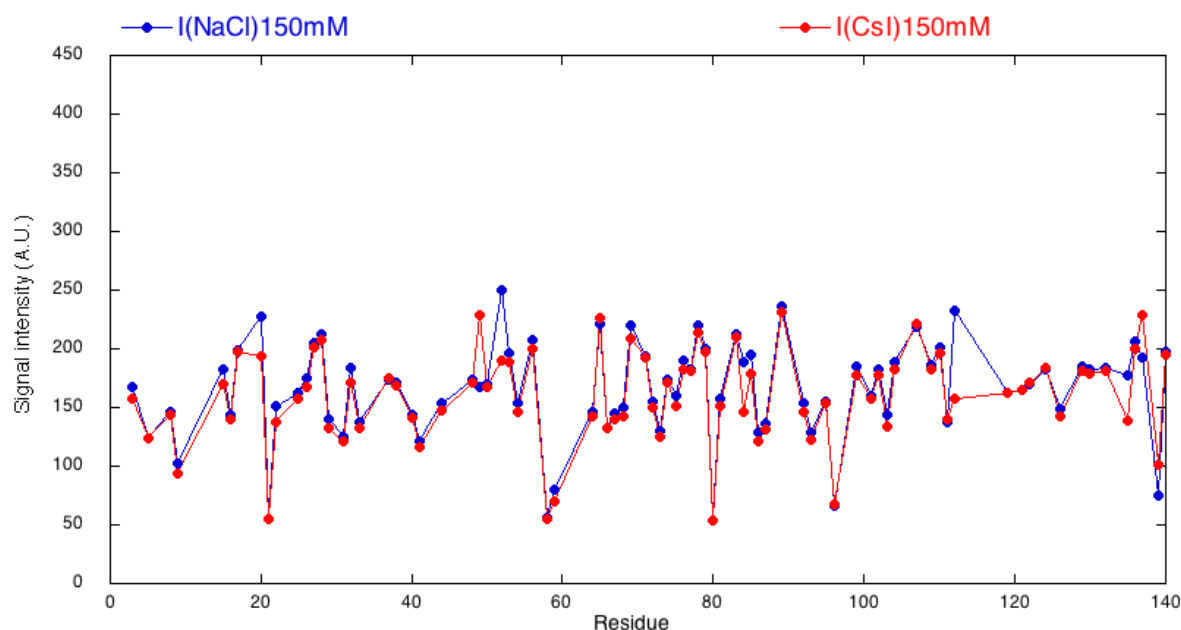
Supplementary Figure 9. Intensity signal of ^1\text{H} and ^{15}\text{N} -labelled aSyn in 150 mM NaCl is slightly higher than in 150 mM CsI HSQC NMR spectroscopy was used to measure the intensity of 150 \mu\text{M} ^1\text{H} and ^{15}\text{N} -labelled aSyn in 95% \text{H}_2\text{O} , 5% \text{D}_2\text{O} (vol/vol) in 150 mM CsI and NaCl. Each residue covered is represented by a spot. The signal intensity of aSyn in 150 mM NaCl is similar, but marginally high than in CsI, indicating less mobility in NaCl.
