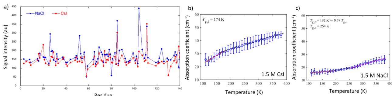
Figure 4. NMR and THz-TDS show that aSyn is more mobile in CsI compared to NaCl.
