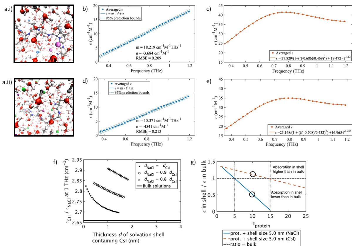
Figure 2. Addition of NaCl and CsI alter water mobility in the bulk and in the aSyn solvation shell. A snapshot of the AIMD simulations of the solvated aSyn 72-78 peptide in a 125 nm 3 box after introduction and equilibration with 1.5 M salts. (a.i) aSyn 72-78 peptide in 1.5 M CsI and (a.ii) aSyn 72-78 peptide in 1.5 M NaCl, Cs + light purple, I - light blue, Na + dark purple, Cl - green, O red, H white, C grey, N dark blue. The molar absorption coefficient measured with THz-TDS for (b) NaCl solutions, (c) CsI solutions, (d) solutions of NaCl and aSyn, and (e) solutions of CsI and aSyn. (b) and (d) are fitted with a linear function and (c) and (e) with the sum of a power law and a Lorentzian to account for the spectral shape. (f) At 1 THz the solvation shell surrounding aSyn containing CsI ( \epsilon_{\text{CsI}} ) absorbs more than the shell containing NaCl ( \epsilon_{\text{NaCl}} ) and both solvation shells absorb more compared to bulk only (black line at 2.66). The dependency of absorption on the salt is plotted for several possible sizes d of the solvation shell, allowing a smaller shell size d_{\text{NaCl}} in solutions containing NaCl. The same trend is apparent for all shell sizes. (g) Absorption in the solvation shell excluding the protein itself is compared to bulk absorption at 1 THz. Representative ratio of the absorption in the shell compared to bulk absorption for NaCl (blue line) and CsI (orange, dotted) for varying protein absorption ( \epsilon_{\text{p}} ) between 1-25 cm -1 M -1 . The solvation shell with NaCl absorbs less than the bulk (denoted by the black dashed horizontal line) above \epsilon_{\text{p}} = 5 cm -1 M -1 (denoted by the black vertical dotted line at 5 cm -1 M -1 ), while the solvation shell with CsI absorbs less than the bulk above \epsilon_{\text{p}} = 15 cm -1 M -1 (denoted by the black dotted vertical line 15 cm -1 M -1 ) at an ion shell size of 5 nm. At \epsilon_{\text{p}} = 10 cm -1 M -1 , an intermediate protein absorption coefficient,
