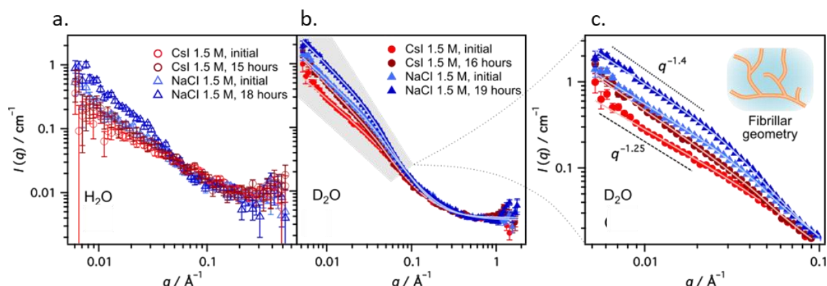
Supplementary Figure 4. Model fits to the SANS data using the Guinier-Porod model. SANS data for solutions of 434 \mu\text{M} aSyn in either 1.5 M NaCl or Csl in \text{H}_2\text{O} (a) and \text{D}_2\text{O} (b). The aSyn in \text{H}_2\text{O} samples had high scattering, therefore the model was fit to \text{D}_2\text{O} data only. In c, solid symbols indicate experimental scattering data and solid lines represent the model fits. (g) Zoomed-in view of the low q region in b (shaded area) highlighting the differences in scattering intensity for each sample. Characteristic slopes are indicated with the data ( q^{-1.25} and q^{-1.4} ), and the inset has been added to signify the fibrillar-type structure as determined by the modelling. Fitting values are shown in Supplementary Table 1.
