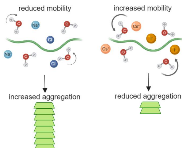
Figure 5. Aggregation kinetics of aSyn are dependent on water mobility which is strongly affected by the presence of ions. Presence of Na + (light blue) and Cl - (dark blue) lead to reduced mobility of water (H 2 O) and aSyn monomers (green protein), allowing the formation of stable intermolecular bonds between two adjacent monomers which can lead to aggregation into aSyn amyloid fibrils (stacked green protein). Presence of Cs + (light orange) and I - (dark orange) lead to increased mobility of water and aSyn monomer, which decreases the likelihood of two monomers being stable enough to permit intermolecular interactions and thus results in reduced aggregation.
