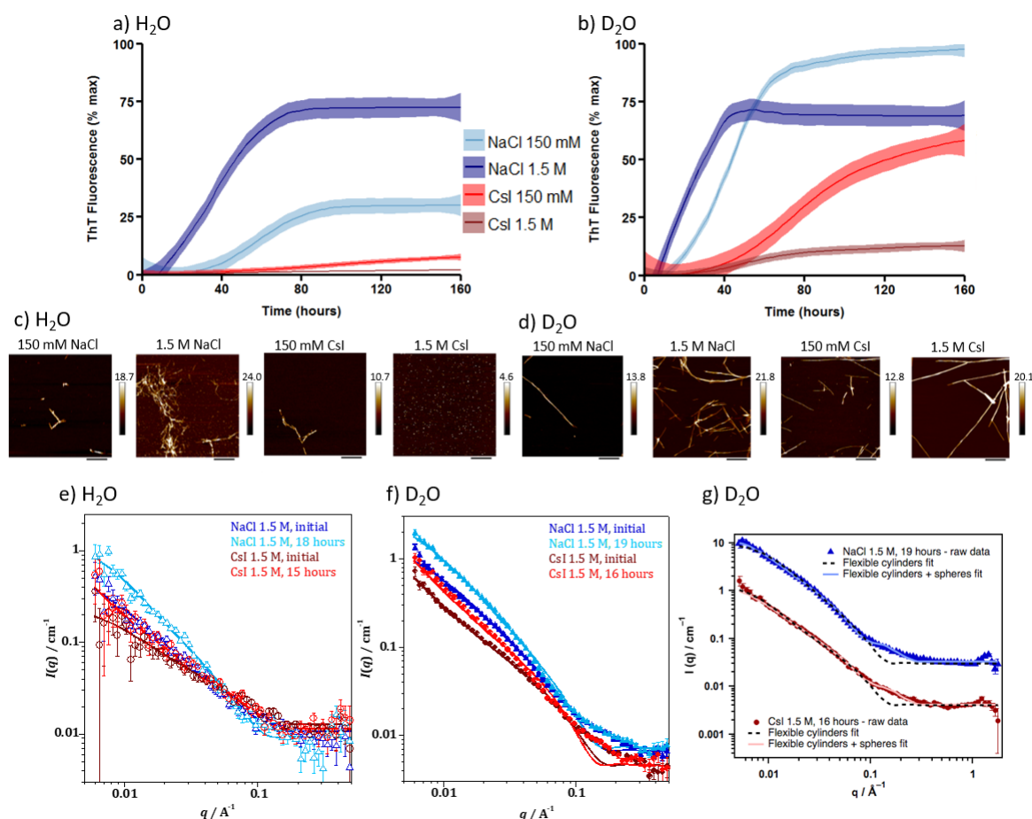
Figure 1. NaCl and CsI concentrations influence aSyn aggregation rate and morphology.
