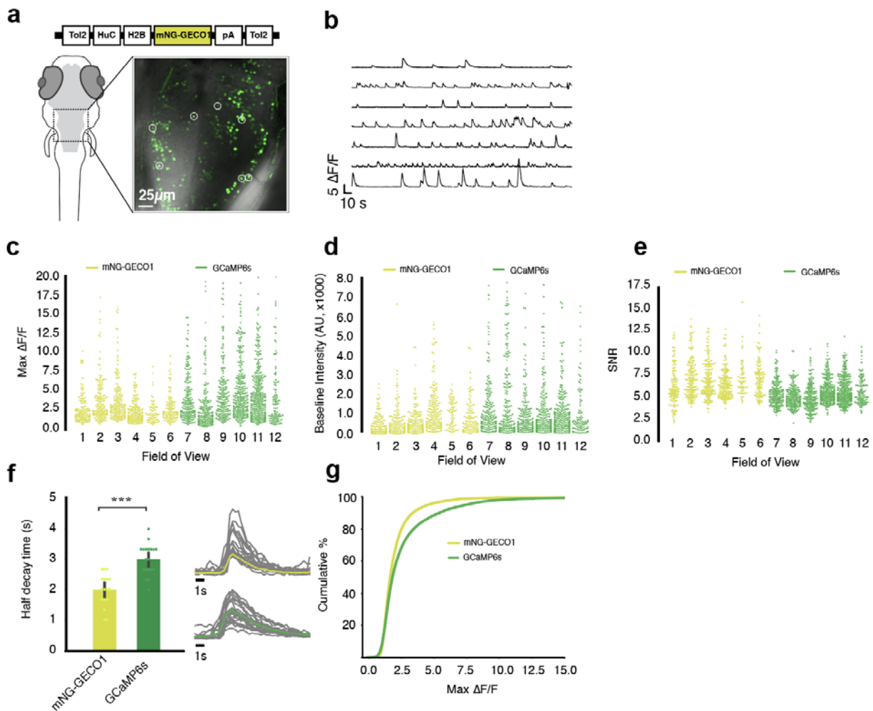
Figure 3 Characterization of mNG-GECO1 and GCaMP6s in transgenic zebrafish hind brain tissue. a Schematic representation of Tol2[HuC-H2B-mNG-GECO1] construct and confocal image of one fish (5 to 6 days post fertilization) with 7 region of interests (ROI) circled. b Traces of ROI's from a). c Max \Delta F/F_0 calculated by taking the max peak of each cell within the field of interest over 5 minutes; six ROI's each are used from 5 independent fish expressing mNG-GECO1 and 5 fish expressing GCaMP6s. d Baseline fluorescence intensity of each cell within all ROI's from 5 fish; confocal settings are kept consistent between GCaMP6s and mNG-GECO1 imaging. e Signal-to-noise ratio (SNR) computed by dividing \Delta F/F_0 by raw standard deviation of each cell across 6 FOV's each for both sensors. f Average half decay time plotted for mNG-GECO1 (n = 17) and GCaMP6s (n = 19) by averaging randomly selected peaks. g
