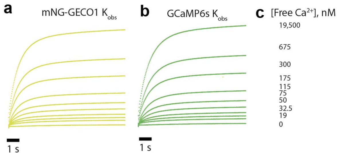
Supplementary Figure 3 K_{on} , (observed) traces of mNG-GECO1 and GCaMP6s purified protein using Photophysics SX-20 Stopped-flow. Each protein buffered in 30 mM MOPS, 100 mM KCl, 50 \mu M EGTA is rapidly mixed at 1:1 ratio with varying concentrations of Ca^{2+} produced by reciprocal dilutions of 10 mM EGTA and 10 mM CaEGTA. a mNG-GECO1 change in fluorescence over time as Ca^{2+} is rapidly mixed. b GCaMP6s change in fluorescence over time as Ca^{2+} is rapidly mixed. c Final free- Ca^{2+} concentrations produced after reciprocal dilutions. mNG-GECO1 and GCaMP6s fit with a double exponential curve due to a slow rate limiting step likely caused by the conformational change of the proteins upon binding to Ca^{2+} . Both sensors have a similar t_{1/2} for physiologically relevant Ca^{2+} concentrations.
