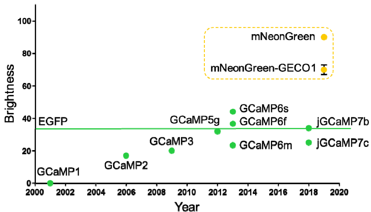
Supplementary Figure 4 In vitro brightness comparison of mNG-GECO1 to GCaMP series 1P purified protein brightness of first generation mNG-GECO1 compared to the GCaMP series of \text{Ca}^{2+} indicators. mNG-GECO1 is substantially brighter in vitro than the highly-engineered GCaMP series, which is roughly as bright as its own scaffold, EGFP.
