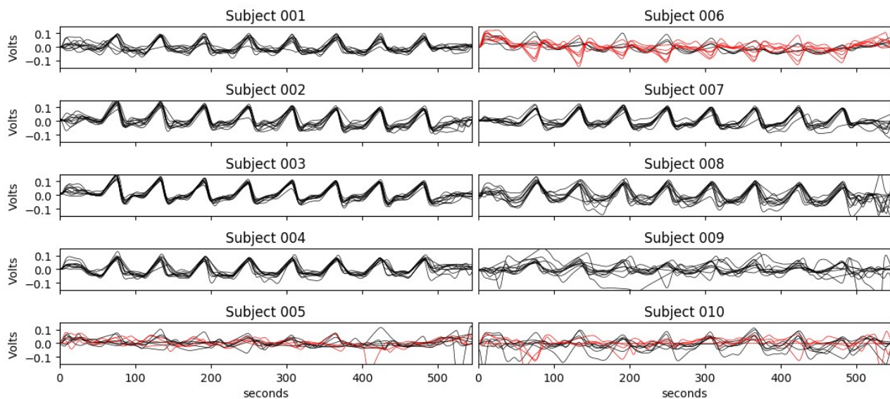
Figure 2: P_{ET}CO_2hrf trace for all subjects and all sessions. Rejected sessions are plotted in red. Rejection was based on having less than three proper P_{ET}CO_2 increases after breathholds or having more P_{ET}CO_2 decreases than increases after breathholds. Note that the first session of subject 10 was lost due to a software malfunction during acquisition.
