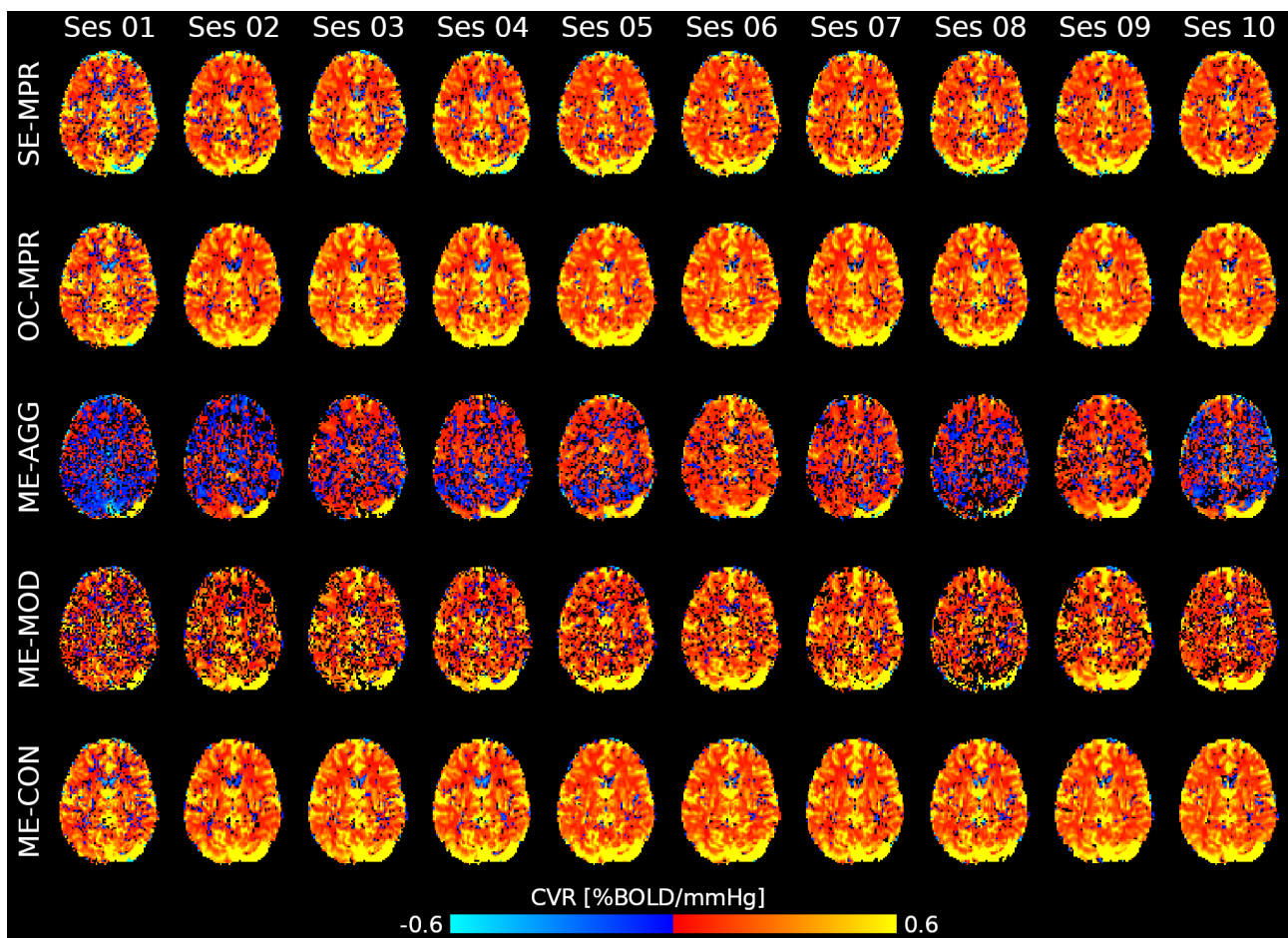
Figure 5: Thresholded CVR map obtained with the different lagged-GLM analysis for all the sessions of a representative subject (subject 002). Note the low CVR response in ME-AGG, depicting numerous voxels with a negative values, as well as the increased amount of masked voxels in SE-MPR, ME-AGG and ME-MOD. SE-MPR: single-echo; OC-MPR: optimally combined; ME-AGG: aggressive; ME-MOD: moderate; ME-CON: conservative. The CVR maps of other subjects are available in the supplementary materials.
