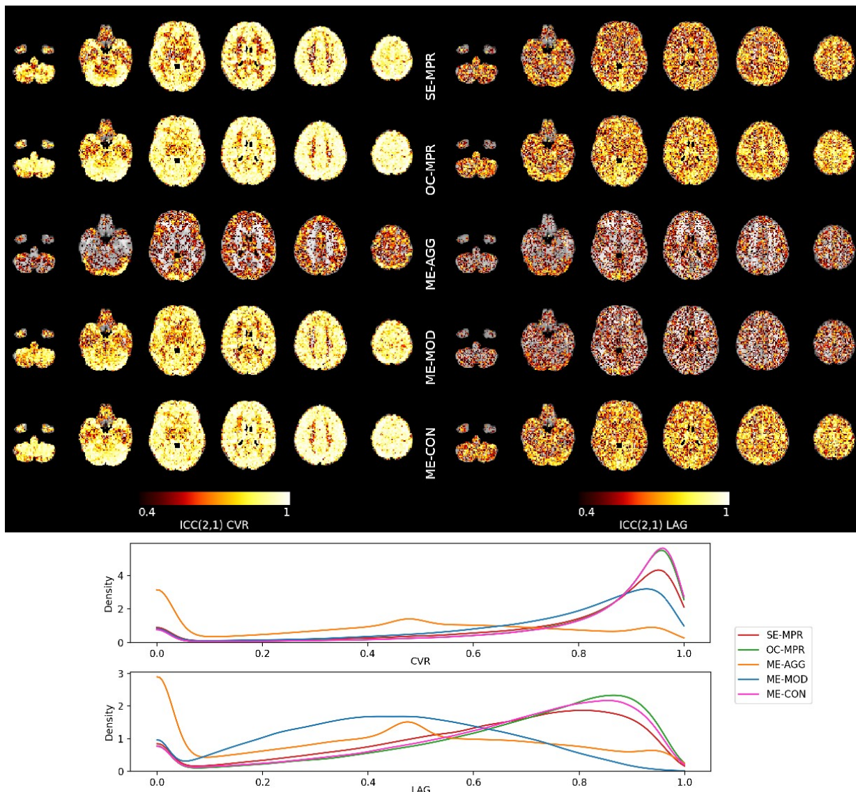
Figure 9: ICC(2,1) maps of CVR (left) and haemodynamic lag (right) for each analysis pipeline. The maps are thresholded at 0.4 since scores lower than it indicate poor reliability. A high ICC score indicates that the inter-subject variability is higher than the intra-session variability, while a low ICC score suggest that the variability across sessions is the same as the one across subjects. Following the classification given by Cicchetti (2001), an ICC score lower than 0.4 is considered poor, lower than 0.6 fair, lower than 0.75 good, and equal or higher than 0.75 excellent. The bottom rows depict the whole brain distribution of ICC scores across voxels. Note how OC-MPR and ME-CON have generally higher ICC scores than the other approaches, and are very similar to each other, while ME-AGG has the lowest ICC scores for both CVR and lag maps. SE-MPR: single-echo; OC-MPR: optimally combined; ME-AGG: aggressive; ME-MOD: moderate; ME-CON: conservative. The distribution of ICC scores across GM voxels only is available in the Supplementary Material (Supplementary figure 6).
