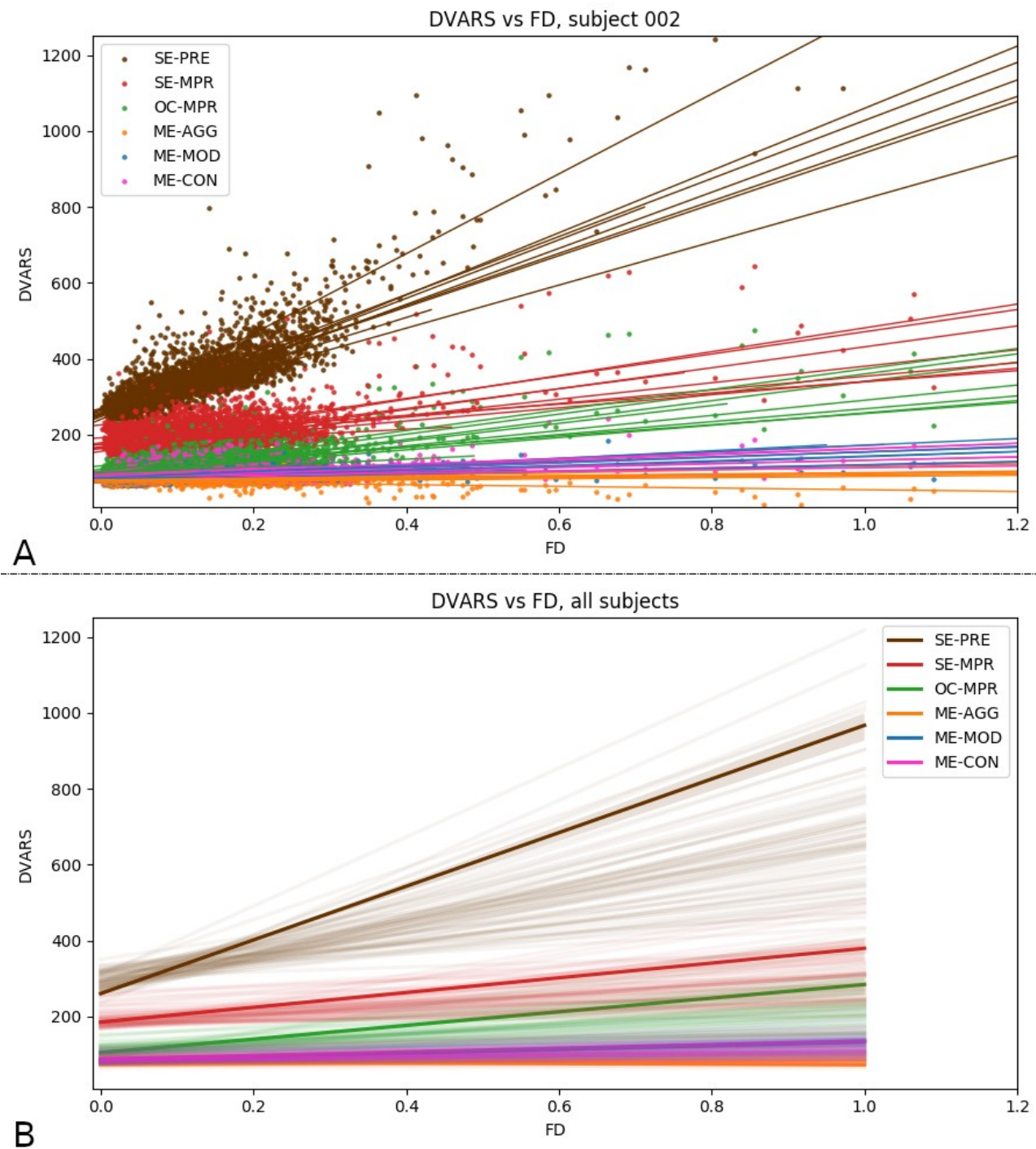
Figure 3: (A) Relation between the DVARS of the denoised data following different analysis pipelines and FD for a representative subject. Each point represents a timepoint, each line the linear regression between both timeseries in a session. In general, OC-MPR shows lower DVARS than SE-MPR, but similar modulation of the DVARS-FD relationship. All the ICA denoising solutions performs better in reducing motion-related effects described by FD on DVARS. Between the ICA solutions, ME-AGG performs the best in reducing this relationship, while ME-MOD and ME-CON seem to be equivalent. (B) DVARS vs. FD for all the subjects. Each transparent line represents a session, the solid line represents the estimation across subjects and sessions. Similar patterns to the representative subject are shown. SE-PRE: raw data; SE-MPR: single-echo; OC-MPR: optimally combined; ME-AGG: aggressive; ME-MOD: moderate; ME-CON: conservative. The relation between DVARS and FD of the other subjects can be found in the Supplementary Material (Supplementary figure 2).
