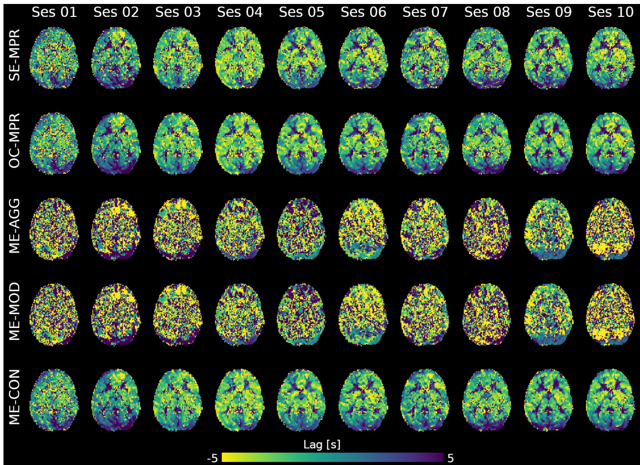
Figure 6: Unthresholded lag map obtained with the different lagged-GLM analysis, for all the sessions of a representative subject (same as figure 5). These lag maps represent the delay between the best shifted version of the P_{ET}CO_2hrf trace and the bulk shift (i.e. the best match between average grey matter signal and P_{ET}CO_2hrf trace). The scale from -5 to +5 represents earlier to later hemodynamic responses. Note the lack of anatomically informative patterns in ME-MOD and ME-AGG. SE-MPR: single-echo; OC-MPR: optimally combined; ME-AGG: aggressive; ME-MOD: moderate; ME-CON: conservative. The lag maps of other subjects are available in the supplementary materials.
