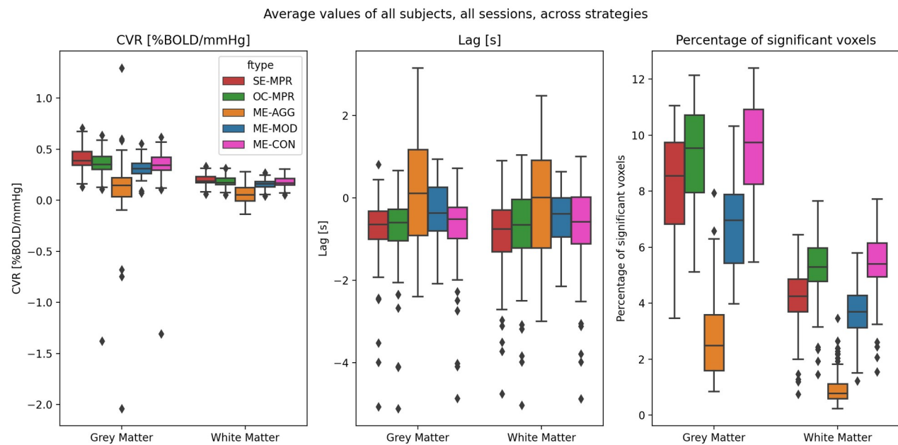
Figure 7: Average values of CVR, lag, and percentage of significant voxels, for voxels in the grey and white matter tissues separately, for all denoising strategies. The dots correspond to a singular session of a singular subject considered an outlier in the distribution. Note that all maps were thresholded before plotting. SE-MPR: single-echo; OC-MPR: optimally combined; ME-AGG: aggressive; ME-MOD: moderate; ME-CON: conservative.
