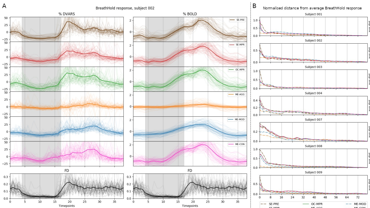
Figure 4: (A) Average GM %DVARS and %BOLD response of all BH trials across ten sessions for the same representative subject. The apnoea period is highlighted in grey. Each transparent line is a trial, the solid line is the average across all the trials. (B) Manhattan distance between the average of N trials and the average of all 80 BH trials as N increases from 1 to 80 for each subject. Each vertical line divides the number of trials in each session. SE-PRE: raw data; SE-MPR: single-echo; OC-MPR: optimally combined; ME-AGG: aggressive; ME-MOD: moderate; ME-CON: conservative. The average %DVARS and %BOLD response of the other subjects can be found in the Supplementary Material (Supplementary figure 2)
